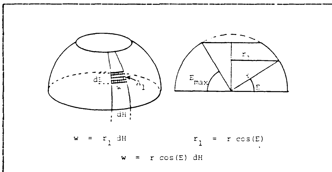
Figure C.1 Hemispherical Geometry.
