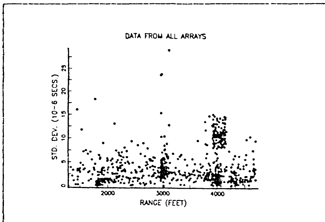
Figure 6.1 Error Estimation Versus Range of Target.
