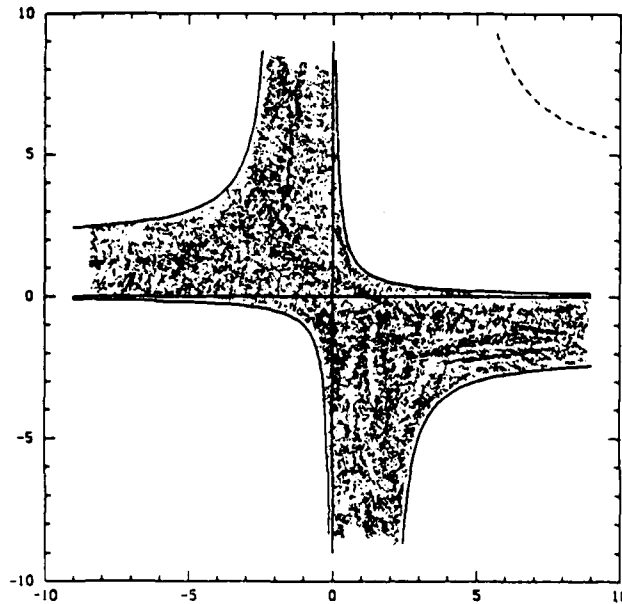
Figure 7: Stability regions for the ILU factorization.
