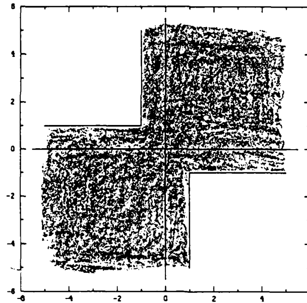
Figure 8: Stability regions for the MILU factorization.
