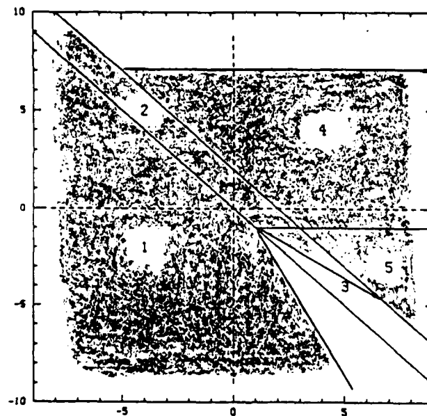
Figure 11: Values of x and y where inequality (6.3) holds.
