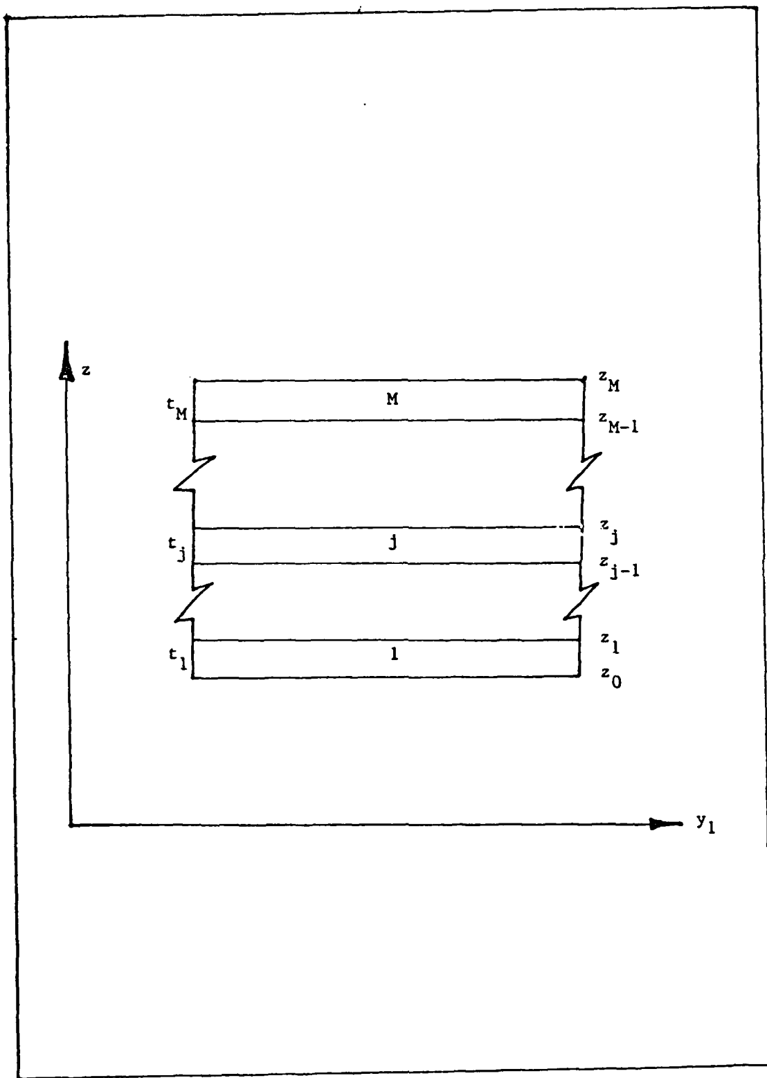
Fig. 2 Typical Lamina Lay-up
