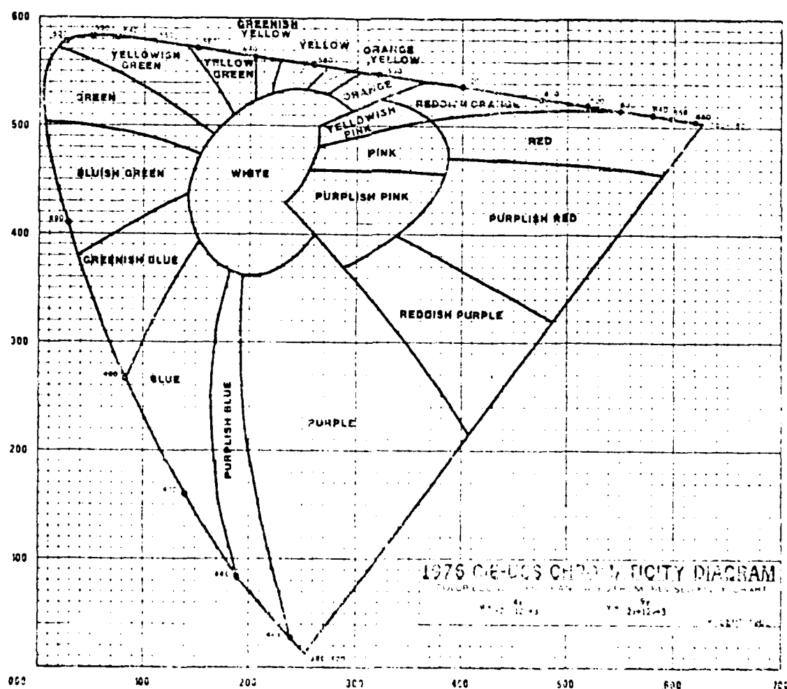
Figure 2. Color Chart for 1976 CIE-UCS Chromaticity Diagram
