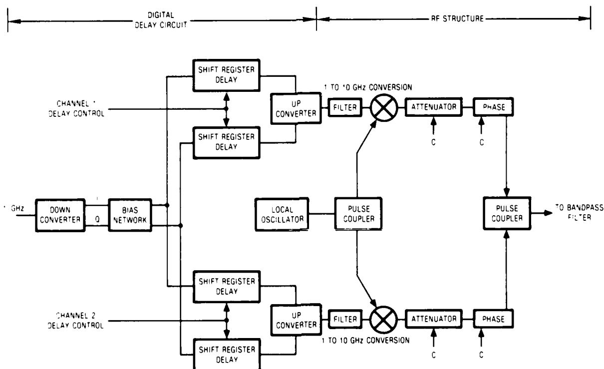
Figure 21. One-Channel Cancellor
