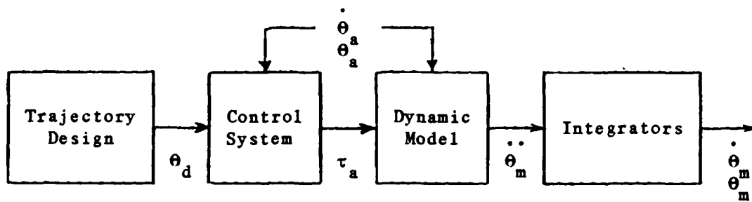
Figure 1. Manipulator Model Block Diagram
