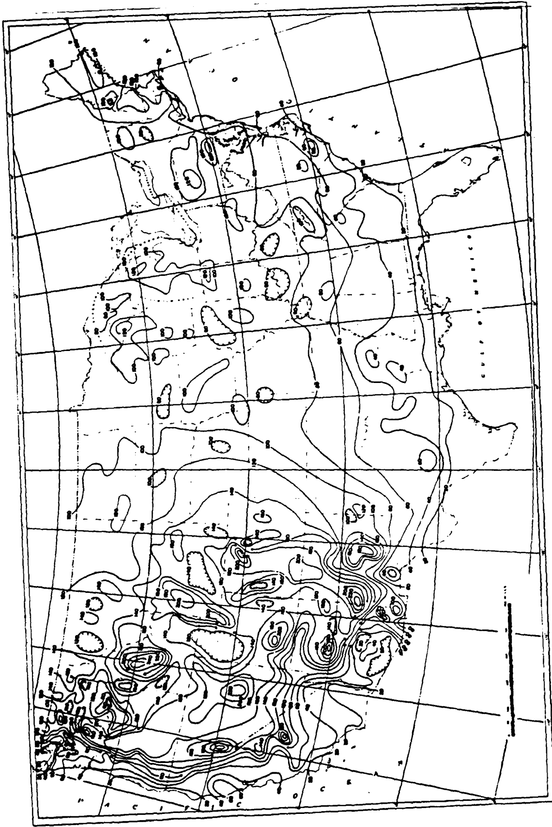
Figure 13. Mean annual frequency (days) of freeze-thaw cycles (Hershfield, 1974).
