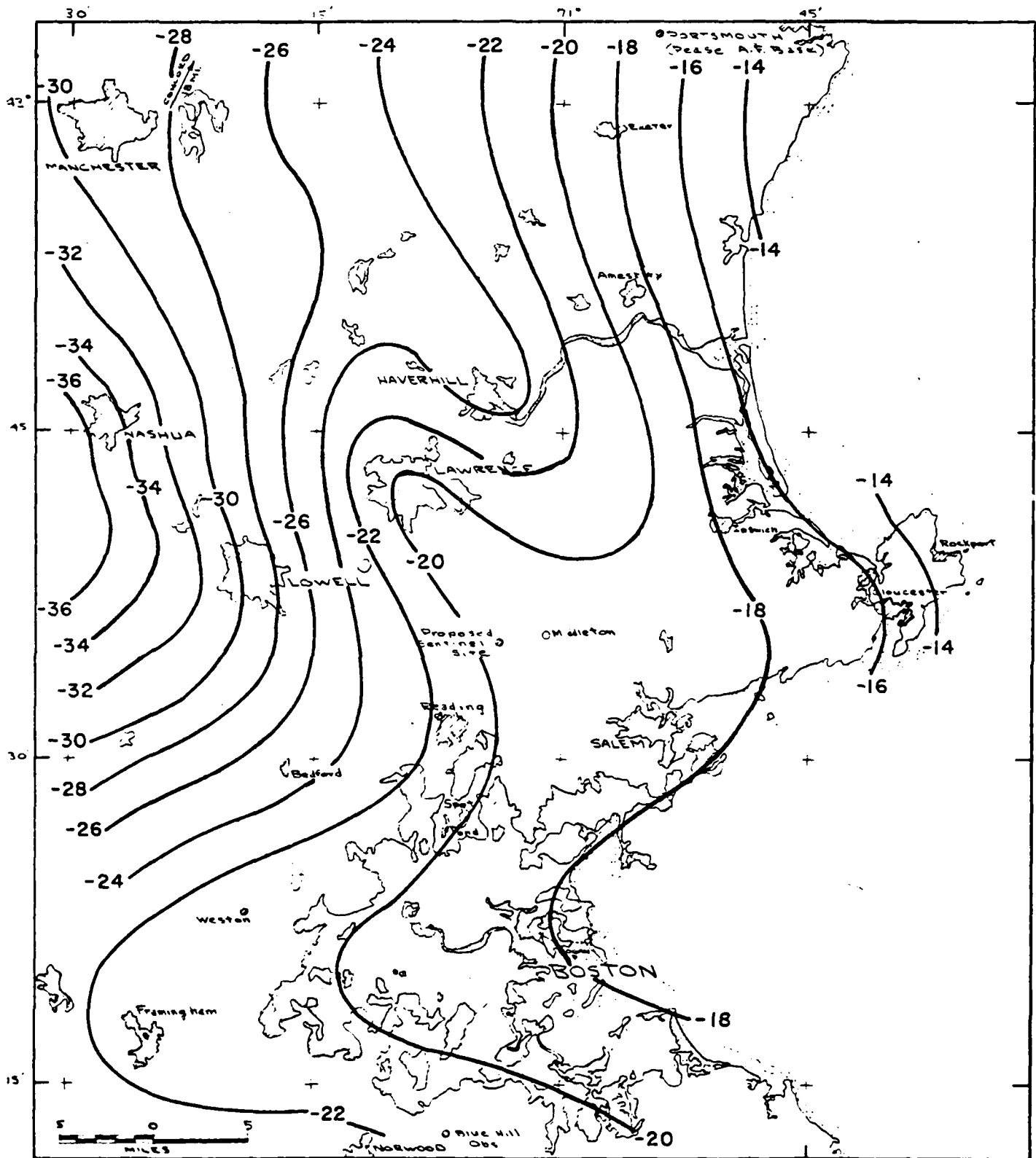
Figure 5. Extreme observed minimum air temperatures ( ^{\circ} F) for southeastern New Hampshire and northeastern Massachusetts (Bilello, 1968).
