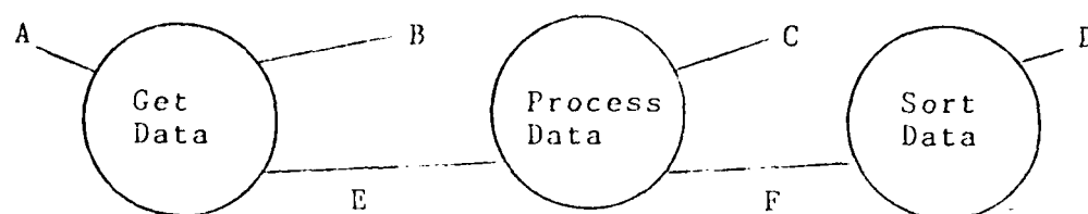
Bubble_IO Relation
