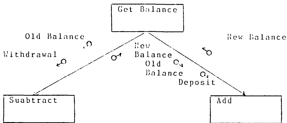
Pr_Passed Relation
