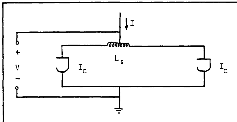
Figure II-3. Circuit Diagram of a DC-SQUID (7:79).
