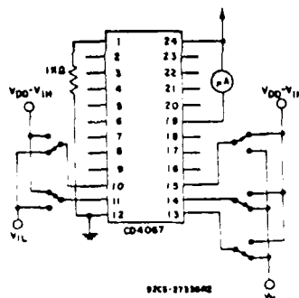
Fig. 8—Input voltage—measure < 2\text{ }\mu\text{A} on all OFF channels (e.g., channel 12).
