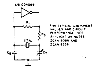
Fig. 19 - Typical crystal oscillator circuit.
