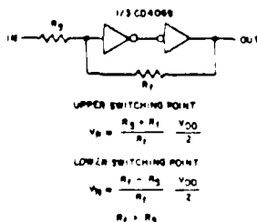
Fig. 22 - Input pulse shaping circuit (Schmitt trigger)
