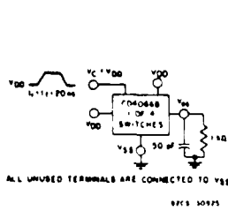
Fig. 14 - Propagation delay t_{PLH} , t_{PHL} control-signal output. Delay is measured at V_{Oj} level of +10% from ground (turn-on) or on-state output level (turn-off).
