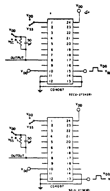
Fig. 12—Turn-on and turn-off propagation delay—inhibit input to signal output (e.g. measured on channel 1).
