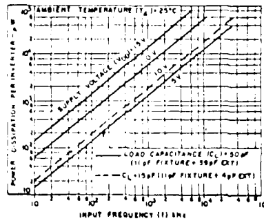
Fig. 13 - Typical dynamic power dissipation vs. frequency.
