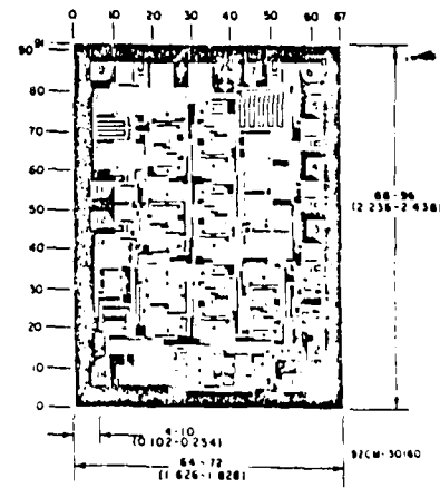
Dimensions and Pad Layout for CD4024BH.
