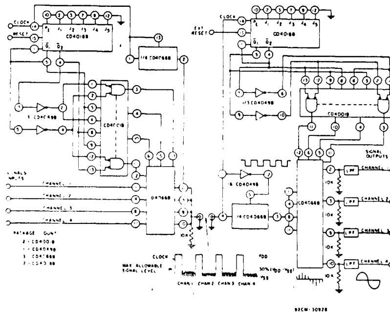
Fig. 17 - 4-channel PAM multiplex system diagram.
