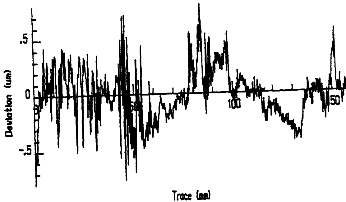
b. Surface profile after test
