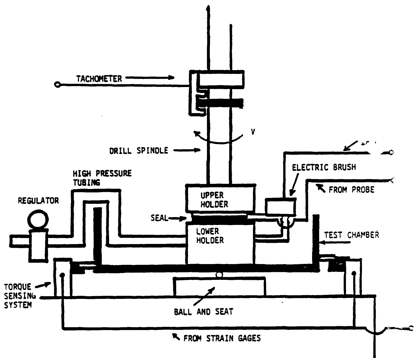
FIGURE 1. SCHEMATIC DIAGRAM OF TEST APPARATUS
