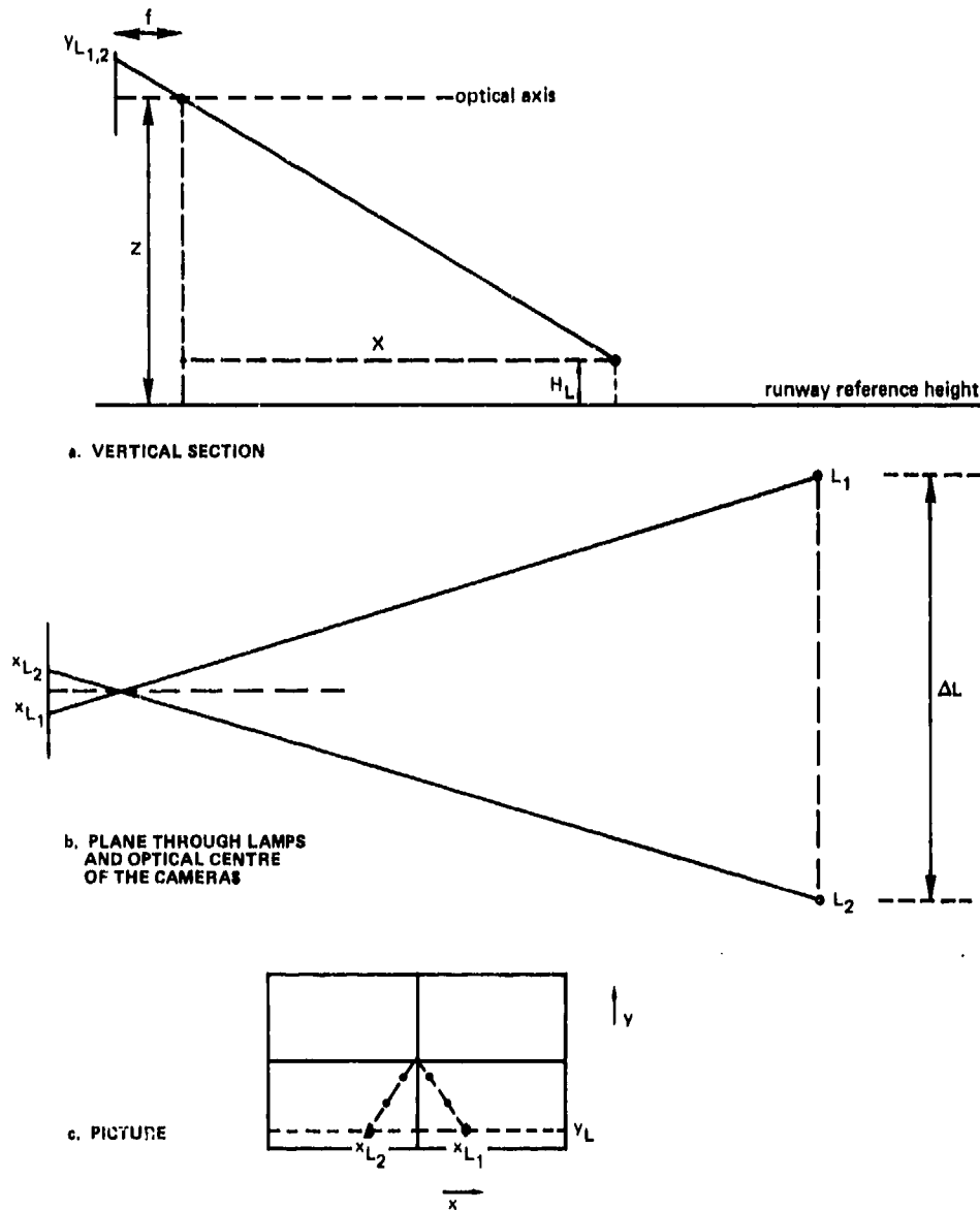
Fig. 18 Optical schematics and film picture of a nose camera if \theta , \phi , \psi and Y are zero
