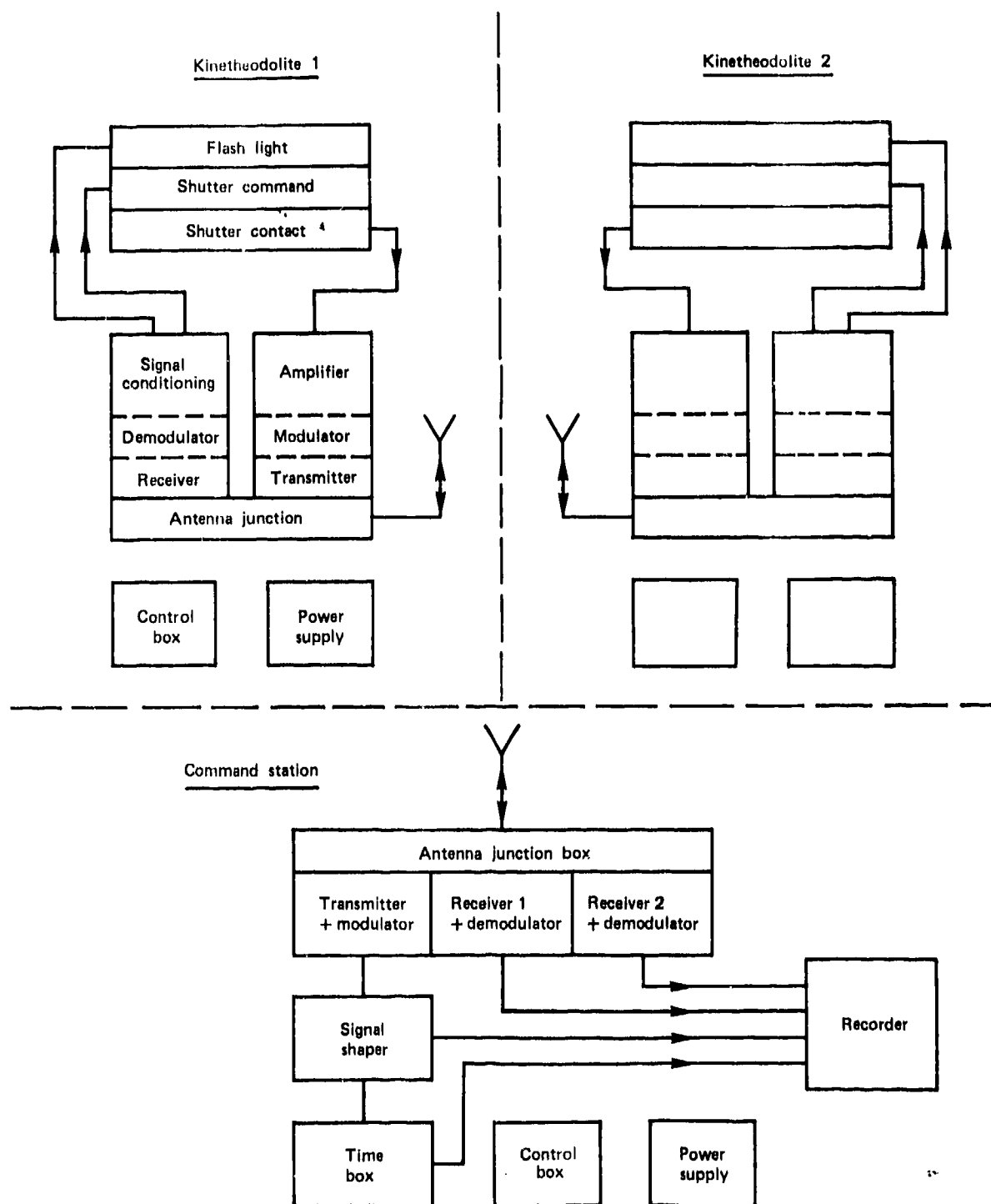
Fig. 12 Block diagram of a setup with two kinetheodolites connected to the command station by radio
