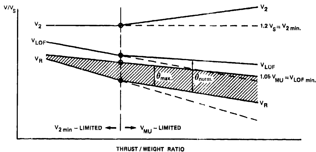
Fig. 2 Relations between several speed values for a take-off schedule
