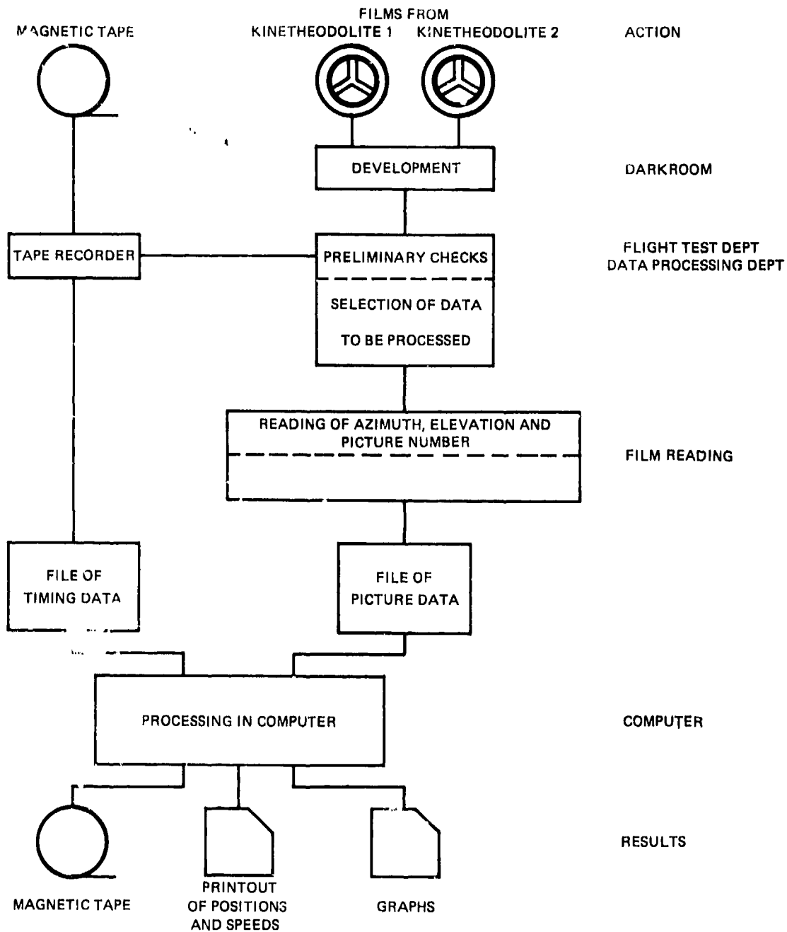
Fig. 14 Block diagram of kinetheodolite processing
