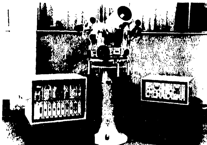
Fig. 9 An Askania kinetheodolite with (right) its control unit and (left) the command station
