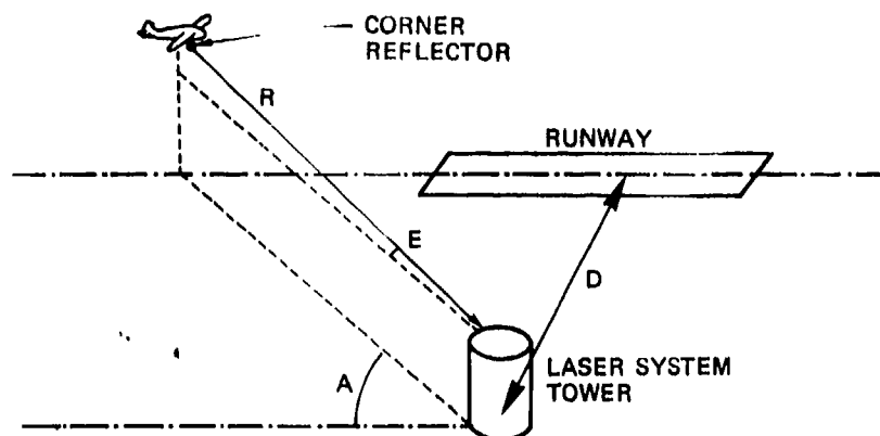
Fig. 24 Basic setup of a trajectory measurement system using a laser
