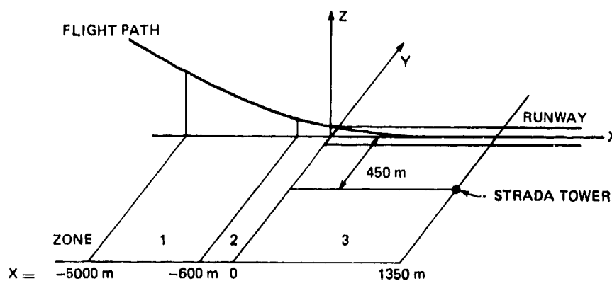
Fig. 30 Definition of axes and zones for trajectory measurements with laser
