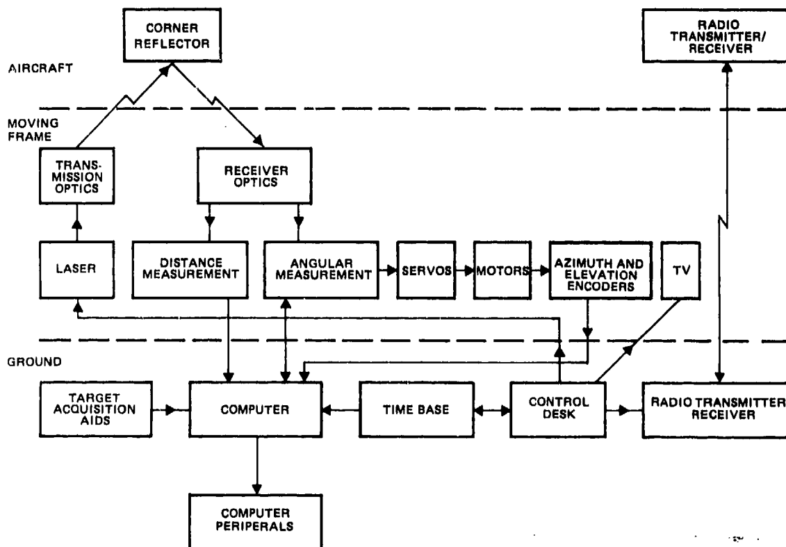
Fig. 25 Block diagram of a trajectory measuring system using a laser
