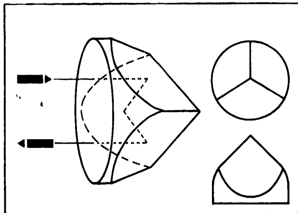
Fig. 26 Principle of a corner reflector
