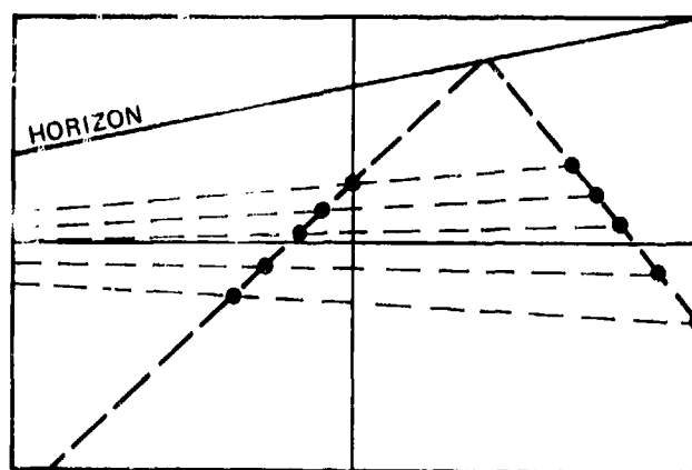
Fig. 21 Nose camera picture for the case that both \phi and \psi are 10 degrees
