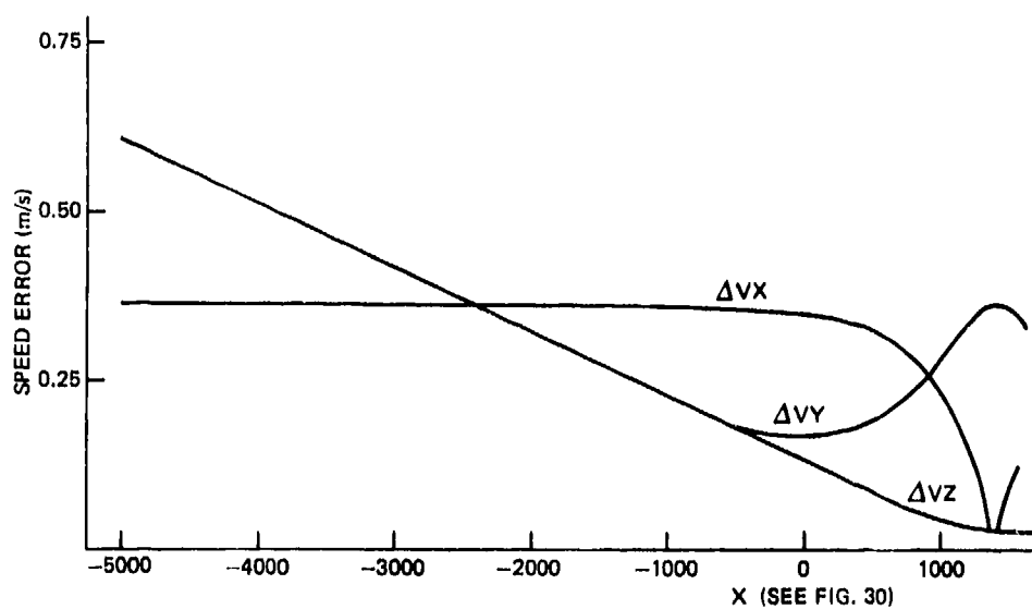
Fig. 29 Typical overall speed errors of a laser tracker
