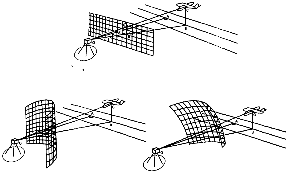
Fig. 15 Cameras photographing through a plane, a cylindrical and spherical grid
