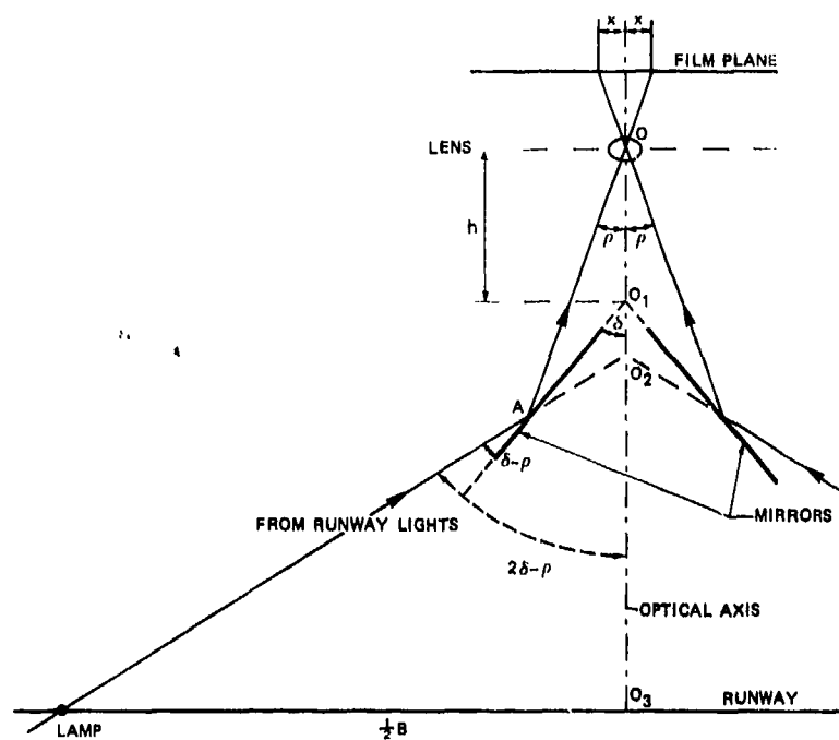
Fig. 22 Principle of the side-looking on-board camera
