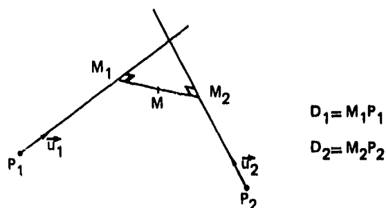
Fig. 8 Definition of parameter in Eq. 3.2.5
