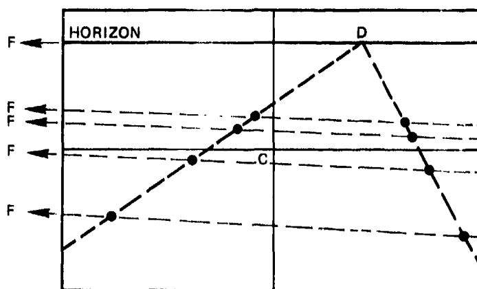
Fig. 20 Nose camera picture for the case that \phi = 0 and \psi = 10 degrees
