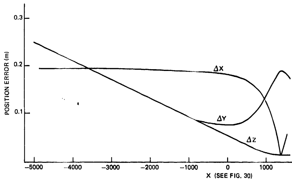
Fig. 28 Typical position errors of a laser tracker
