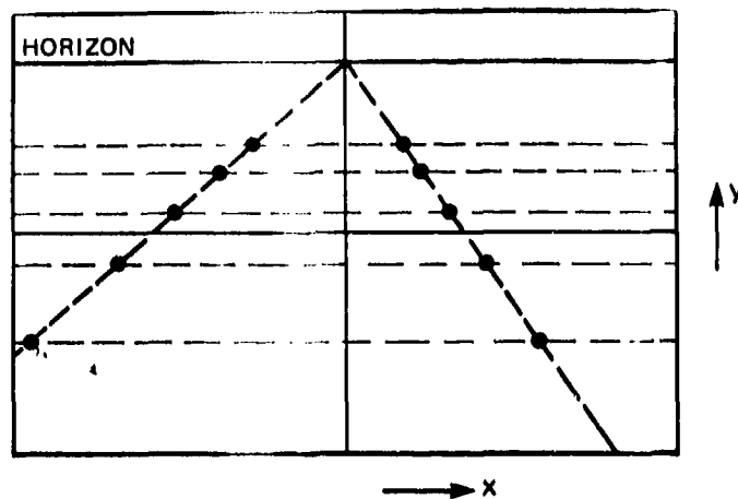
Fig. 19 Nose camera picture for the case that \phi and \psi are zero, Y is non-zero
