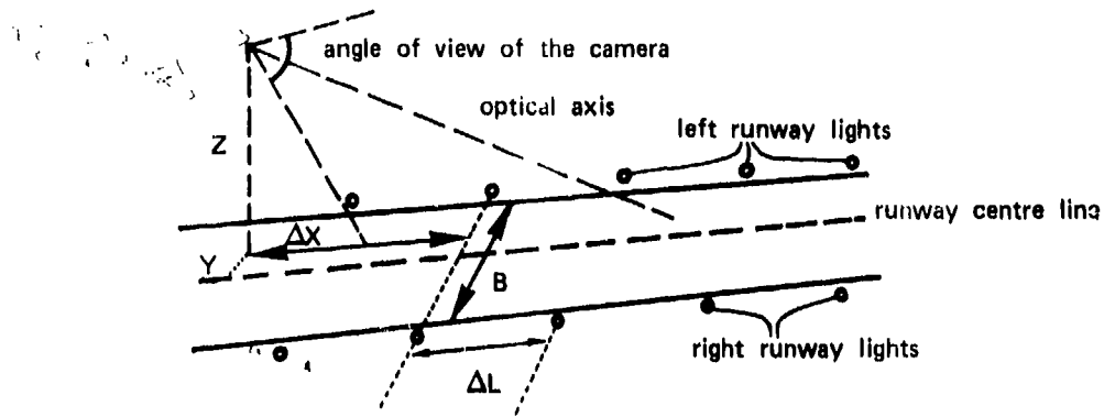
Fig. 17 Principle of the nose camera method
