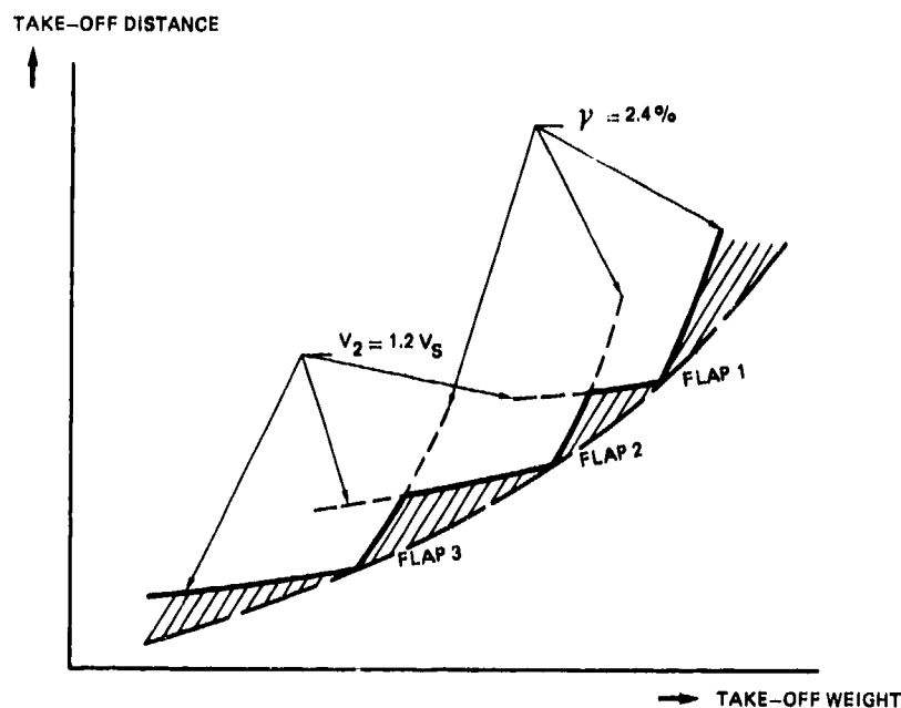
Fig. 3 Limitations of the take-off distance if only 3 flap settings are available
