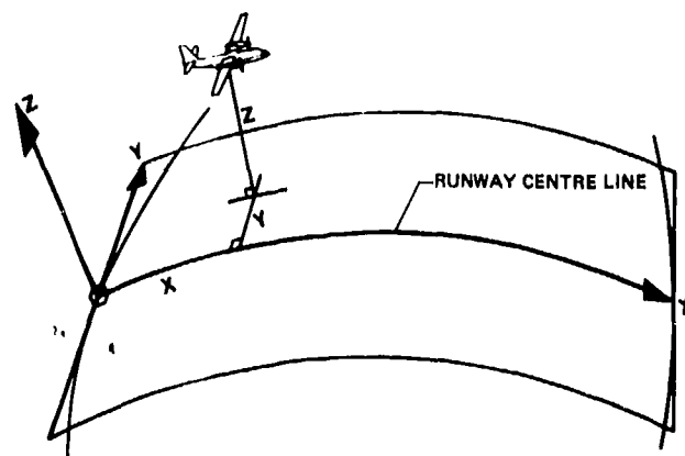
Fig. 31 The Lambert I co-ordinate system for take-off and landing measurements
