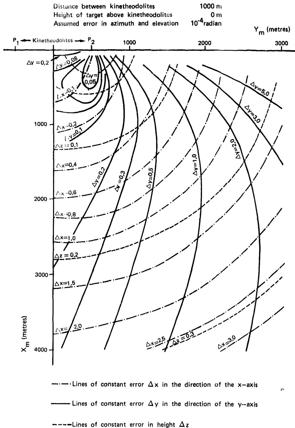
Fig. 13 Typical graph showing kinetheodolite errors for fixed values of the distance between the kinetheodolites (1000 m), height of the target (0 m) and assumed angular errors ( 10^{-4} radian)
