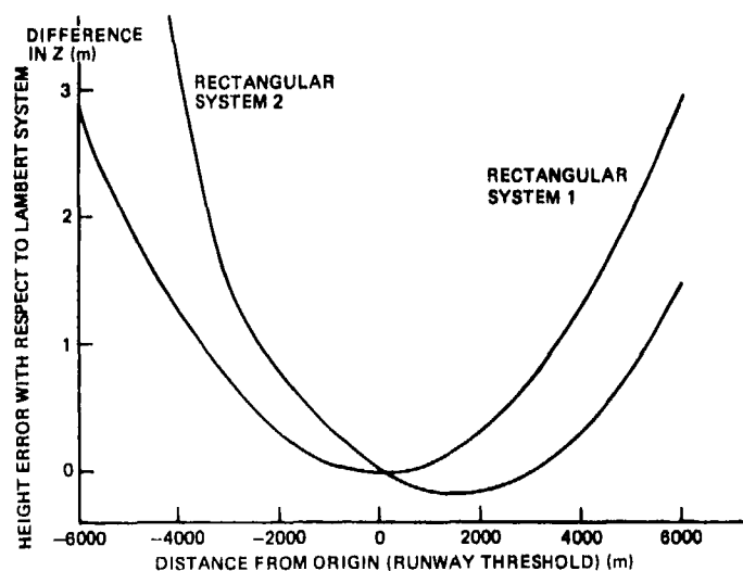
Fig. 33 Errors in aircraft height for the two rectangular co-ordinate systems
