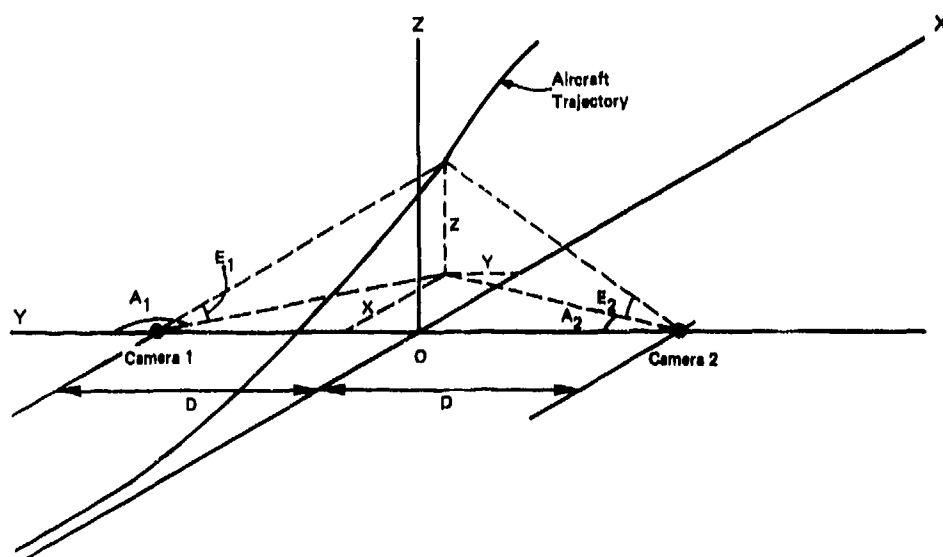
Fig. 7 Measurement of an aircraft trajectory using two kinetheodolites
