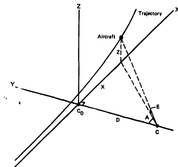
Fig. 6 Measurement of a take-off trajectory using a single kinetheodolite
