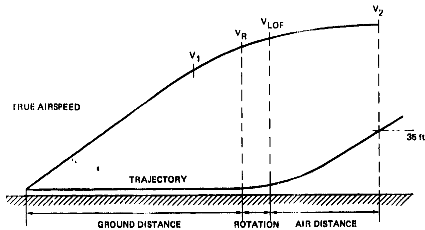
Fig. 1 The speed and trajectory schedule for a take-off
