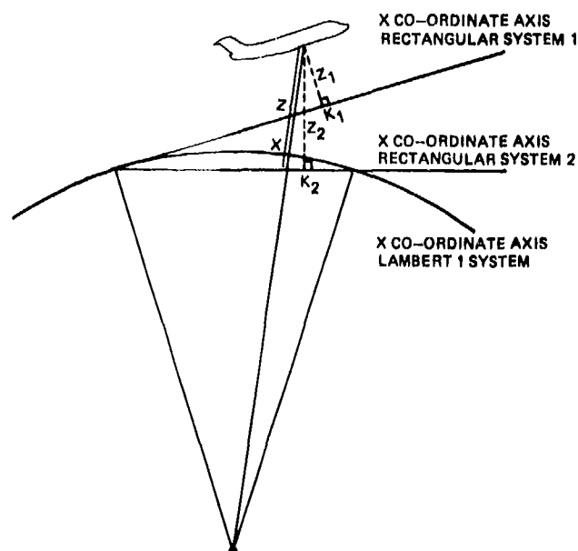
Fig. 32 The X and Z co-ordinates of the three co-ordinate systems discussed in the Appendix
