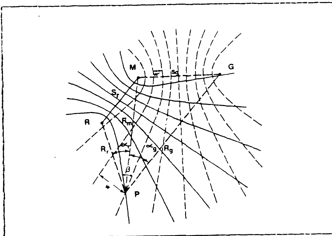
Figure 2.2 Geometry of a Hyperbolic-Hyperbolic Position
