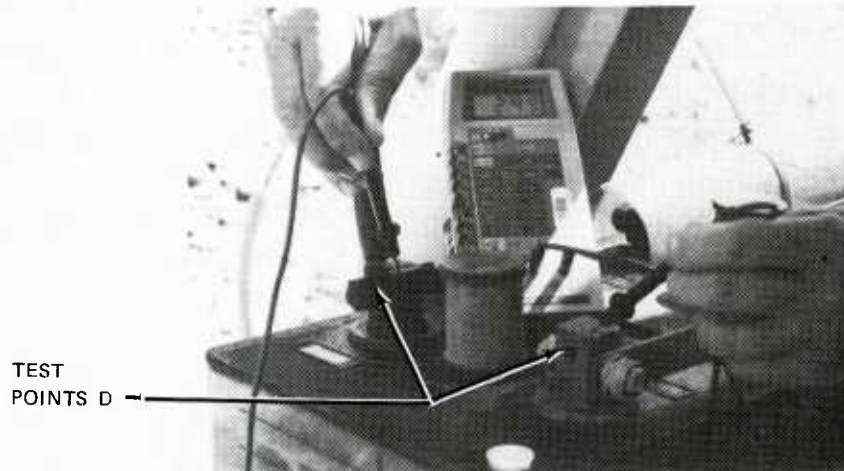
FIGURE 4-5. Measurement of Battery Cell Voltage.
