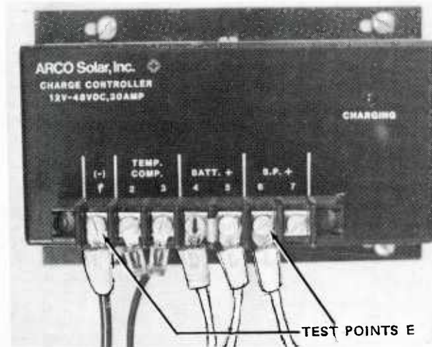
FIGURE 4-9. Bypassing the Array at the Voltage Regulator.
