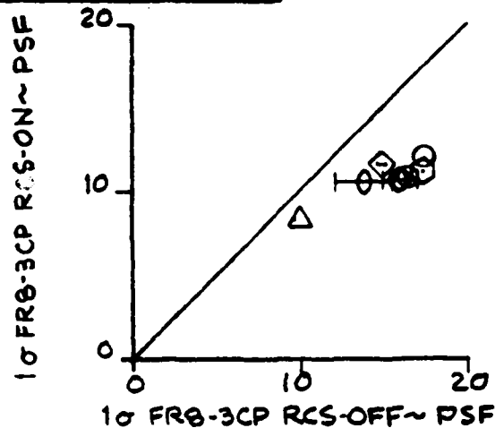
FIGURE 8-40 SEA STATE IV EFFECT OF RCS ON HEAVE ACCELERATION, CUSHION PRESSURE AND SHIP SPEED MAXIMUM SPEED-1900 LIFT FAN RPM
