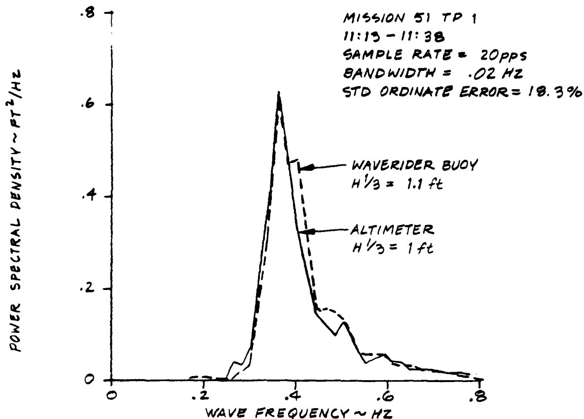
FIGURE B-2 SEA STATE I WAVE SPECTRA-MISSION 51
