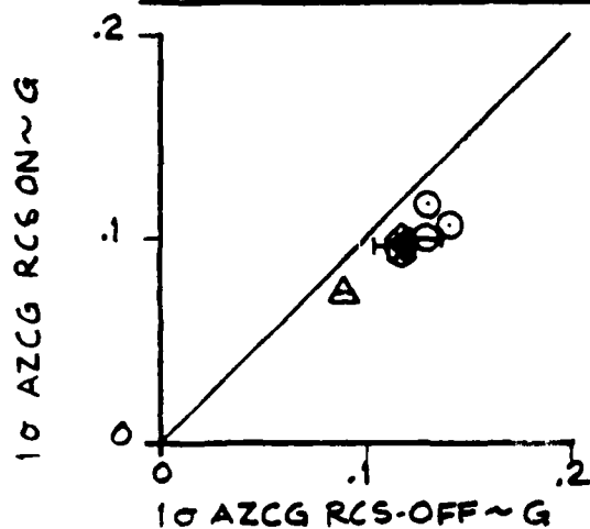
FIGURE 8-40 SEA STATE IV EFFECT OF RCS ON HEAVE ACCELERATION, CUSHION PRESSURE AND SHIP SPEED MAXIMUM SPEED-1900 LIFT FAN RPM
