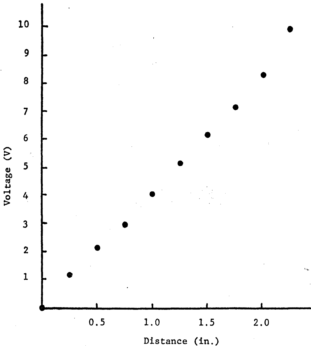
Figure 5-12. Voltage versus distance along a strip cut from Type A pad (Aquadag contacts)
