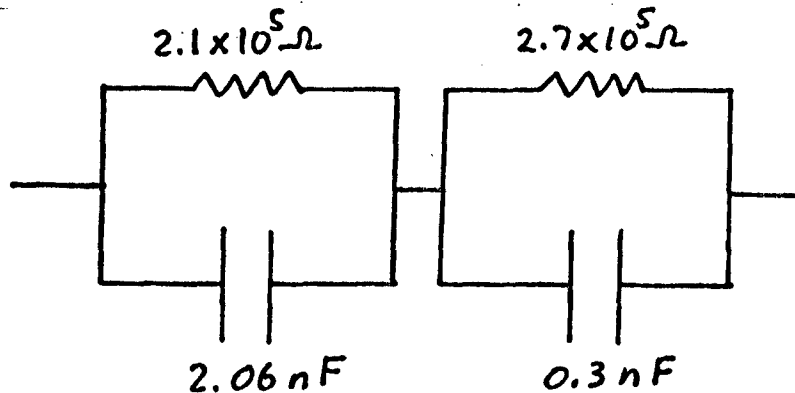
Figure A-3. Model for sample C4 derived from C and G measurements and the above equations.
