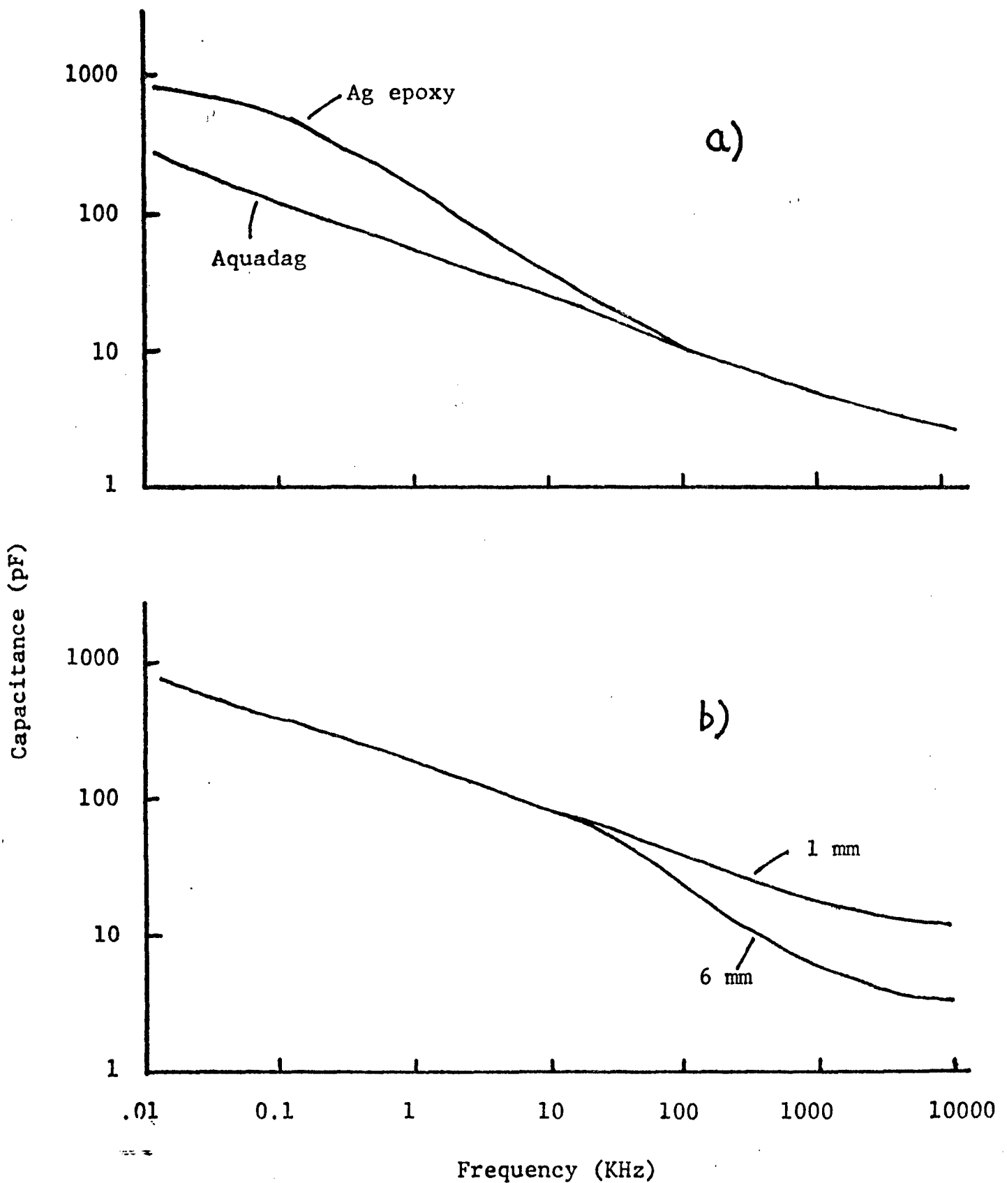
Figure A-2. Capacitance versus frequency for samples with a) different contacts (same thickness); b) different thickness (same contacts)
