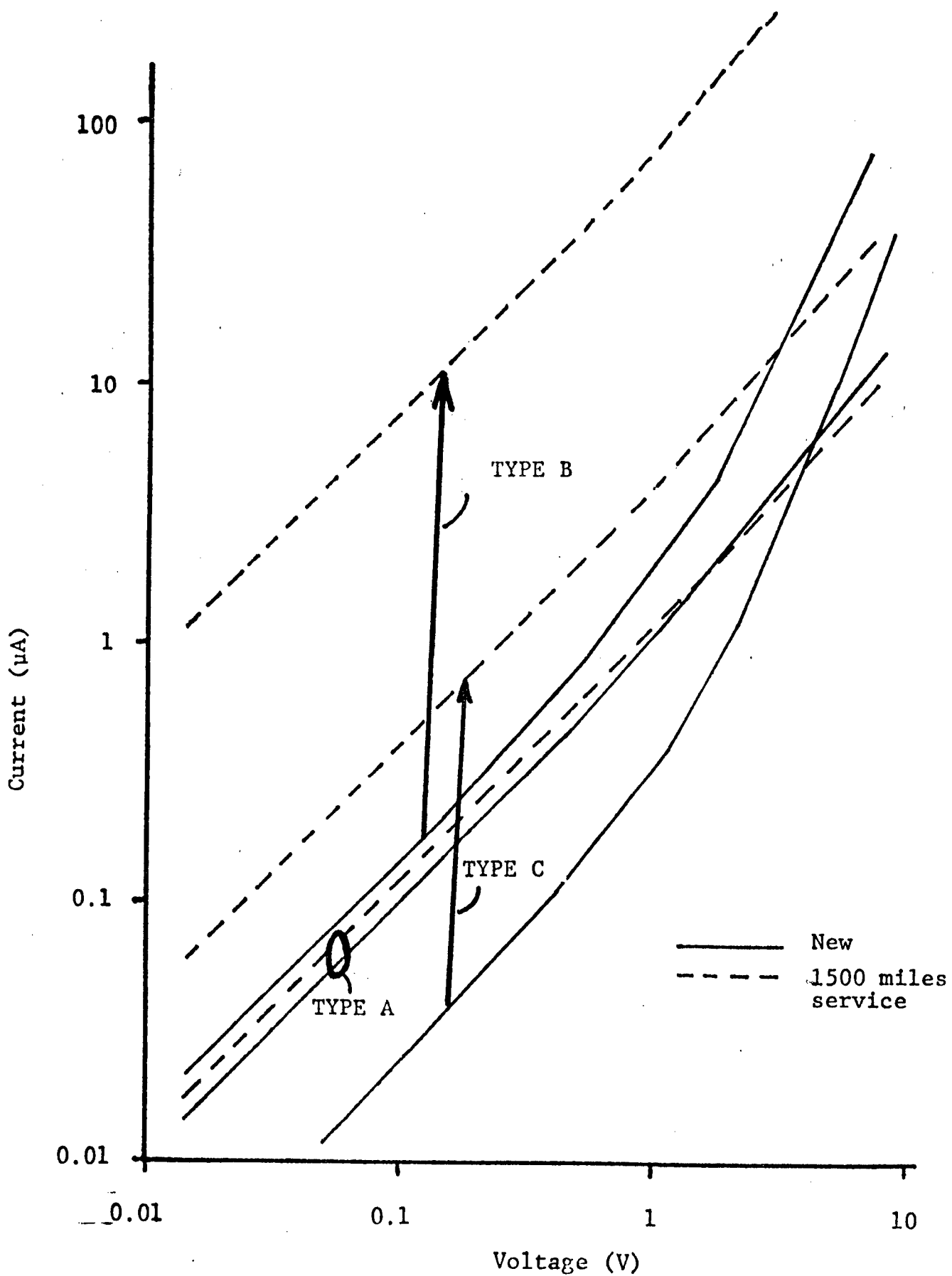
Figure 5-11. Current-voltage characteristics for samples cut from six pads (Identified in Addendum.)
