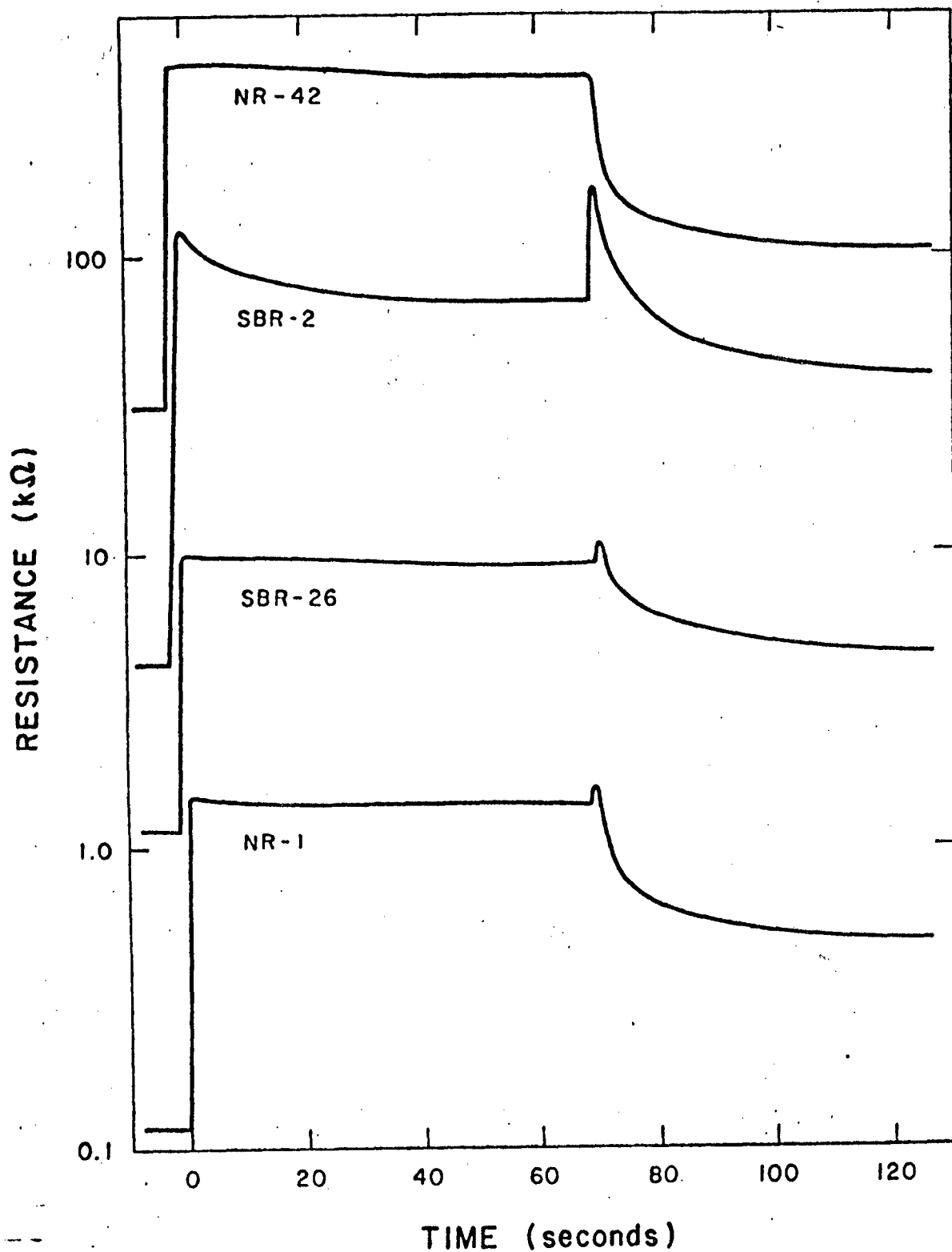
Figure 5-3. Typical resistance increase and relaxation curves for pressure applied at t=0 and removed at t=70 sec. (Curves displaced slightly for clarity)
