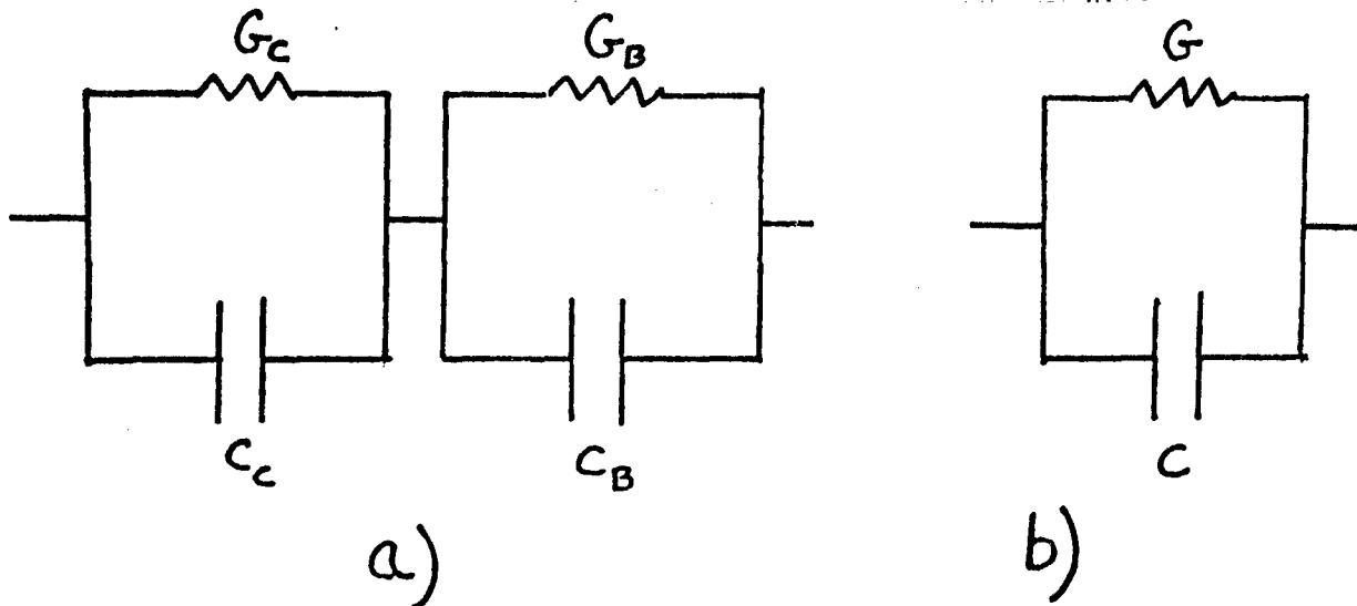
Figure A-1. a) Lumped model for rubber and contacts; b) Parallel combination read out on the Impedance Analyzer
