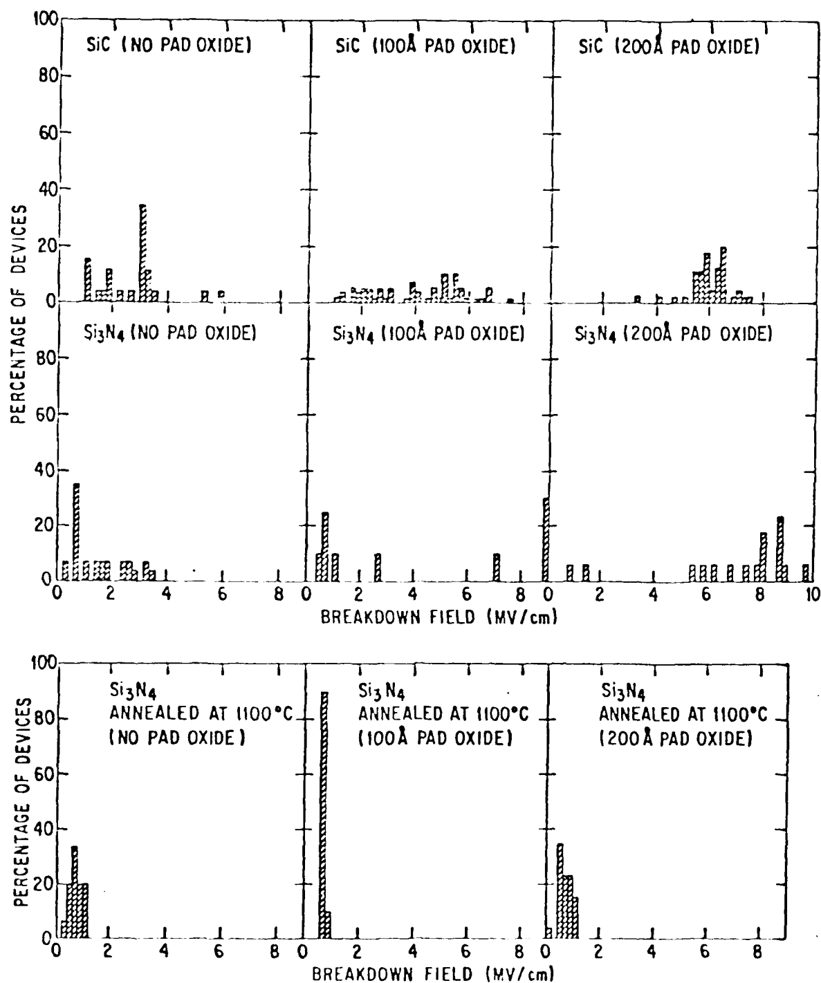
Fig. 3 MOS capacitor breakdown field histograms for carbide- and nitride-based processes with various pad oxide thickness.
