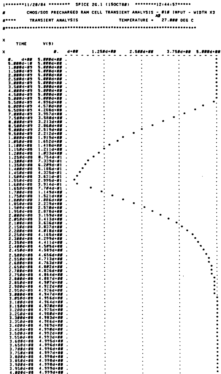
Figure B-25. SPICE Plot of Precharged RAM Cell Output, with Input 010 and Transmission Gate Widths Tripled.
