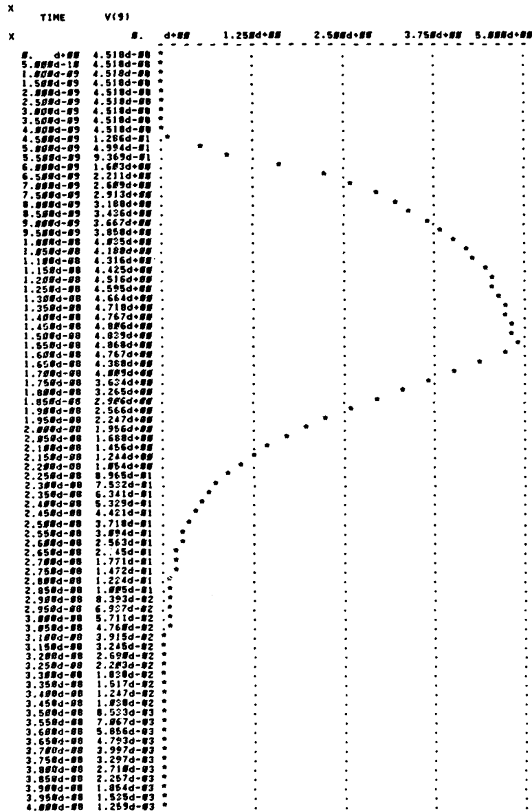
Figure B-24. SPICE Plot of Precharged RAM Cell with Input 101, and Transmission Gate Widths Twice the Basic Widths.
