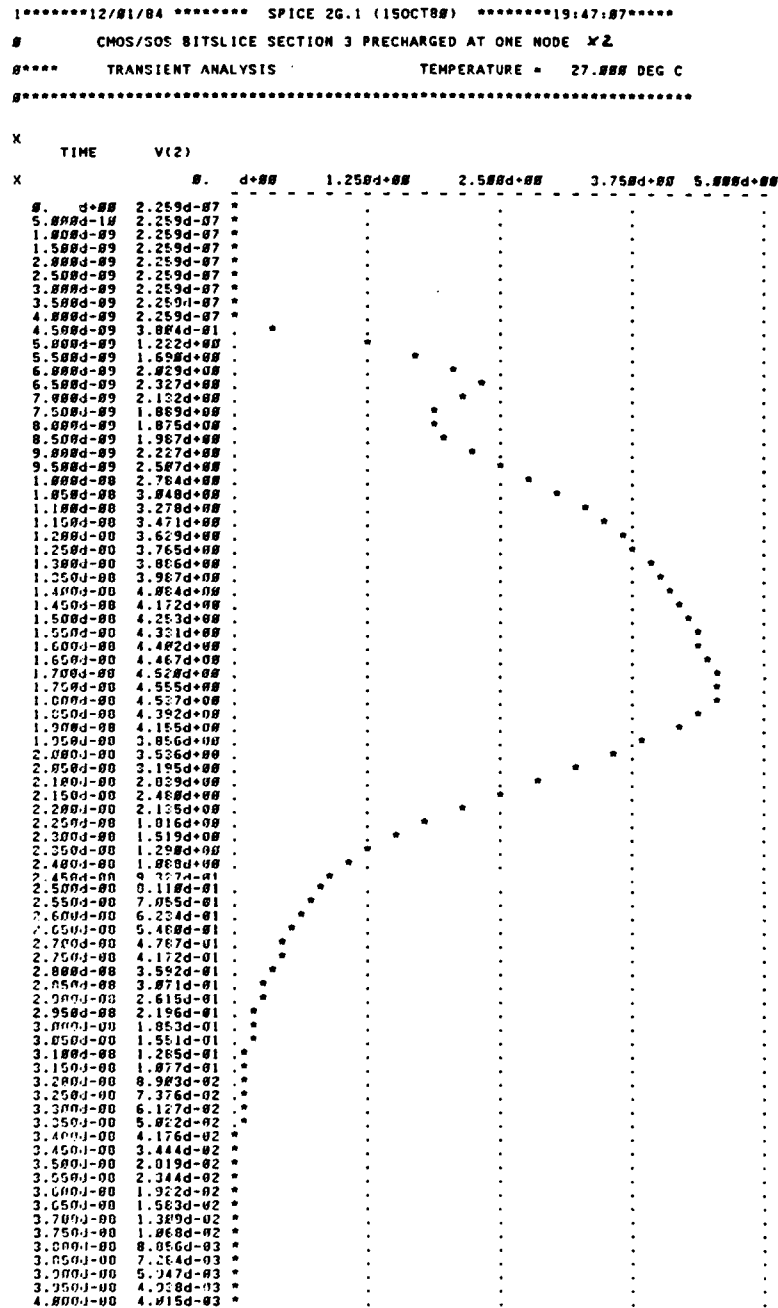
Figure C-50. SPICE Plot Section 3 Input 101 One Node Precharge with Widths x2.
