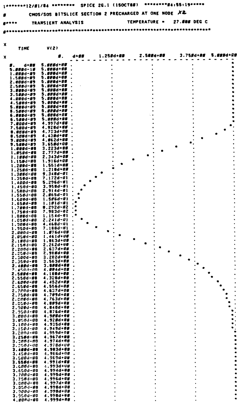
Figure C-29. SPICE Plot Section 2 Input 010 One Node Precharge with Widths x2
