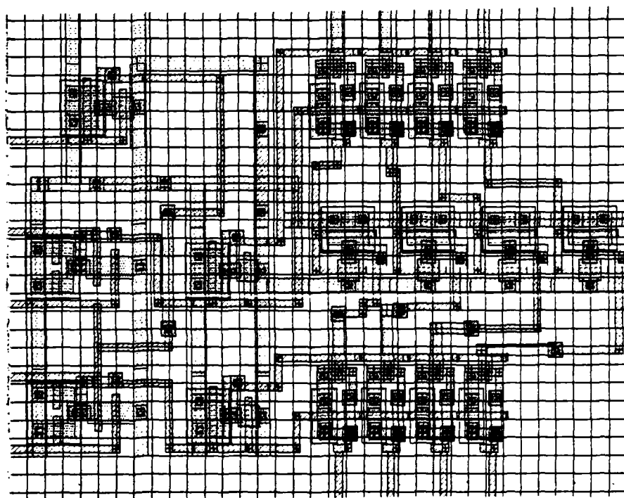
Figure VI-11. CLD Layout of B Register.
