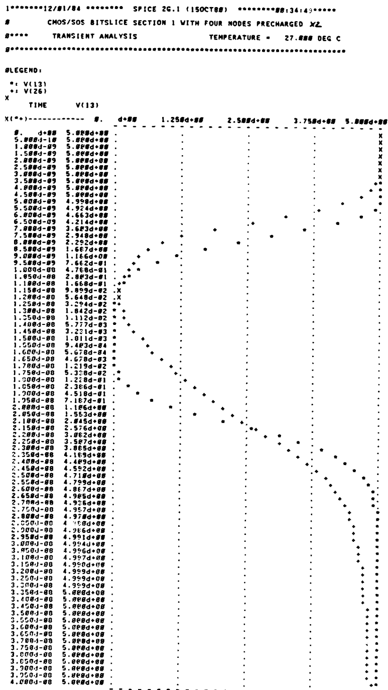
Figure C-17. SPICE Plot Section 1 Input 010 Four Node Precharge with Gate Widths x2
