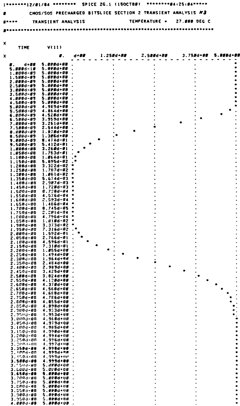
Figure C-39. SPICE Plot Section 2 Input 010 Two Node Precharge with Widths x3.
