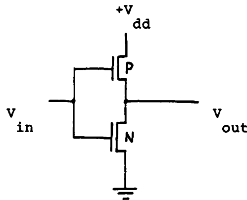
Figure II-1. CMOS inverter.
