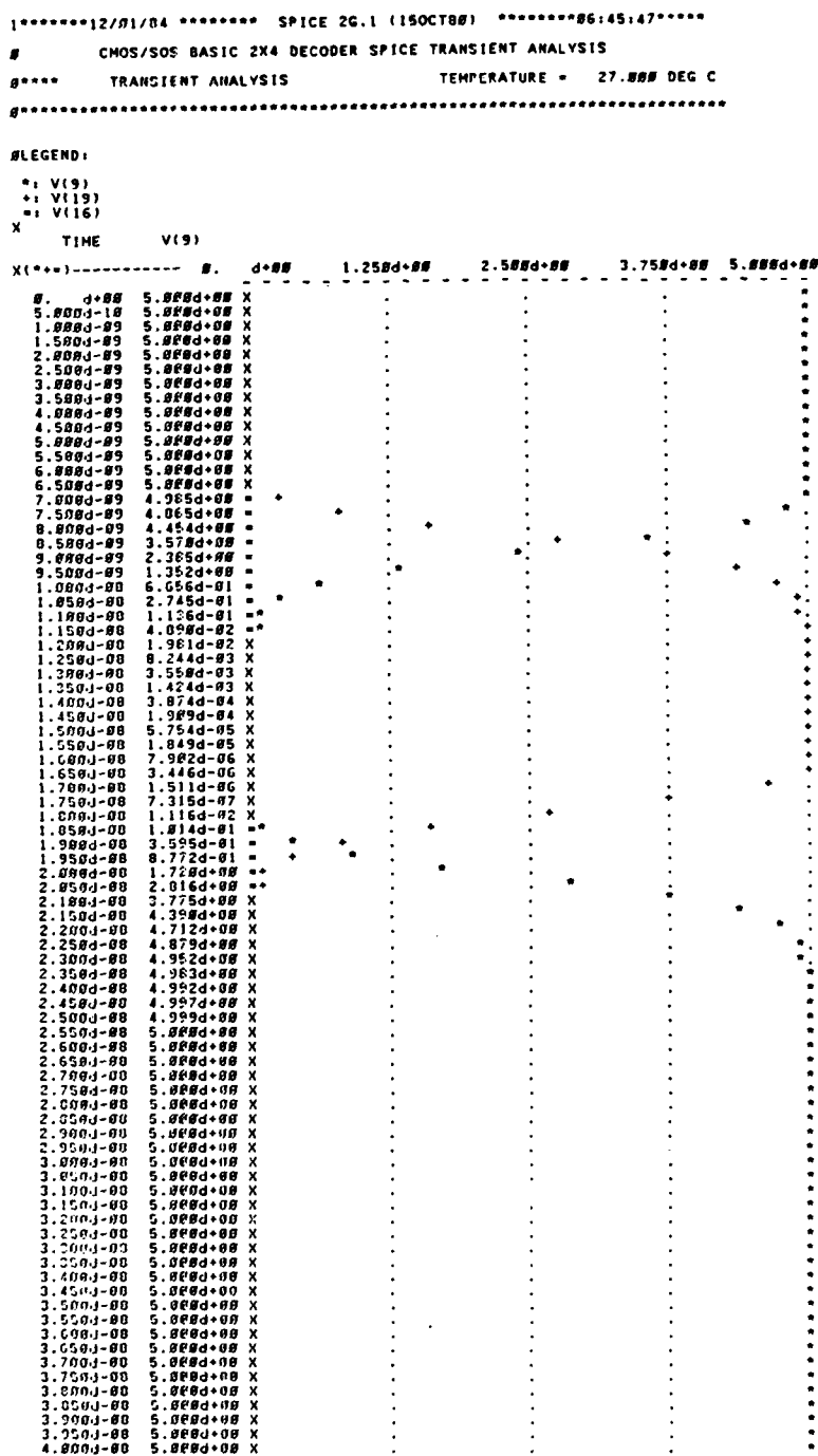
Figure B-2. SPICE Waveform Plot of Basic Decoder with Inputs 010.
