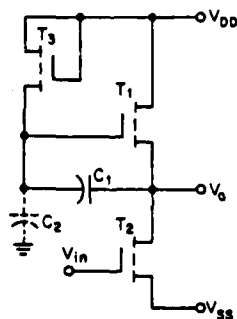
Figure IV-2. Bootstrap Pull-up circuit for increased drive capability [10].
