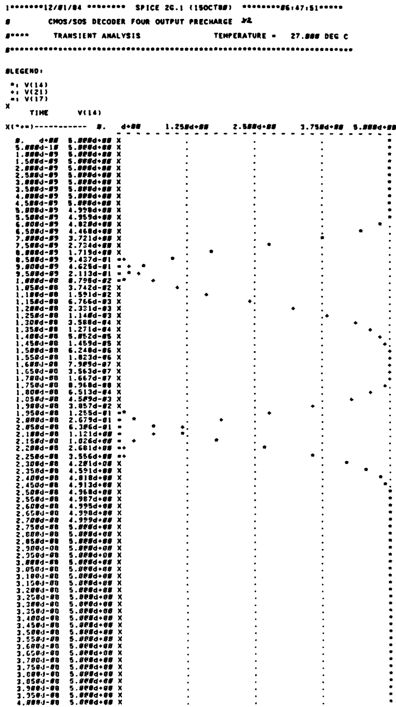
Figure B-5. SPICE Plot of Internal Node Precharged Decoder with Transmission Gate Widths Twice the Basic Widths.
