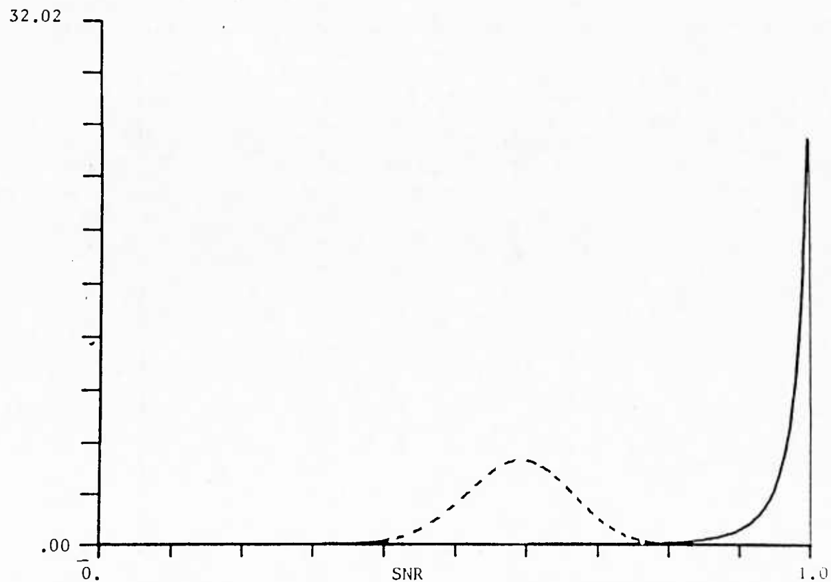
Fig. 7c) THEORETICAL PROBABILITY DENSITY OF SNR FOR TWO METHODS OF DATA DEPENDENT SNR IMPROVEMENT : INR=10 dB , f=.03 , K=45 , \rho=20 , \alpha=.9999 ——— USING FILTER WEIGHTS BASED ON THE PRINCIPAL EIGENVECTOR (1.15) ; - - - - - USING FILTER WEIGHTS BASED ON THE INVERSE OF THE ESTIMATED COVARIANCE MATRIX (1.09)
