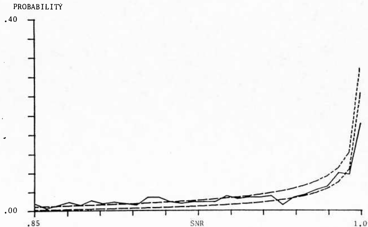
Fig. 4) 1'st ORDER AR NOISE PLUS WHITE NOISE INR=5 dB, SIGNAL FREQUENCY: f=.16 THE STATISTICS OF SNR ARE: MEAN = .93 STANDARD DEVIATION = 7.76E-2
