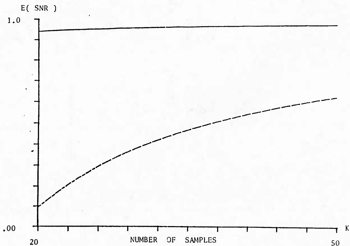
Fig. 6a) THEORETICAL EXPECTED VALUE OF SNR FOR TWO METHODS OF DATA DEPENDENT SNR IMPROVEMENT : \text{INR}=10 dB, f=.03 , \rho=20 , \alpha=.9999 ——— USING FILTER WEIGHTS BASED ON THE PRINCIPAL EIGENVECTOR (1.15) - - - - - USING FILTER WEIGHTS BASED ON THE INVERSE OF THE ESTIMATED COVARIANCE MATRIX (1.09)
