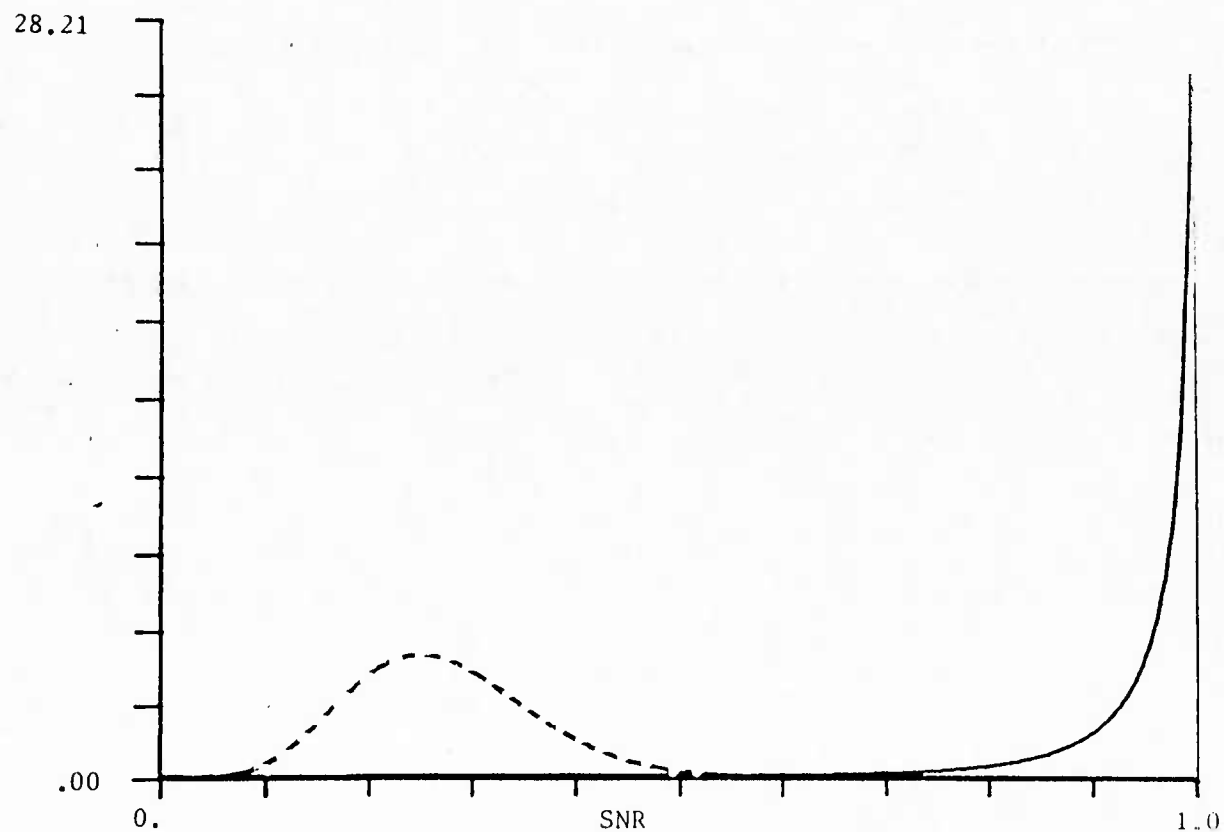
Fig. 7a) THEORETICAL PROBABILITY DENSITY OF SNR FOR TWO METHODS OF DATA DEPENDENT SNR IMPROVEMENT : \text{INR}=10 \text{ dB} , f=.03 , K=25 , \rho=20 , \alpha=.9999 ——— USING FILTER WEIGHTS BASED ON THE PRINCIPAL EIGENVECTOR (1.15) - - - - - USING FILTER WEIGHTS BASED ON THE INVERSE OF THE ESTIMATED COVARIANCE MATRIX (1.09)
