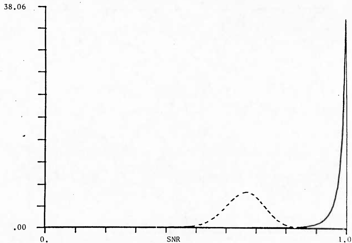
Fig. 7d) THEORETICAL PROBABILITY DENSITY OF SNR FOR TWO METHODS OF DATA DEPENDENT SNR IMPROVEMENT : INR=10 dB , f=.03 , K=55 , \rho=20 , \alpha=.9999 ——— USING FILTER WEIGHTS BASED ON THE PRINCIPAL EIGENVECTOR (1.15) - - - - - USING FILTER WEIGHTS BASED ON THE INVERSE OF THE ESTIMATED COVARIANCE MATRIX (1.09)
