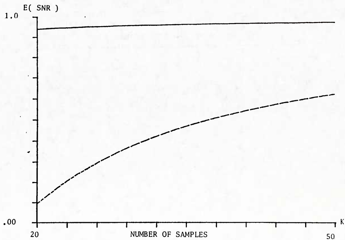
Fig. 6b) THEORETICAL EXPECTED VALUE OF SNR FOR TWO METHODS OF DATA DEPENDENT SNR IMPROVEMENT : \text{INR}=10 \text{ dB} , f=.04 , \rho=20 , \alpha=.9999 ——— USING FILTER WEIGHTS BASED ON THE PRINCIPAL EIGENVECTOR (1.15) - - - - USING FILTER WEIGHTS BASED ON THE INVERSE OF THE ESTIMATED COVARIANCE MATRIX (1.09)
