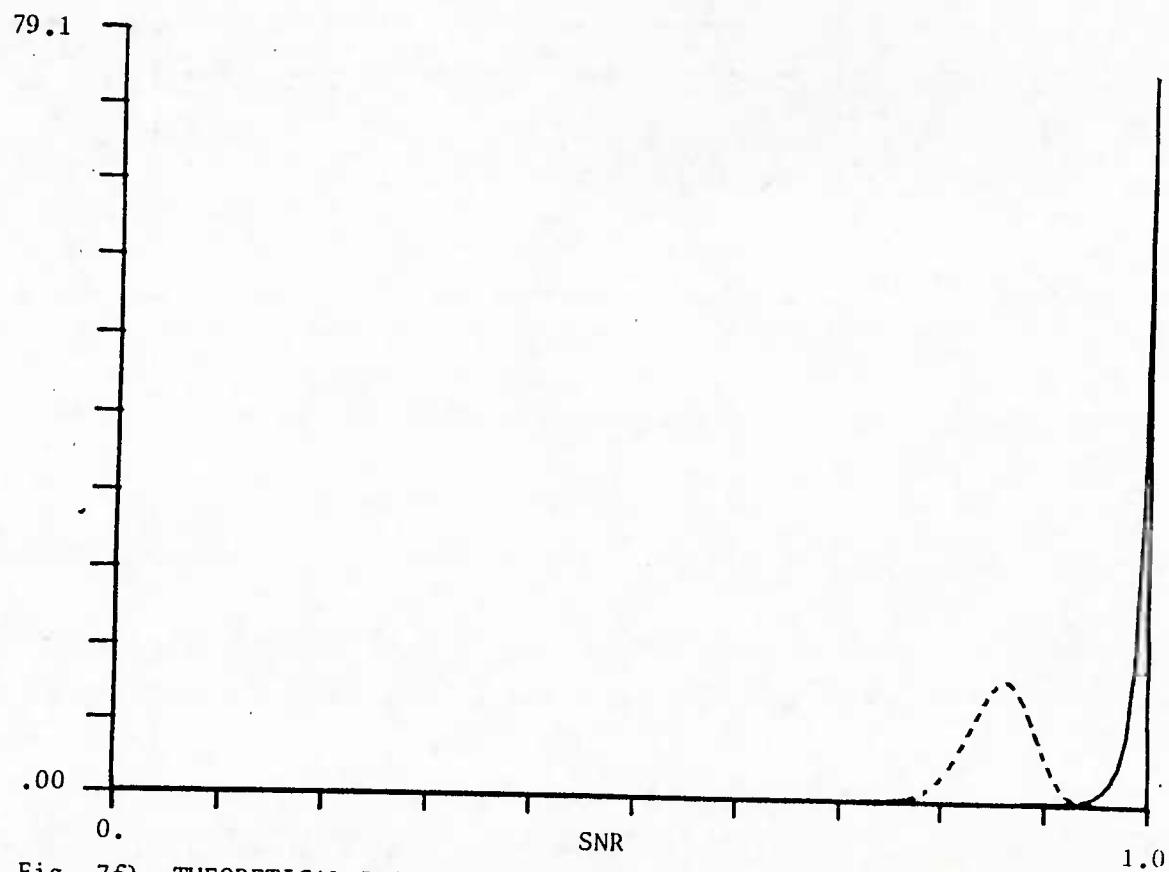
Fig. 7f) THEORETICAL PROBABILITY DENSITY OF SNR FOR TWO METHODS OF DATA DEPENDENT SNR IMPROVEMENT : \text{INR}=10 \text{ dB} , f=.03 , K=130 , \rho=20 , \alpha=.9999 ——— USING FILTER WEIGHTS BASED ON THE PRINCIPAL EIGENVECTOR (1.15) - - - - USING FILTER WEIGHTS BASED ON THE INVERSE OF THE ESTIMATED COVARIANCE MATRIX (1.09)
