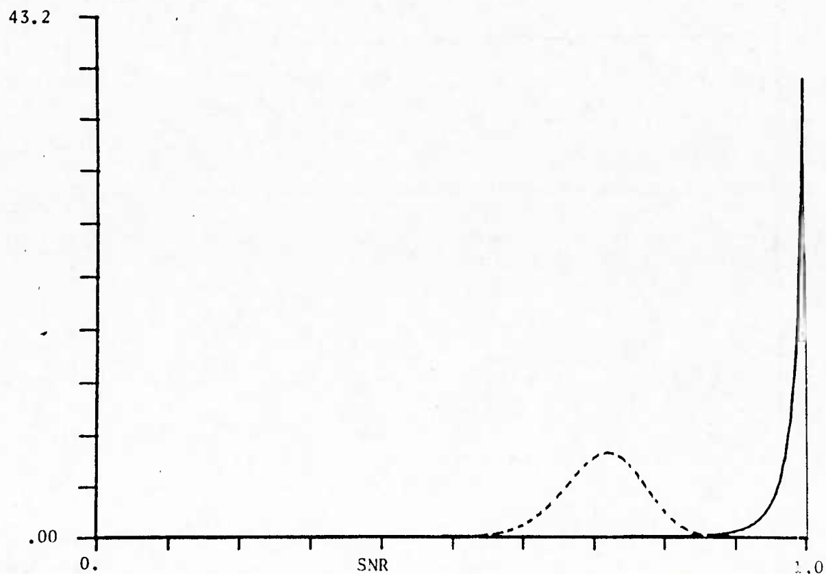
Fig. 7e) THEORETICAL PROBABILITY DENSITY OF SNR FOR TWO METHODS OF DATA DEPENDENT SNR IMPROVEMENT : INR=10 dB , f=.03 , K=65 , p=20 , \alpha=.9999 ——— USING FILTER WEIGHTS BASED ON THE PRINCIPAL EIGENVECTOR (1.15) - - - - - USING FILTER WEIGHTS BASED ON THE INVERSE OF THE ESTIMATED COVARIANCE MATRIX (1.09)
