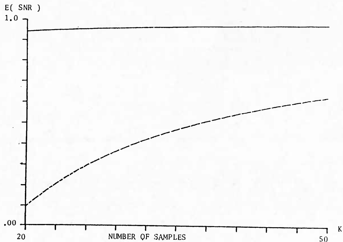
Fig. 6c) THEORETICAL EXPECTED VALUE OF SNR FOR TWO METHODS OF DATA DEPENDENT SNR IMPROVEMENT : INR=10 dB, f=.05 , \rho=20 , \alpha=.9999 ——— USING FILTER WEIGHTS BASED ON THE PRINCIPAL EIGENVECTOR (1.15) - - - - - USING FILTER WEIGHTS BASED ON THE INVERSE OF THE ESTIMATED COVARIANCE MATRIX (1.09)
