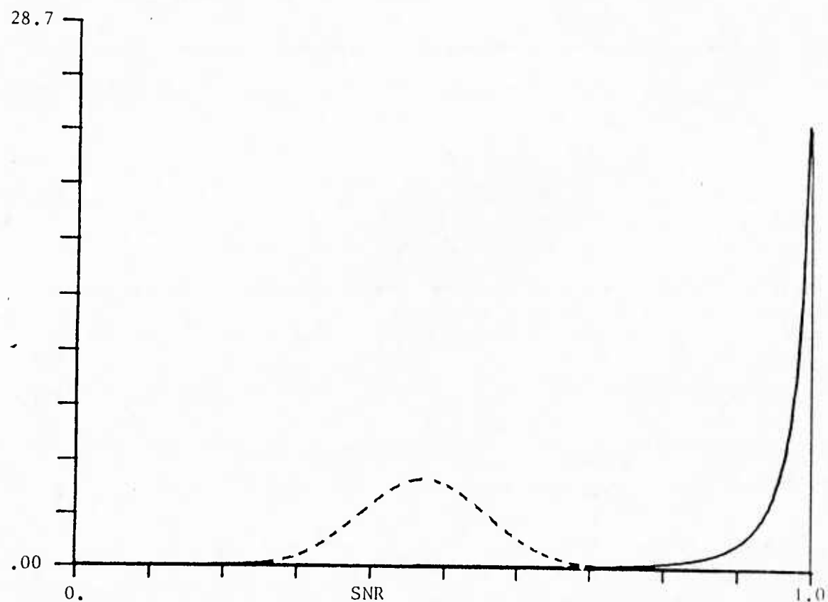
Fig. 7b) THEORETICAL PROBABILITY DENSITY OF SNR FOR TWO METHODS OF DATA DEPENDENT SNR IMPROVEMENT : INR=10 DB , f=.03 , K=35 , \rho=20 , \alpha=.9999 ——— USING FILTER WEIGHTS BASED ON THE PRINCIPAL EIGENVECTOR (1.15) - - - - - USING FILTER WEIGHTS BASED ON THE INVERSE OF THE ESTIMATED COVARIANCE MATRIX (1.09)
