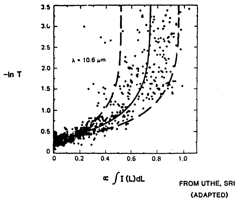
FIGURE 8. Lidar data and theory comparison for a phosphorus smoke cloud
