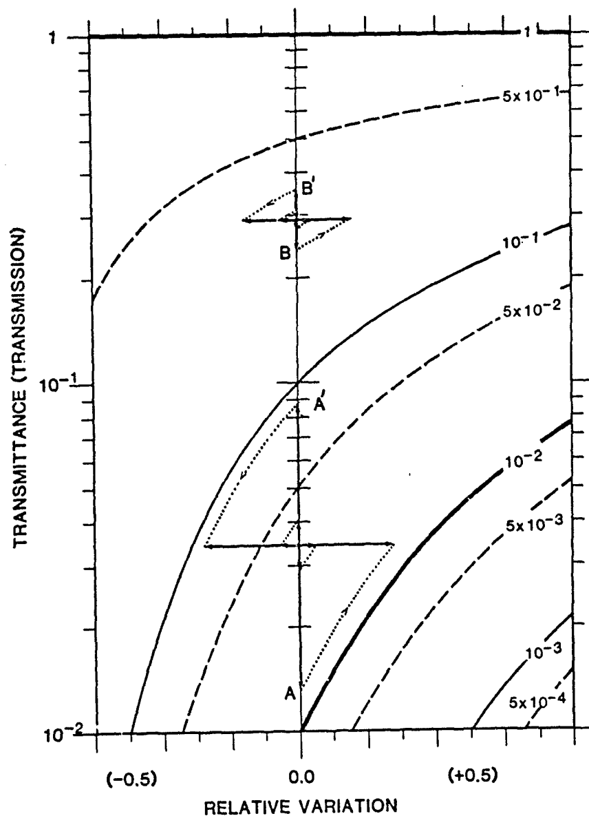
Figure 16. The upper left portion outlined by dots in Figure 13, enlarged, with the fluctuations of Figure 14 plotted thereon (AA' and BB'). The uncertainties due to a 5% residual or systematic relative error (inner horizontal arrows) in the attenuation coefficient measurements used to determine transmittance are shown by the inner vertical arrows.
