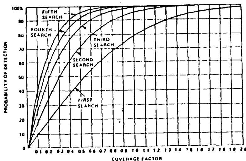
Figure 9. Probability of Detection
