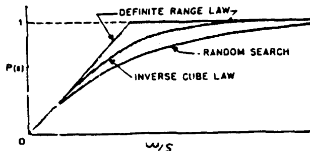
Figure 11. Probability of Detection for Parallel Sweep
