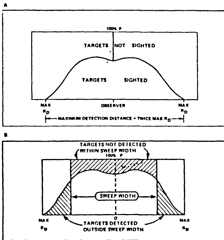
Figure 6. Graphic Presentation of Sweep Width
