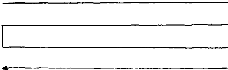
Parallel search
