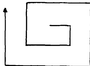
Barrier Search
