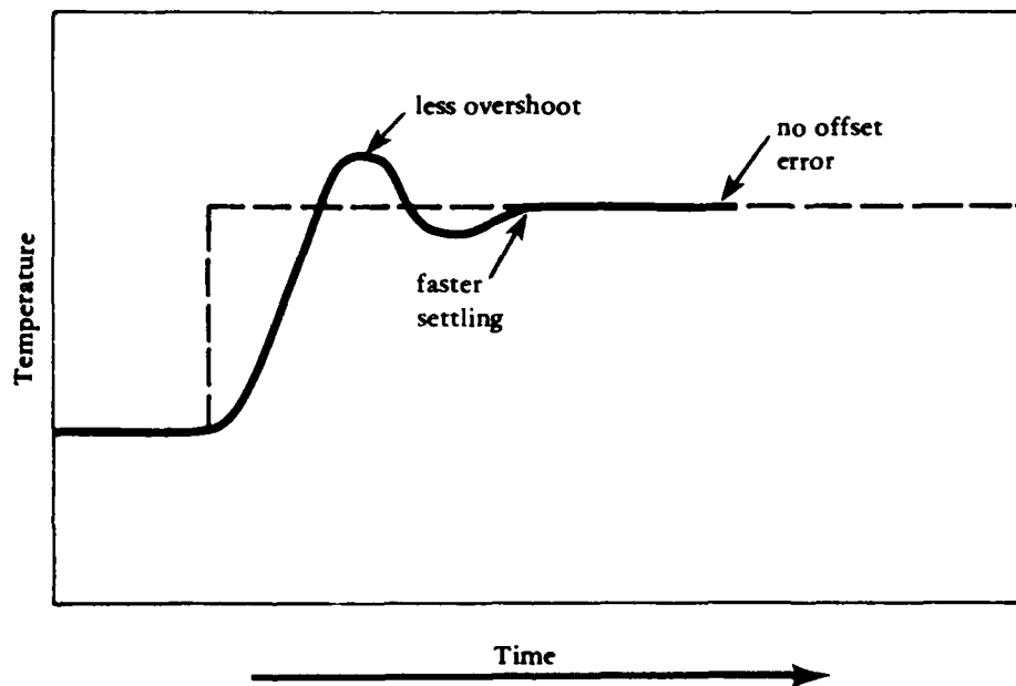
Figure 10. Proportional/integral/derivative control.
