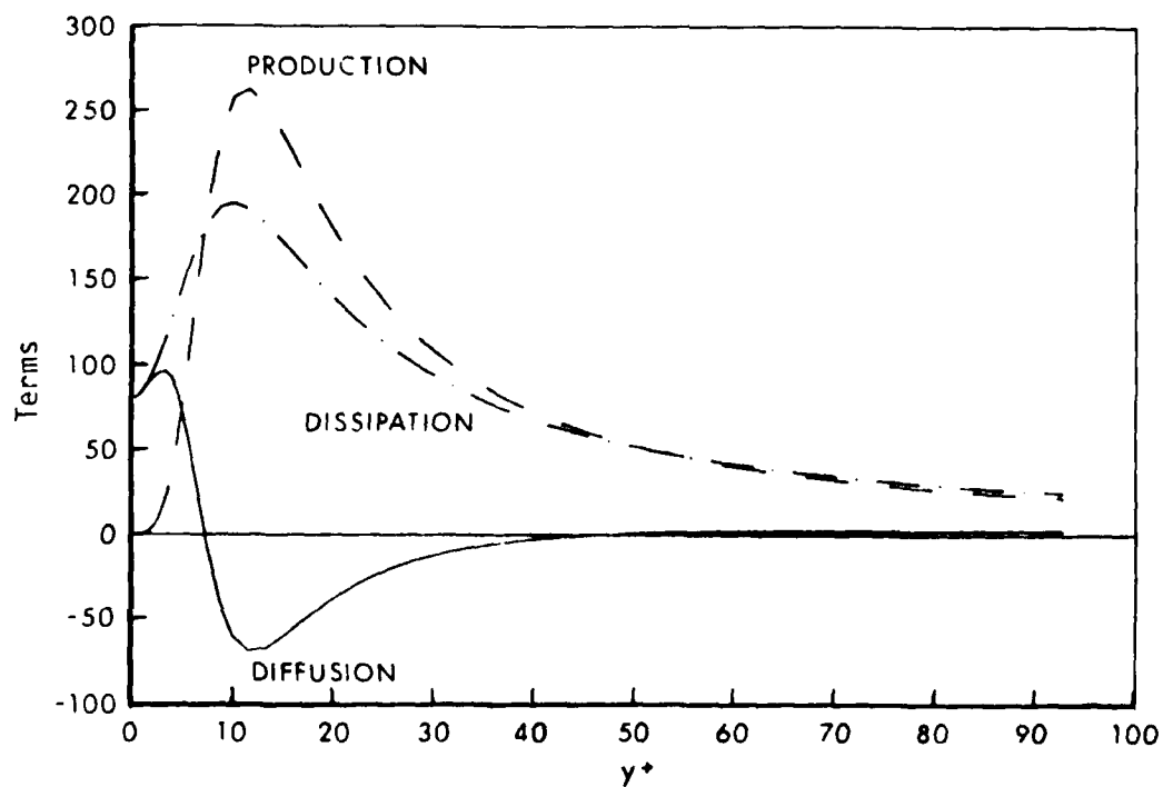
Figure 2. Balance of Terms in the k-equation (Reference 41)
