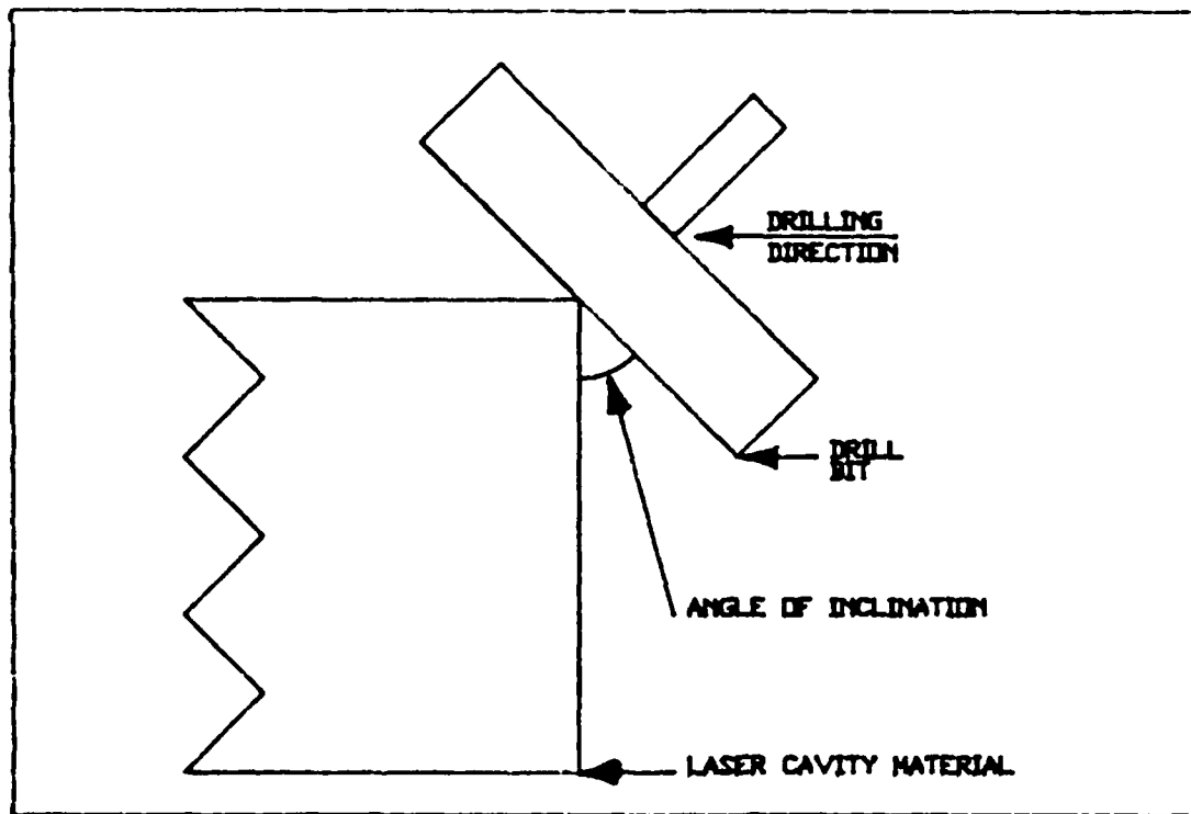
Figure 3.1 Drilling the Elliptical Cavity
