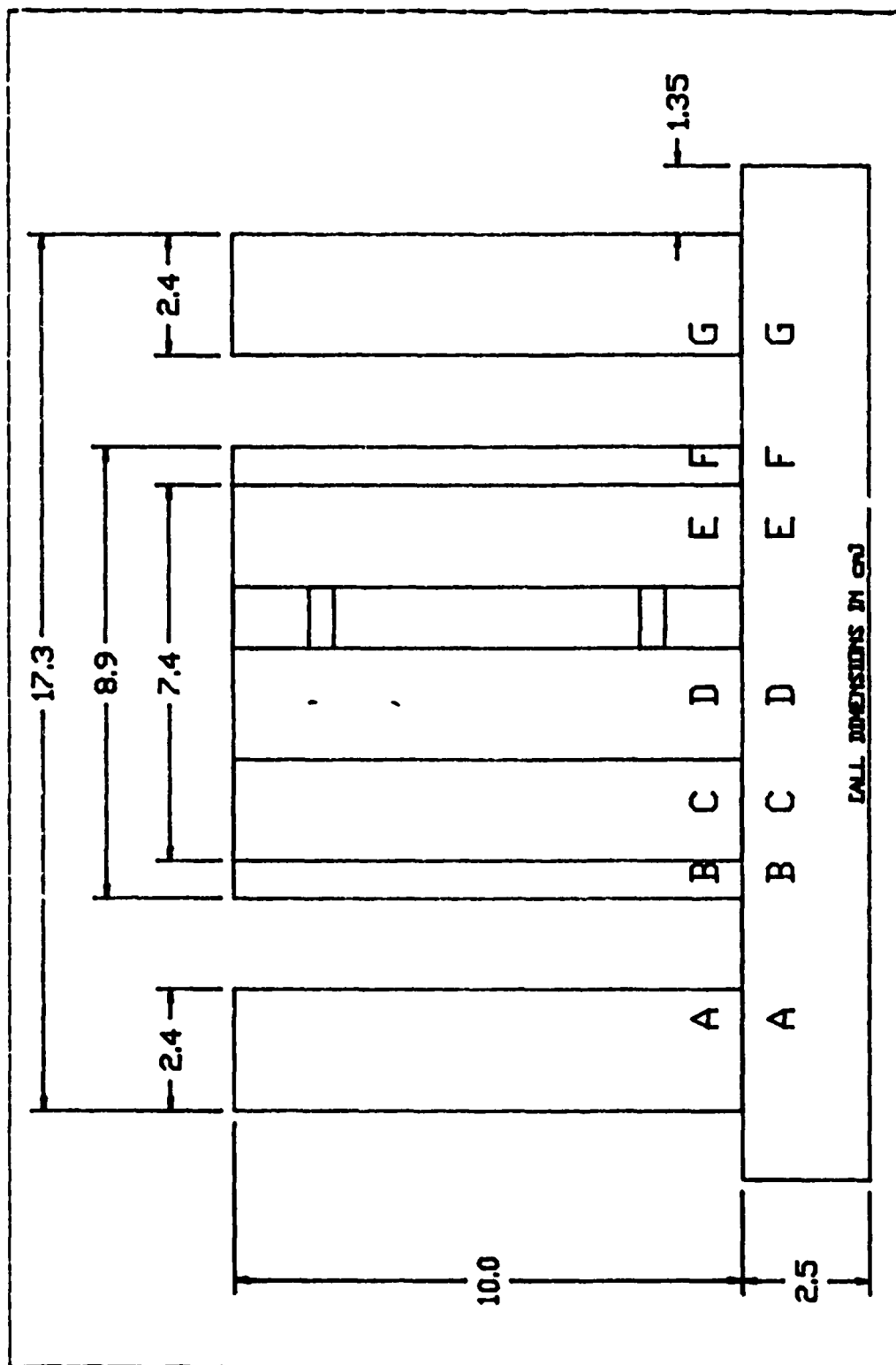
Figure 3.3 Cooling Cavity Dimensions
