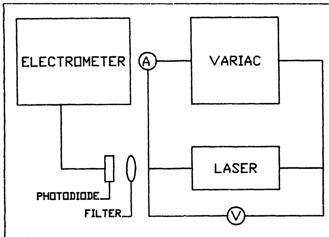
Figure 4.2 Fluorescence Measurement Set Up
