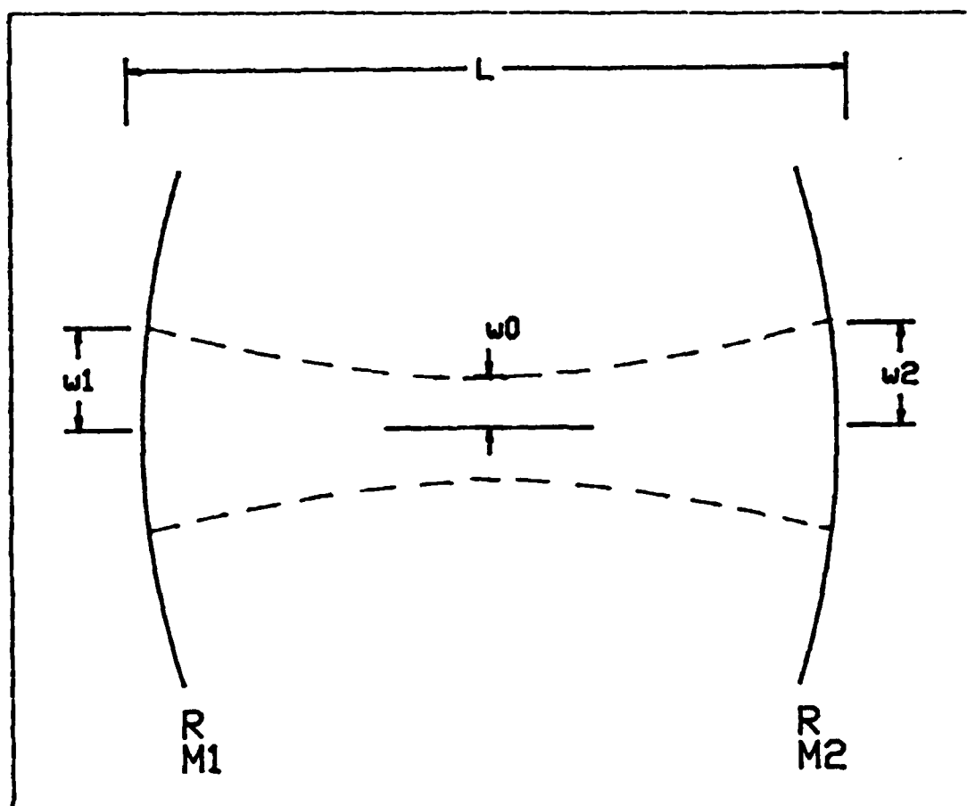
Figure 2.3 A Confocal Resonator
