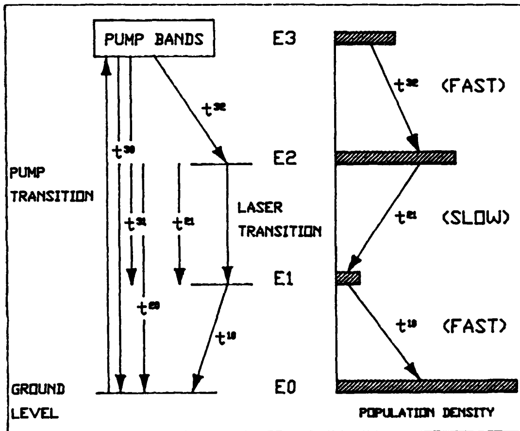
Figure 2.1 A General Four Level Laser
