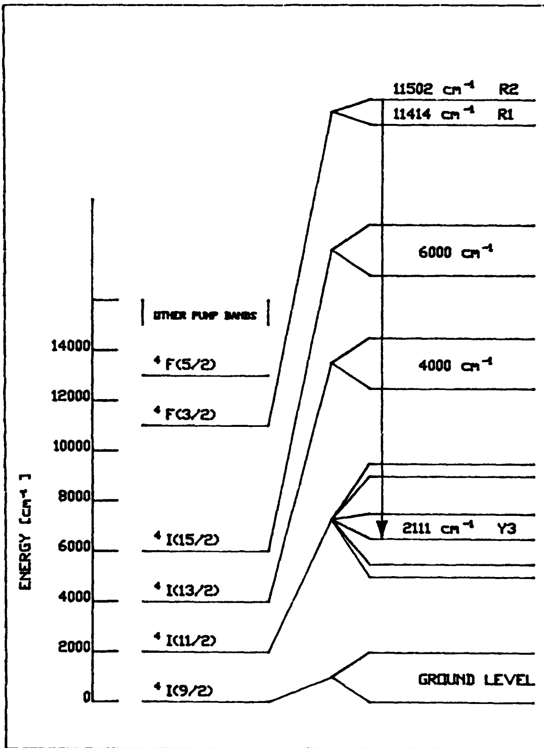
Figure 2.2 Nd:YAG Energy Levels
