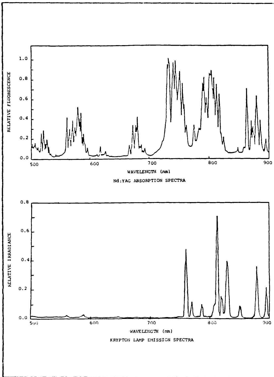
Figure 2.5 Krypton Emission and Nd:YAG Absorption Spectra
