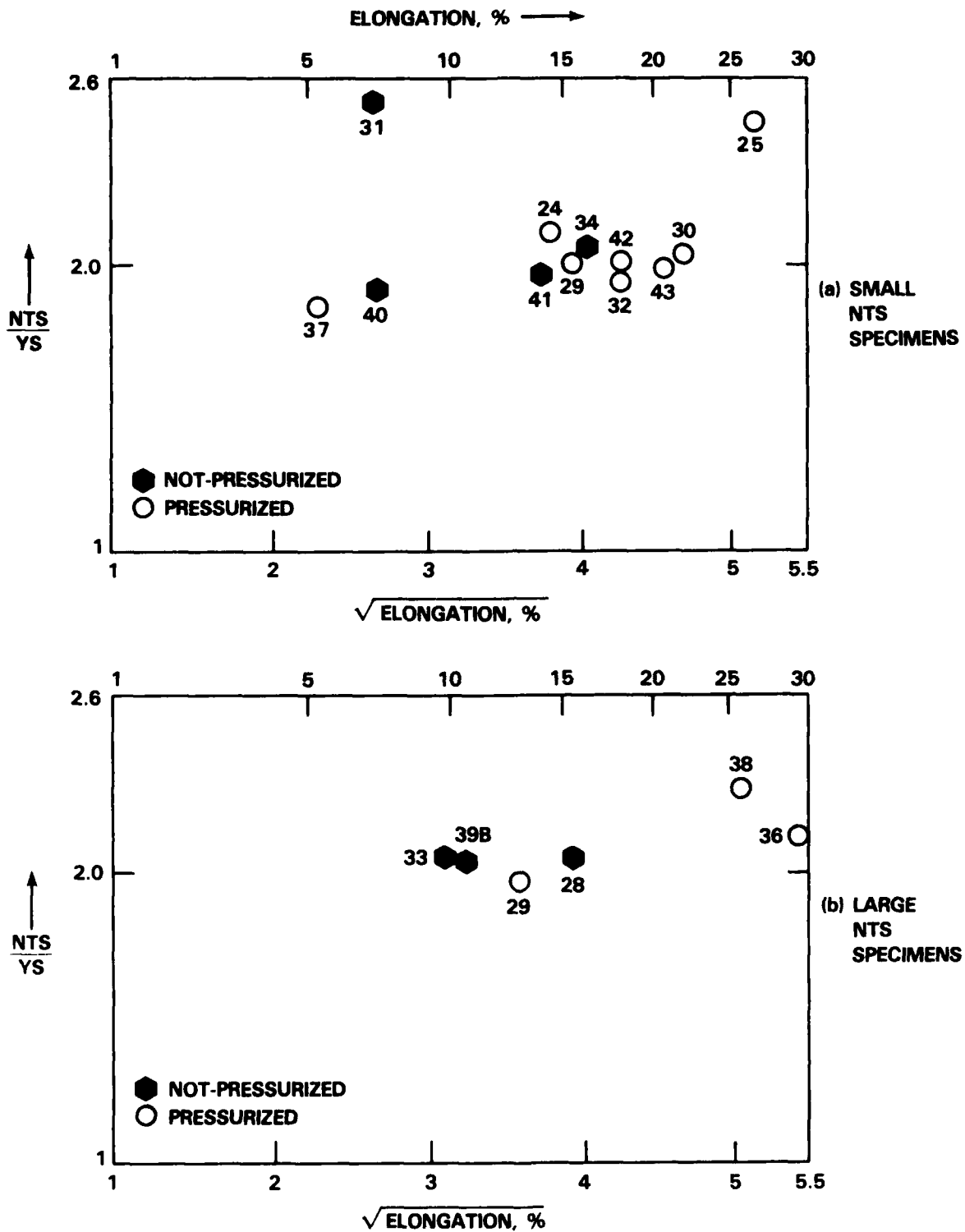
FIGURE 3. NTS/YS RATIO VS. \sqrt{\text{ELONGATION}}
