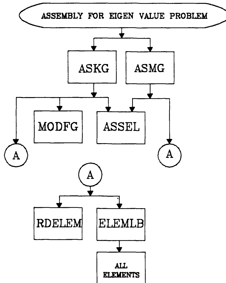
ASSEMBLY FUNCTIONS FOR EIGEN VALUE PROBLEM
