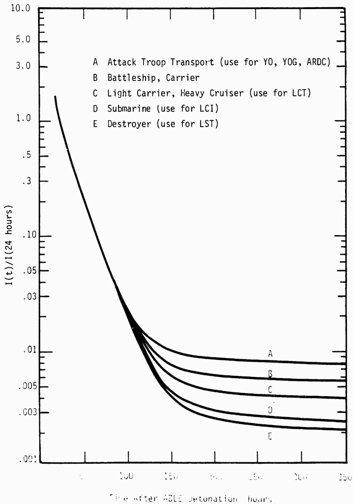
Figure 2-4 Shot ABLE Ship Intensities Relative to Intensity at 24 Hours
