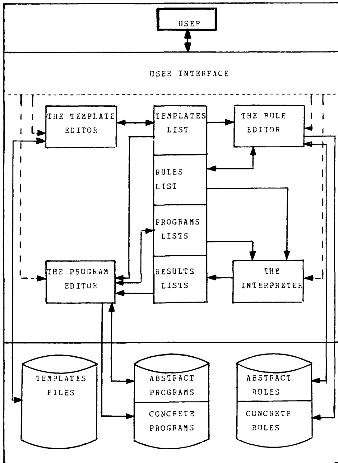
Figure 3.1 General Architecture of the System.
