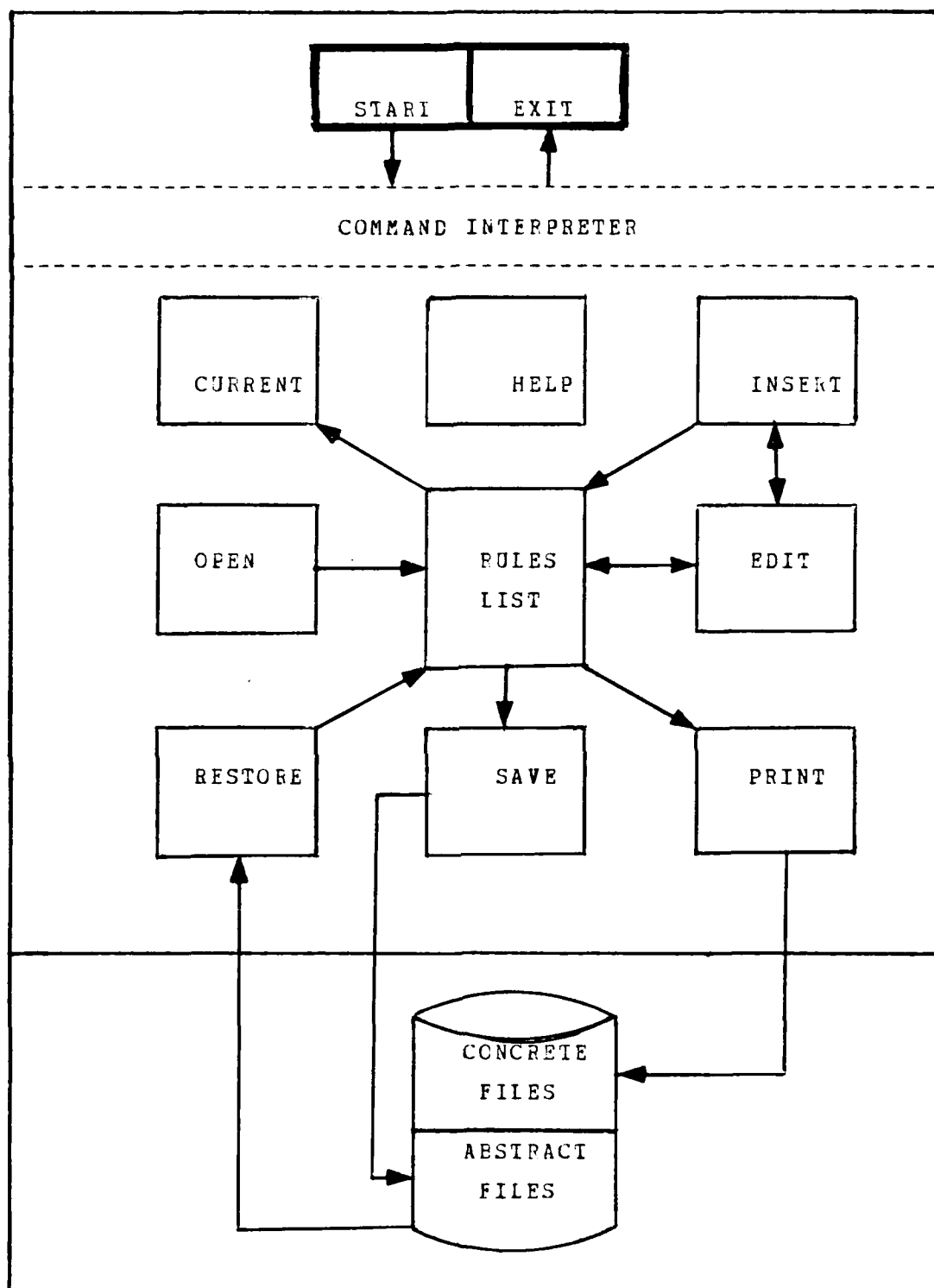
Figure 3.6 Architecture of the Rule Editor.
