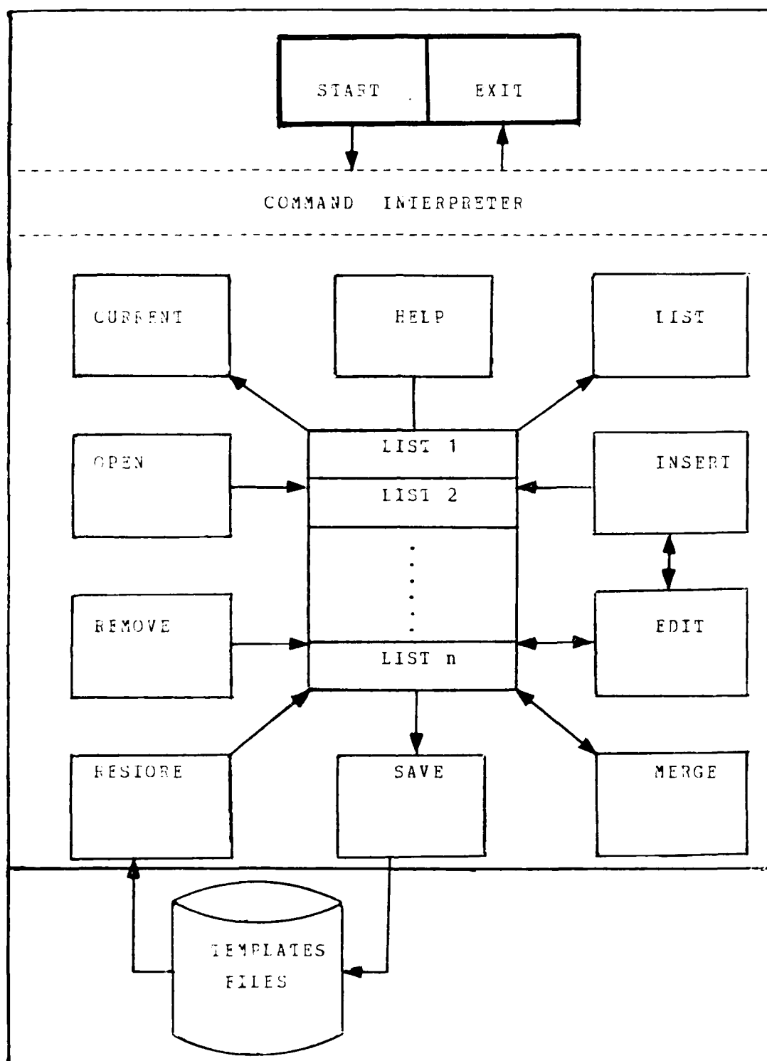
Figure 3.2 Architecture of the Template Editor.
