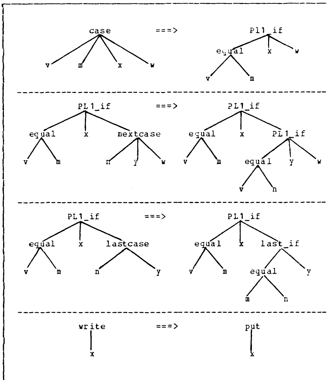
Figure 4.3 Abstract Transformation Rules for Case.
