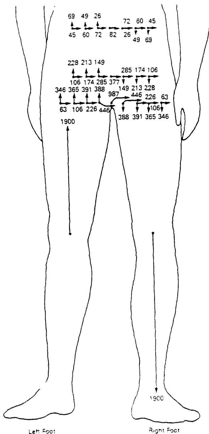
Figure 2.5 Current densities in a homogeneous man model exposed to an electric field in the ground on which he is standing. The total current entering the man through his left foot is 100 A. Current-density values are given in nA/cm 2 .
