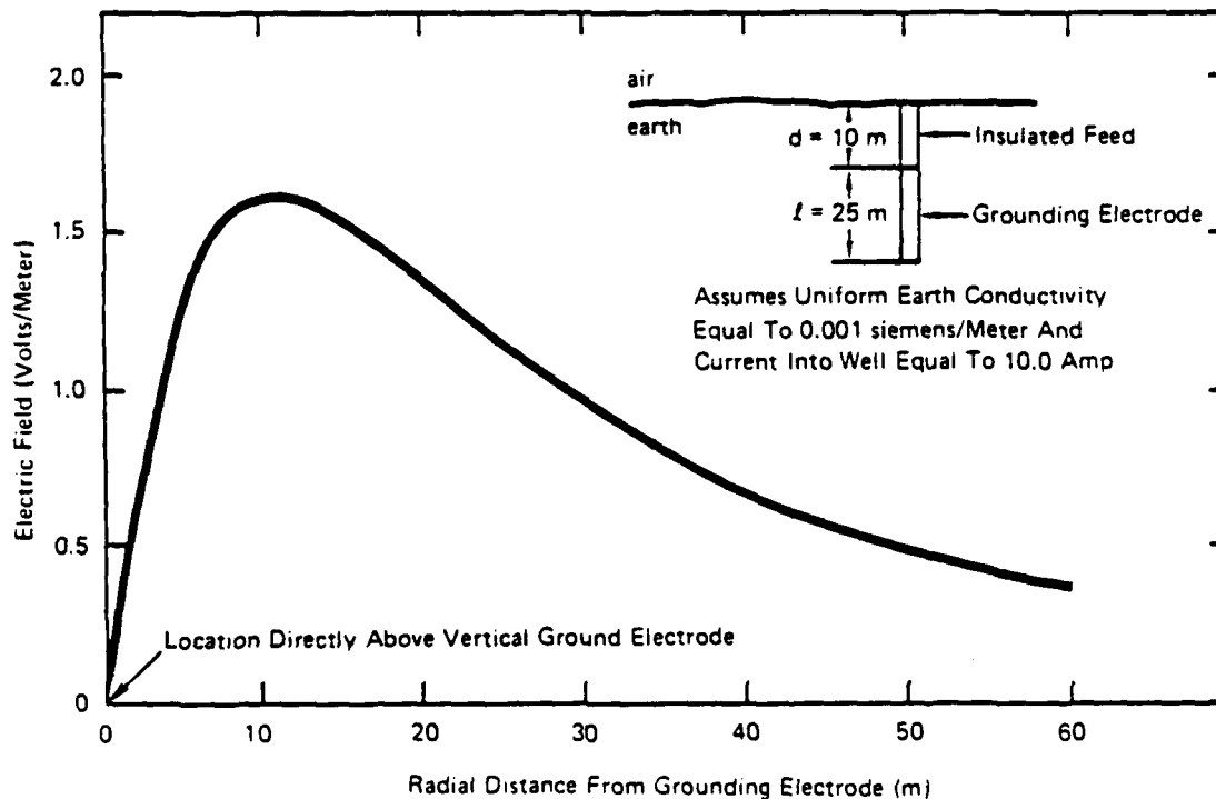
Figure 16. Surface Electric Field Strength Near a Vertical Well Ground.
