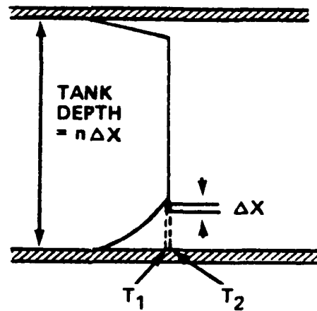
b. Diagram of Holdup Calculation
