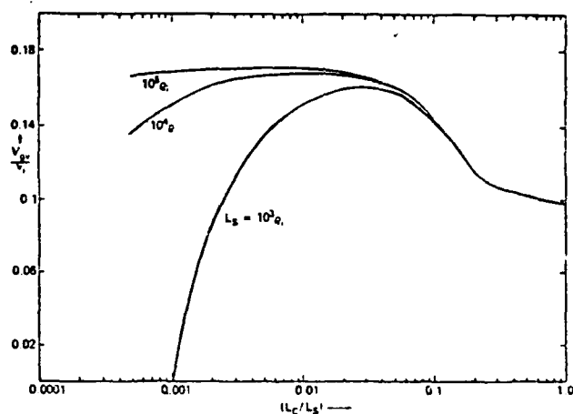
Fig. 4. Plot of V_g against L_c/L_s for the parameter range of figure 3
