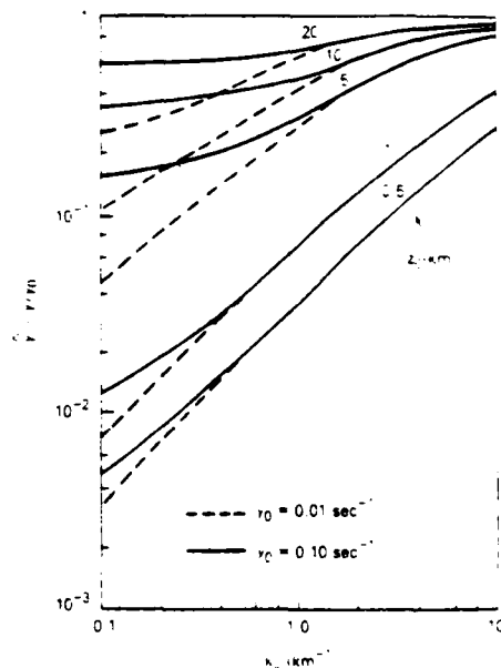
Fig. 7. Plot of perpendicular wave number k_{\perp} (km ^{-1} ) versus growth rate \gamma (s ^{-1} ) for \nu_0 = 0.10 \text{ s}^{-1} (solid curves), \nu_0 = 0.01 \text{ s}^{-1} (dashed curves), and several values of z_0 (km). Curve is based upon (27) for m = 0 . The ionospheric parameters used are given in the text (section 4).
