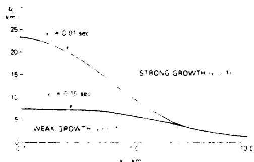
Fig. 6. Plot of "critical" parallel length z_0 (km) versus perpendicular wave number k_{\perp} (km ^{-1} ) based upon (44) for typical ionospheric parameters. The parameters used are given in the text (section 4). These curves denote the boundary between region II (above curves—strong growth ( \gamma > 1 )) and region III (below curves—weak growth ( \gamma < 1 )).
