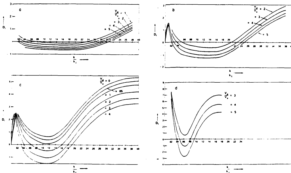
FIG. 4. A plot of imaginary part of the local dispersion relation D_i(\omega, k) vs k/k_i reproduced from Ref. 2 for various V_{\alpha}/V_e . Here b = 0.5 , \mu = 3 \times 10^{-4} and four different values of the temperature ratio \tau are: (a) \tau = 0.1 , (b) \tau = 0.2 , (c) \tau = 0.33 , and (d) \tau = 1.0 .
