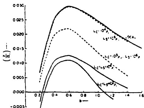
Fig. 2. A plot similar to Figure 1. Here V_g/v_e = 0.28 and equation (4) has been solved. This figure shows how finite current width L_c modifies the results of figure 1.
