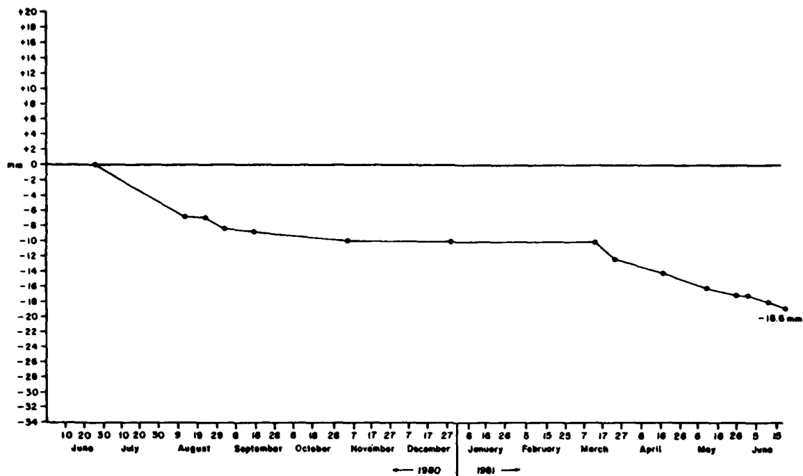
Figure A4.8 Cumulative Average Erosion at Overland Erosion Station #8 Orwell Lake, Minnesota (1980-1981)
