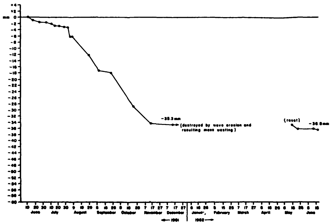
Figure A5.13 Cumulative Average Erosion at Overland Erosion Station #11 Orwell Lake, Minnesota (1961 - 1962)
