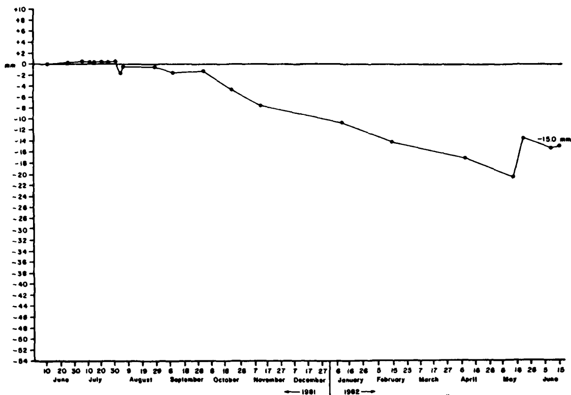
Figure A3.12 Cumulative Net Changes at Overland Erosion Station #10 Orwell Lake, Minnesota (1981 - 1982)
