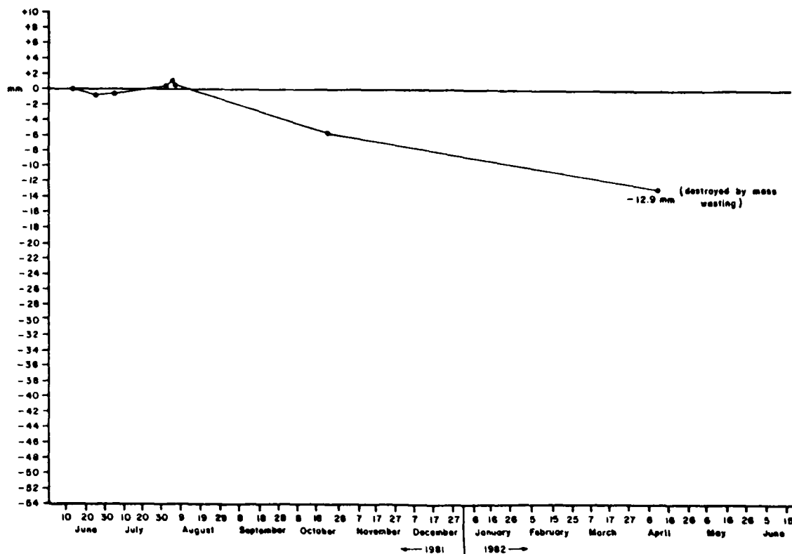
Figure A3.8 Cumulative Net Changes at Overland Erosion Station # 7 A Orwell Lake, Minnesota (1981 - 1982)
