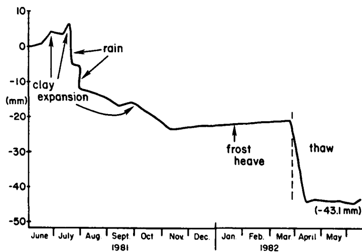
Figure 19. Cumulative net change, erosion station 1, 1981-1982.
