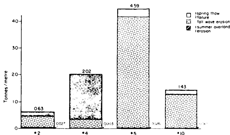
Figure 54. Total bank erosion at four erosion stations, 1981-82.
