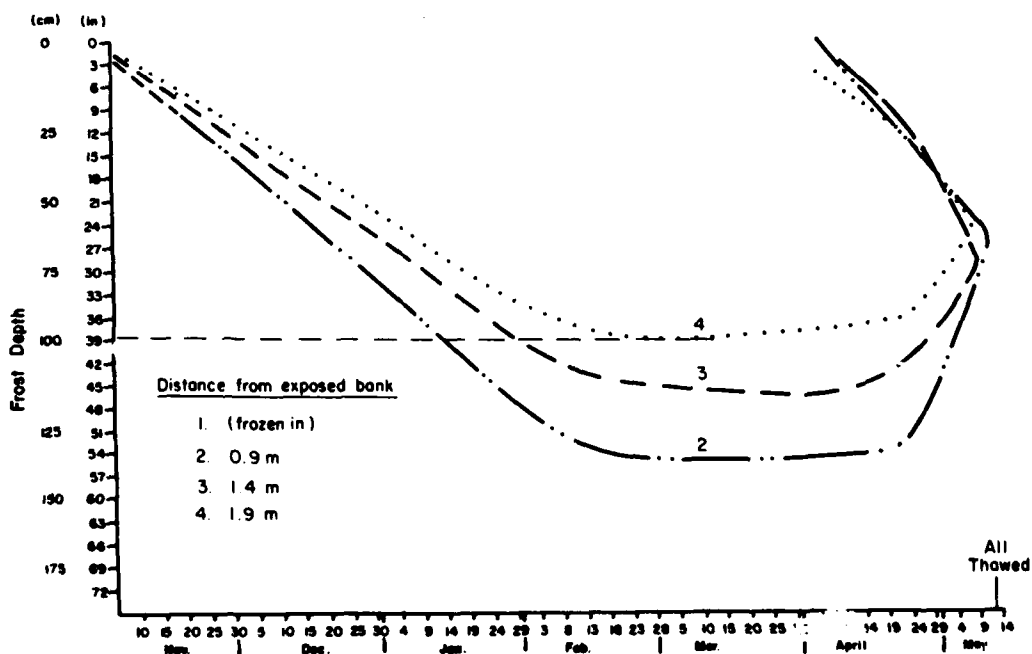
Figure 37. Penetration of frost (winter 1982-83), tubes 2-4.
