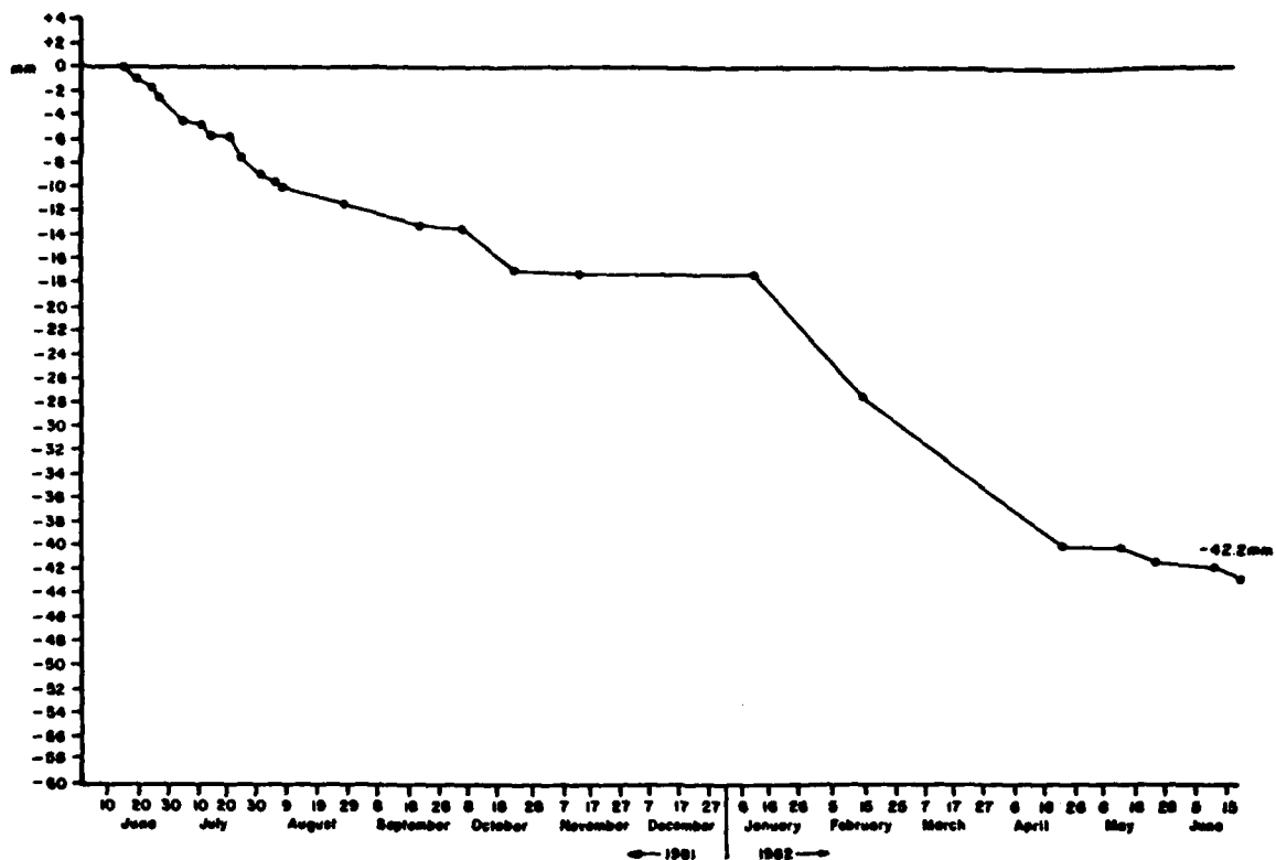
Figure A5.10 Cumulative Average Erosion at Overland Erosion Station #8 Orwell Lake, Minnesota (1981 - 1982)
