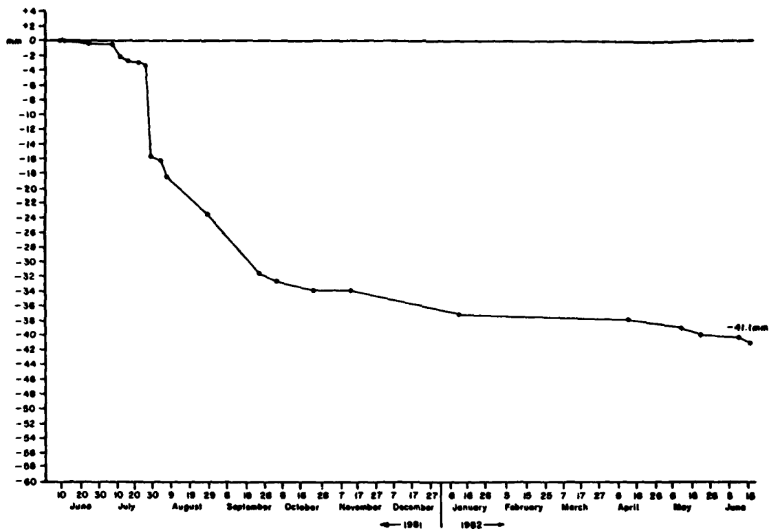
Figure A5.6 Cumulative Average Erosion at Overland Erosion Station #6 Orwell Lake, Minnesota (1981 - 1982)
