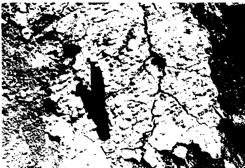
Figure 51. Stripwash caused by wind-directed rainsplash and overland flow at east end of Orwell Lake, June 1980.
