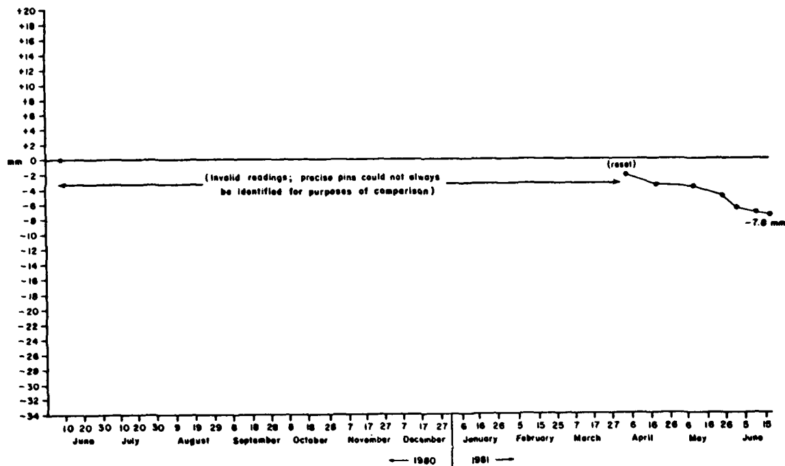
Figure A4.1 Cumulative Average Erosion at Overland Erosion Station #1 Orwell Lake, Minnesota (1980-1981)
