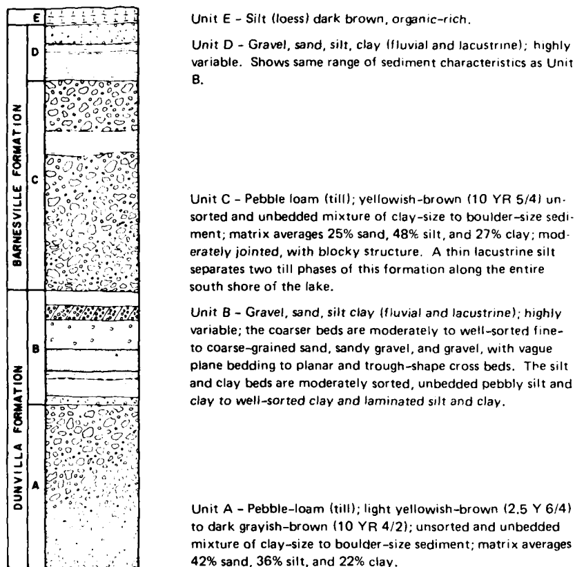
Figure 15. Composite geologic column of the banks of Orwell Lake, Minnesota. (For scale, unit B averages about 1 m thick.)
