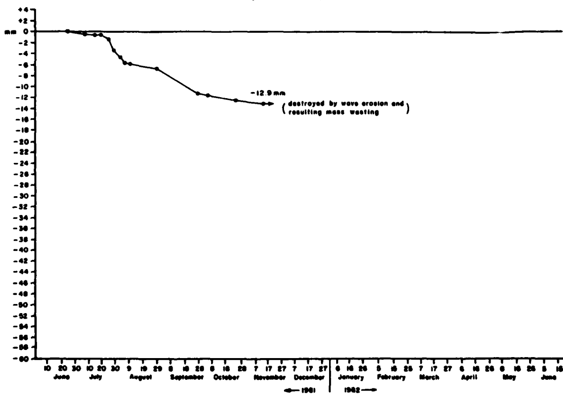
Figure A5.9 Cumulative Average Erosion at Overland Erosion Station #8A Orwell Lake, Minnesota (1981 - 1982)
