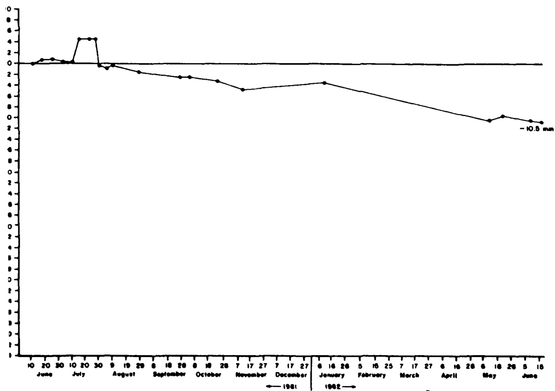
Figure A3.7 Cumulative Net Changes at Overland Erosion Station # 7 Orwell Lake, Minnesota (1981 - 1982)
