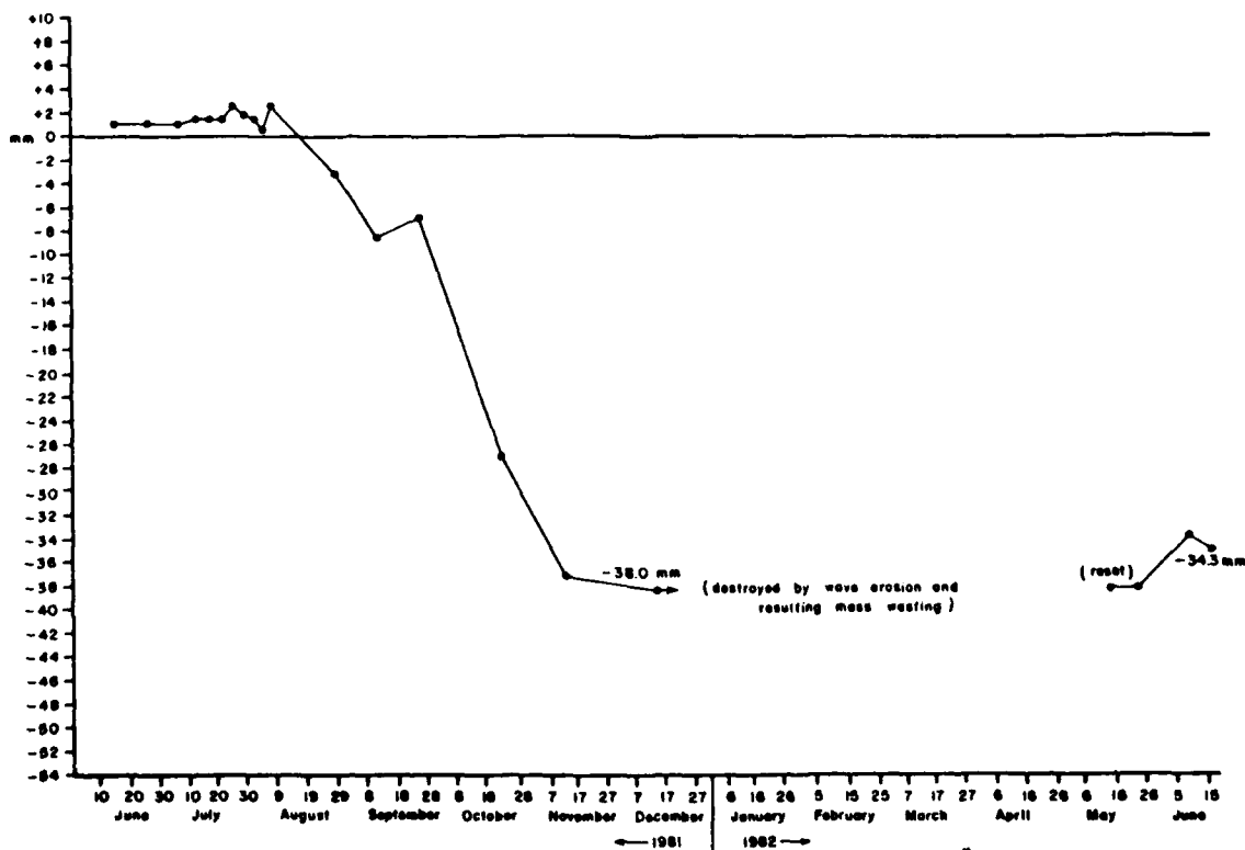
Figure A3.13 Cumulative Net Changes at Overland Erosion Station #11 Orwell Lake, Minnesota (1981 - 1982)
