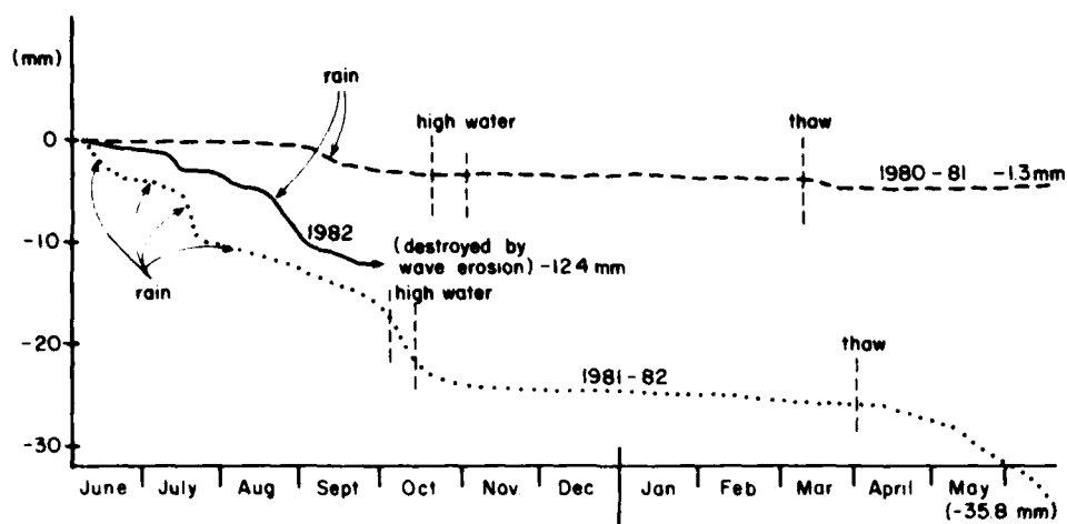
Figure 23. Cumulative average erosion, erosion station 12, 1980-1982.
