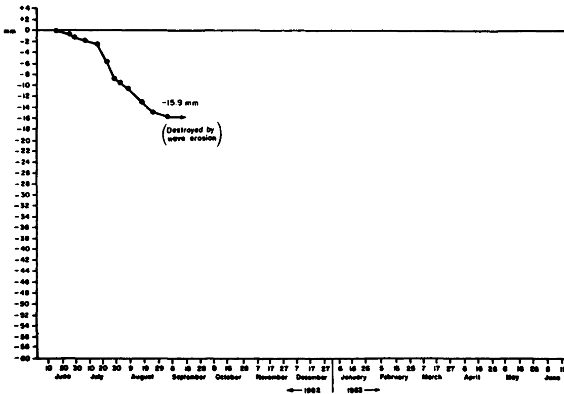
Figure A6.9 Cumulative Average Erosion at Overland Erosion Station #9 Orwell Lake, Minnesota (1982)
