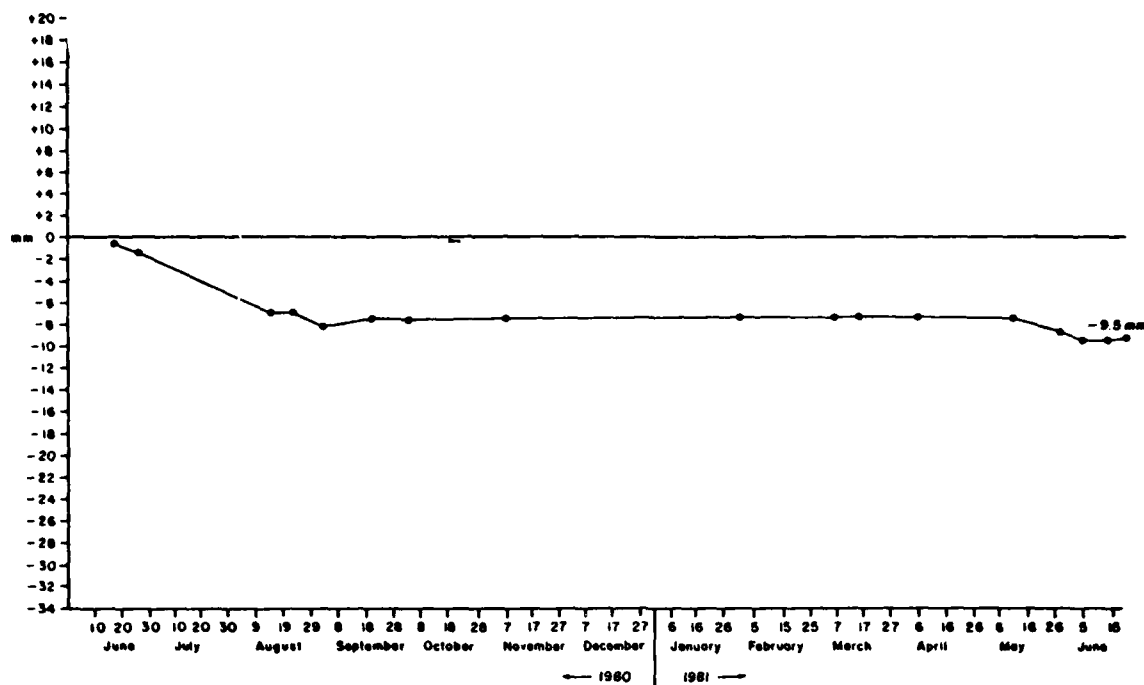
Figure A2.10 Cumulative Net Changes at Overland Erosion Station #10 Orwell Lake, Minnesota (1980-1981)
