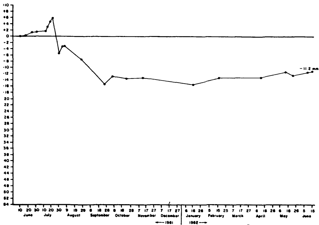
Figure A3.6 Cumulative Net Changes at Overland Erosion Station # 6 Orwell Lake, Minnesota (1981 - 1982)
