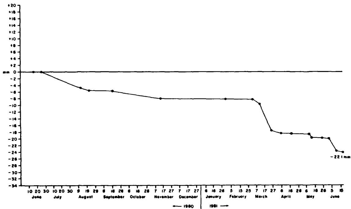
Figure A4.5 Cumulative Average Erosion at Overland Erosion Station #5 Orwell Lake, Minnesota (1980-1981)
