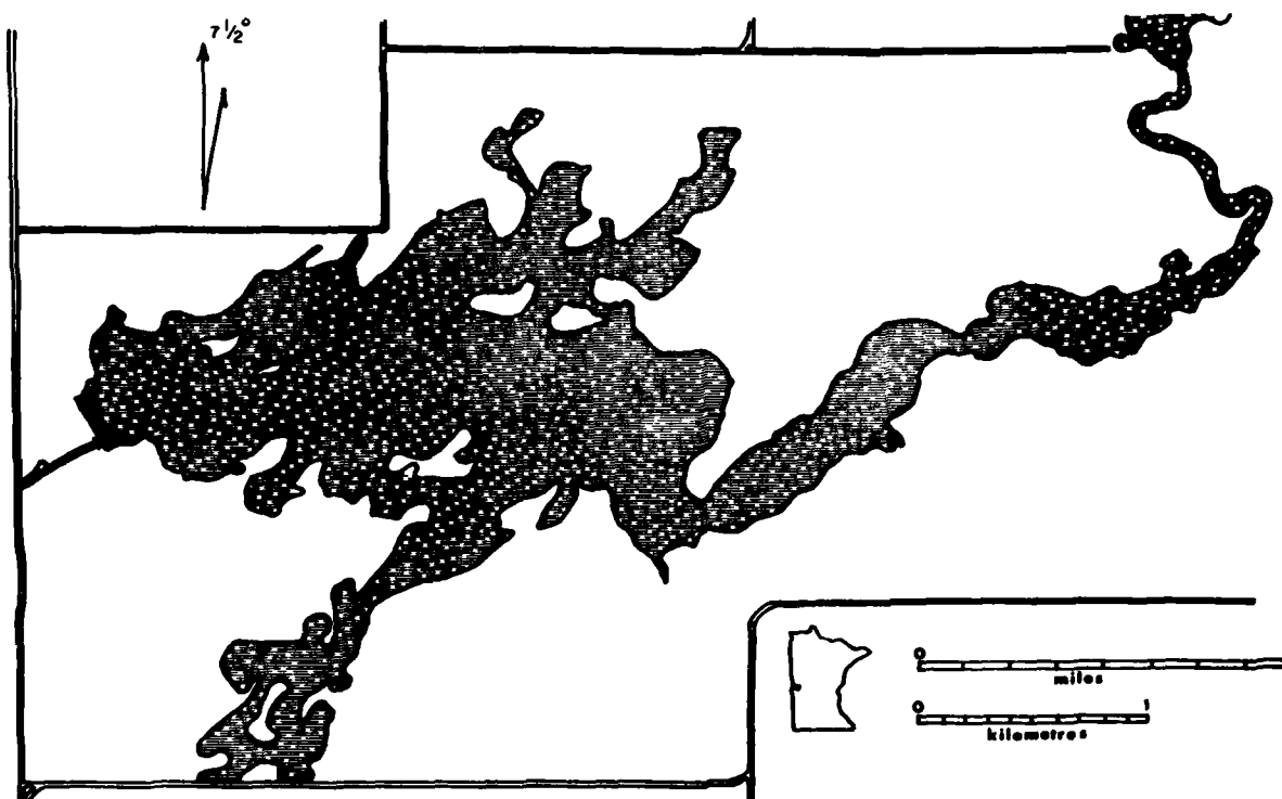
Figure 3. Orwell Lake, Minnesota, 326-m level.
