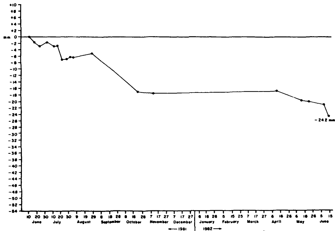
Figure A3.14 Cumulative Net Changes at Overland Erosion Station #12 Orwell Lake, Minnesota (1981 - 1982)
