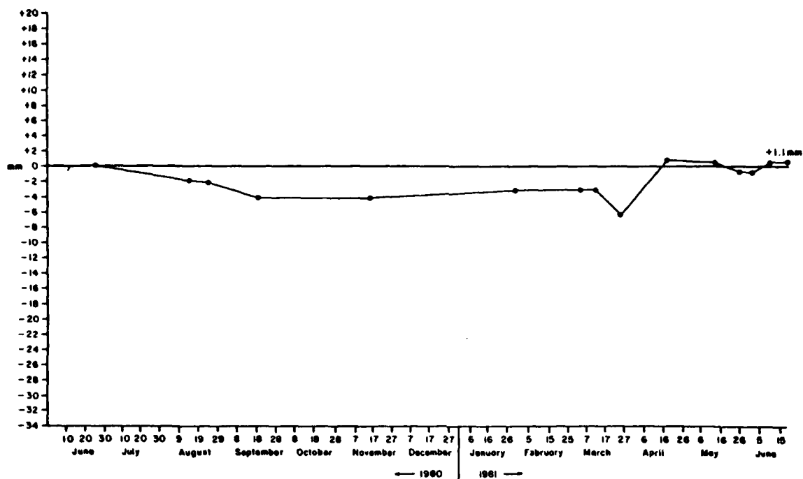
Figure A2.6 Cumulative Net Changes at Overland Erosion Station #6 Orwell Lake, Minnesota (1980-1981)
