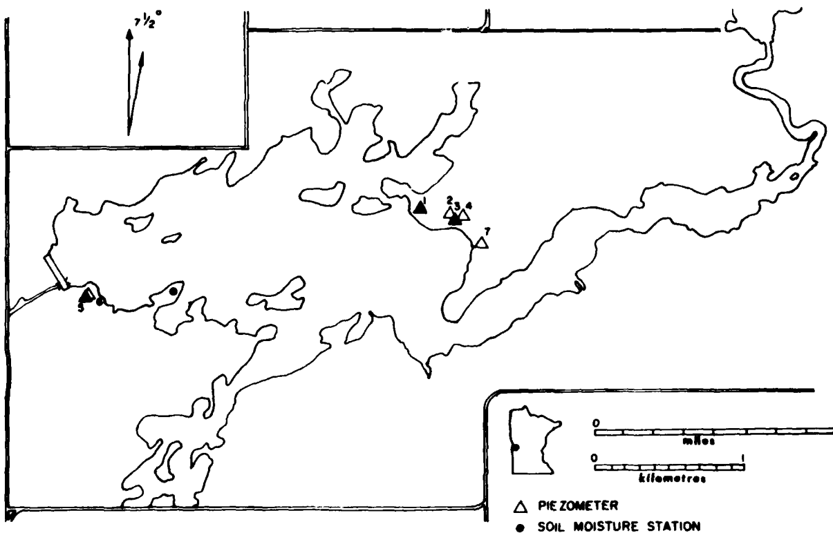
Figure 12. Location of piezometer and soil moisture stations.
