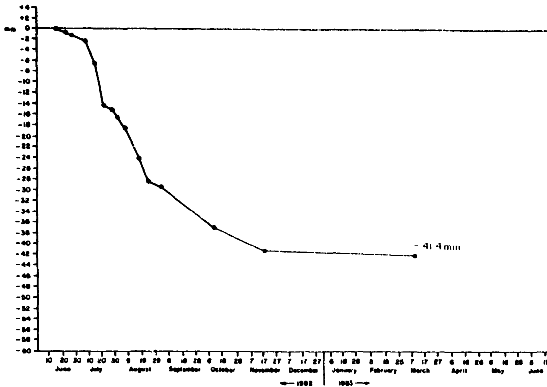
Figure A6.4 Cumulative Average Erosion at Overland Erosion Station # 4 Orwell Lake, Minnesota (1982 - 1983)
