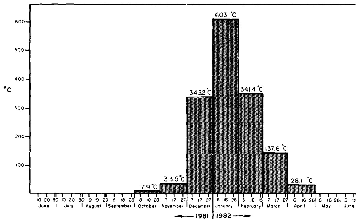
Figure 31. Accumulated average degrees below freezing, winter 1981-82.
