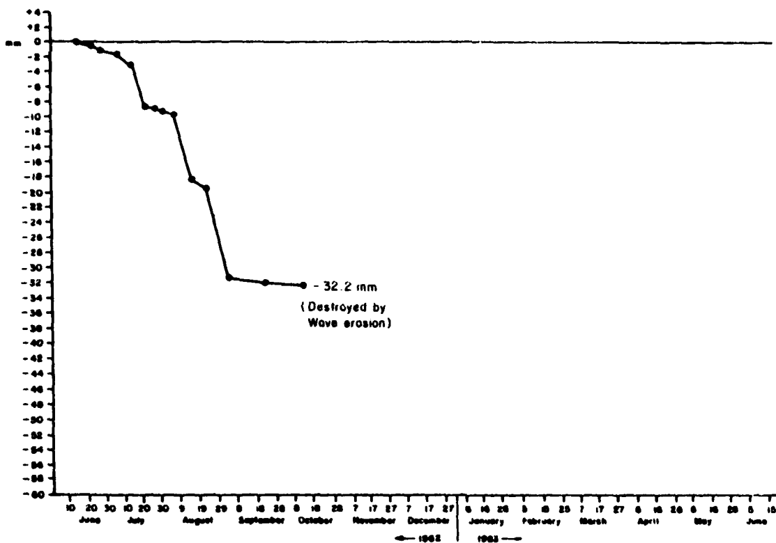
Figure A6.11 Cumulative Average Erosion at Overland Erosion Station #11 Orwell Lake, Minnesota (1982)
