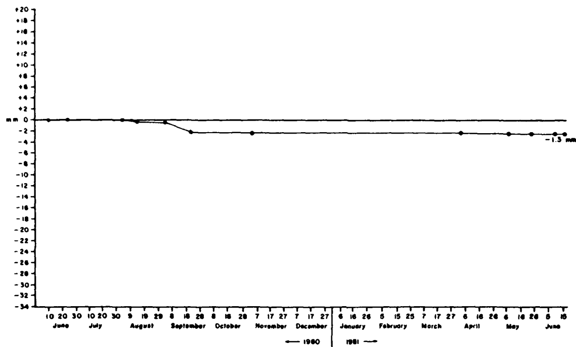
Figure A4.12 Cumulative Average Erosion at Overland Erosion Station # 12 Orwell Lake, Minnesota (1980-1981)
