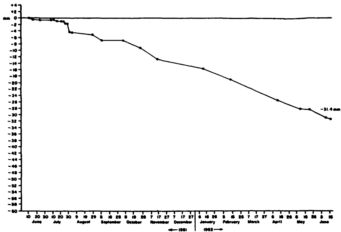
Figure A5.12 Cumulative Average Erosion at Overland Erosion Station #10 Orwell Lake, Minnesota (1961 - 1962)
