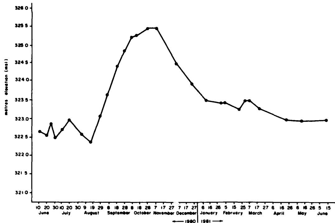
Figure 25. Orwell Lake pool levels 1980-1981.
