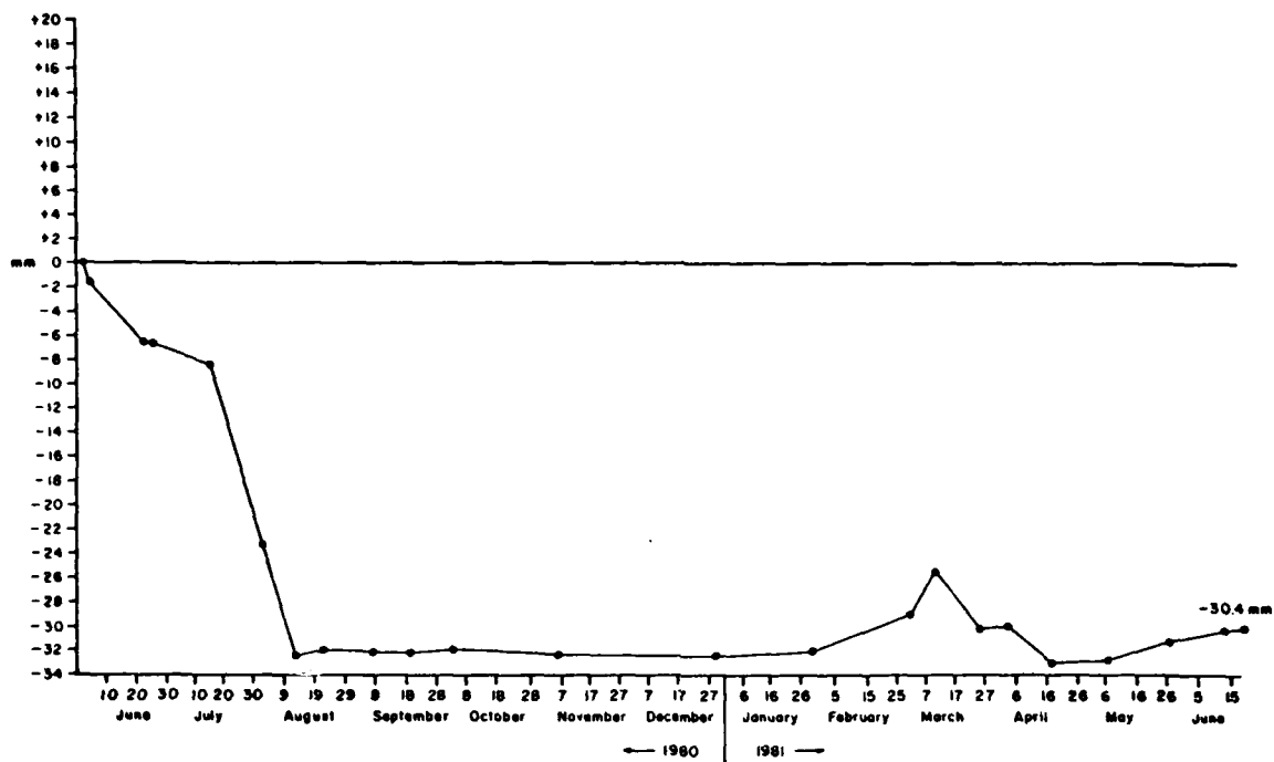
Figure A2.2 Cumulative Net Changes at Overland Erosion Station #2 Orwell Lake, Minnesota (1980-1981)
