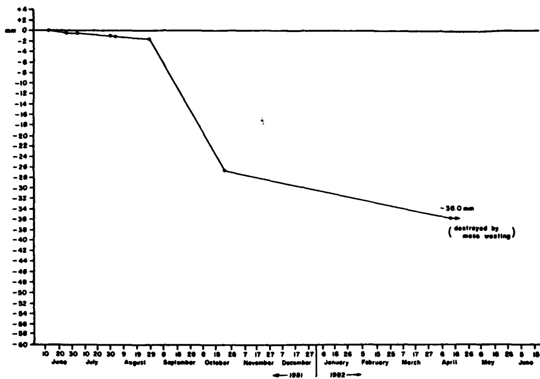
Figure A5.8 Cumulative Average Erosion at Overland Erosion Station #7A Orwell Lake, Minnesota (1981 - 1982)
