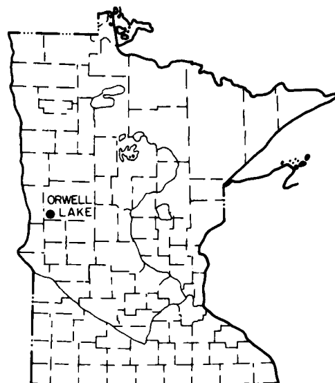
Figure 1. Location of Orwell Lake, Minnesota.
