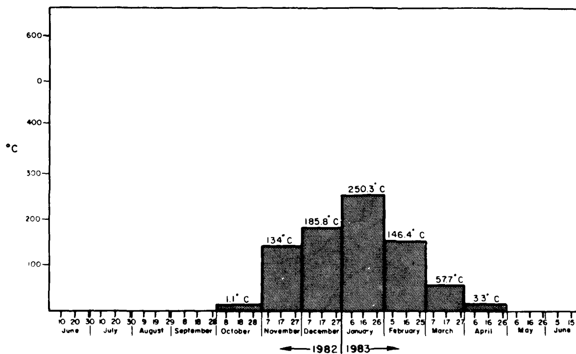
Figure 32. Accumulated average degrees below freezing, winter 1982-83.
