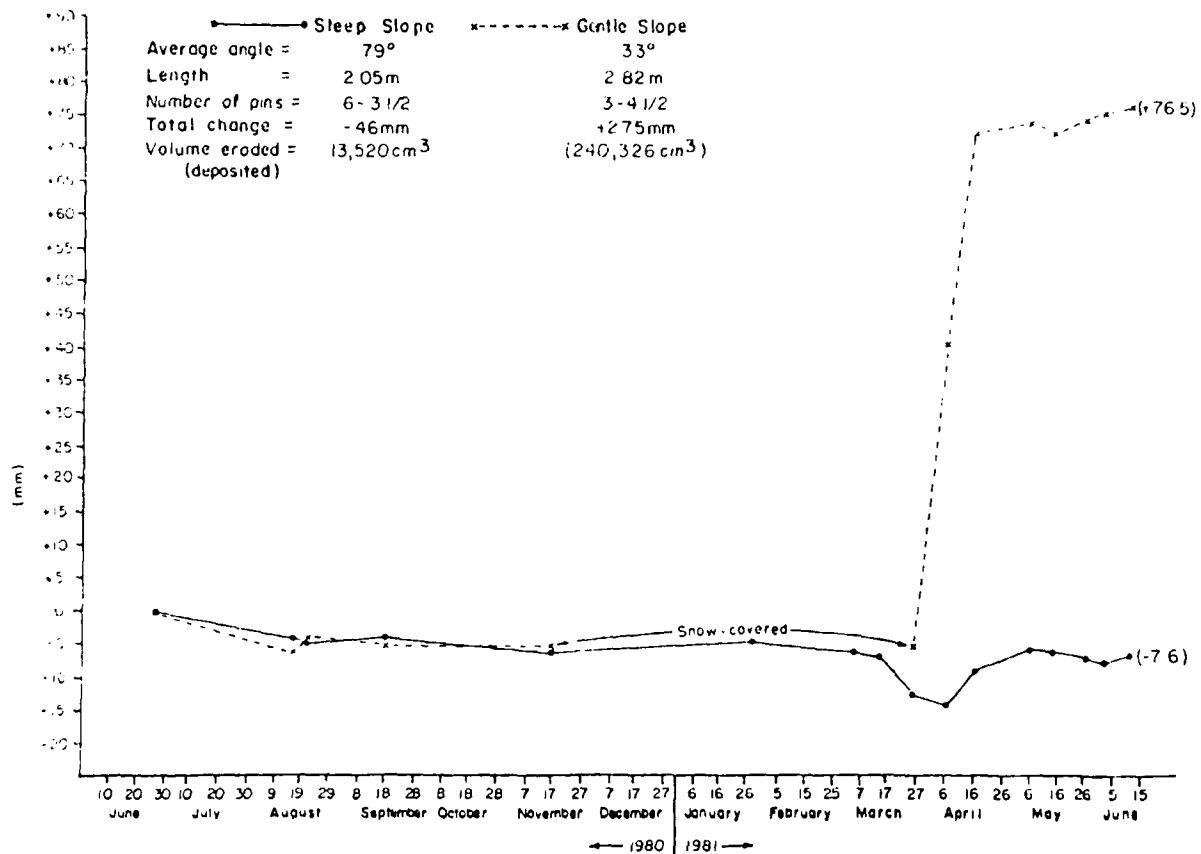
Figure A1.4 Average Cumulative Change of Surface at Erosion Station # 5, 1980-1981, Orwell Lake, Minnesota
