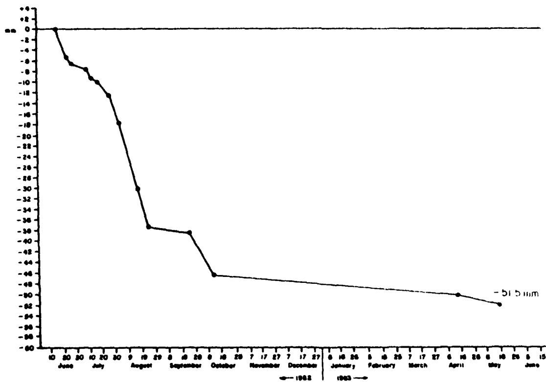
Figure A6.7 Cumulative Average Erosion at Overland Erosion Station #7 Orwell Lake, Minnesota (1982-1983)
