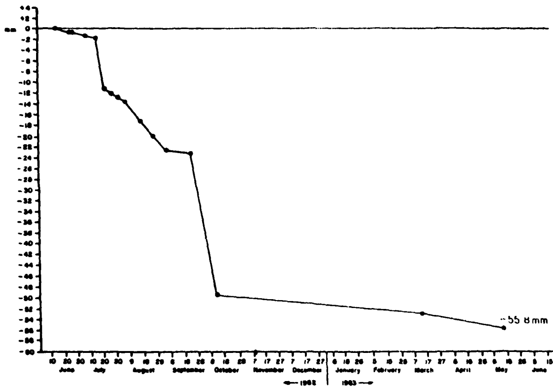
Figure A6.3 Cumulative Average Erosion at Overland Erosion Station #3 Orwell Lake, Minnesota (1982-1983)
