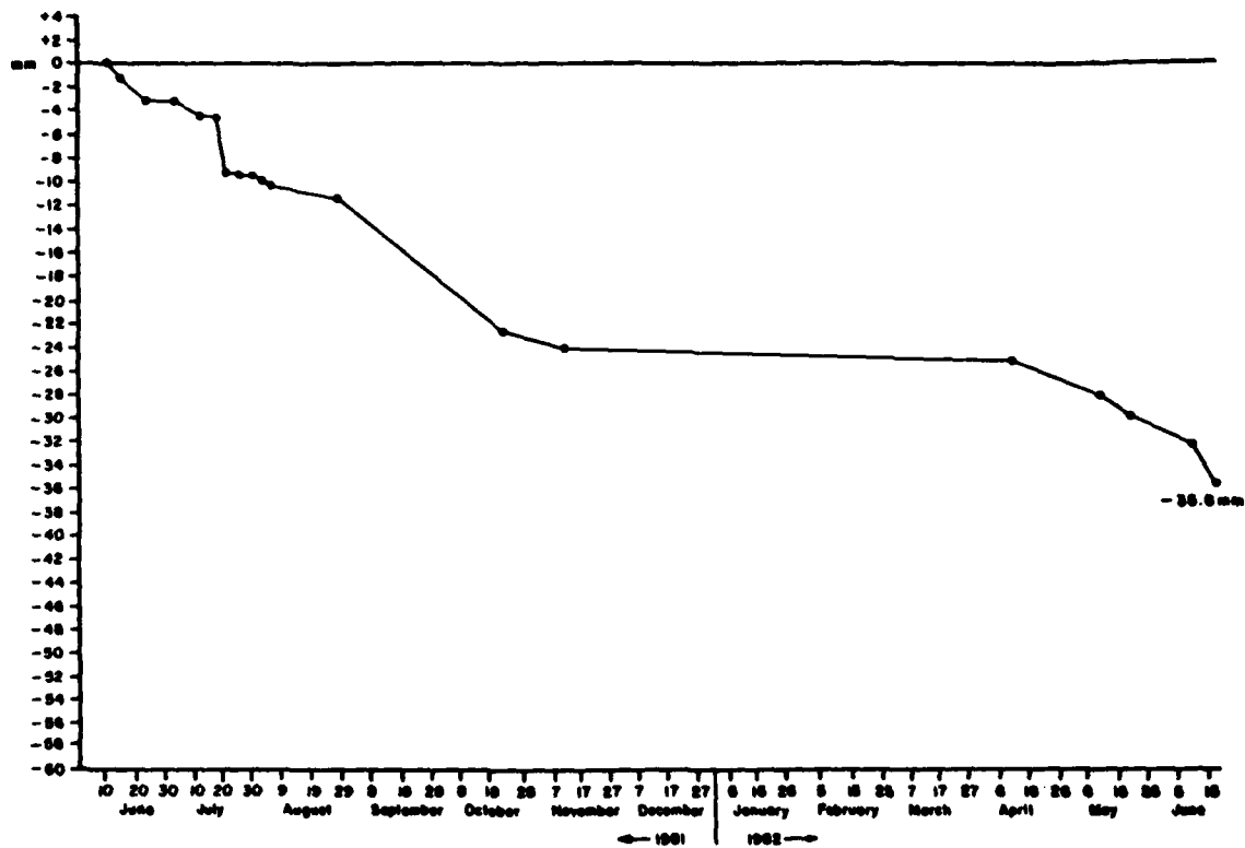
Figure A5.14 Cumulative Average Erosion at Overland Erosion Station #12 Orwell Lake, Minnesota (1961 - 1962)
