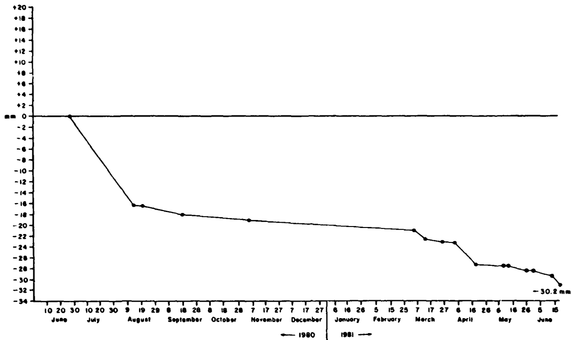
Figure A4.4 Cumulative Average Erosion at Overland Erosion Station #4 Orwell Lake, Minnesota (1980-1981)
