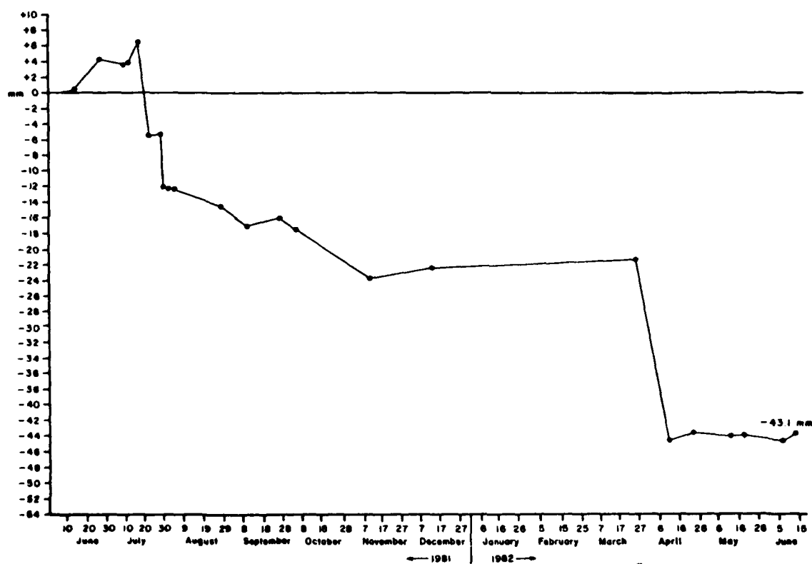
Figure A3.1 Cumulative Net Changes at Overland Erosion Station #1 Orwell Lake, Minnesota (1981 - 1982)
