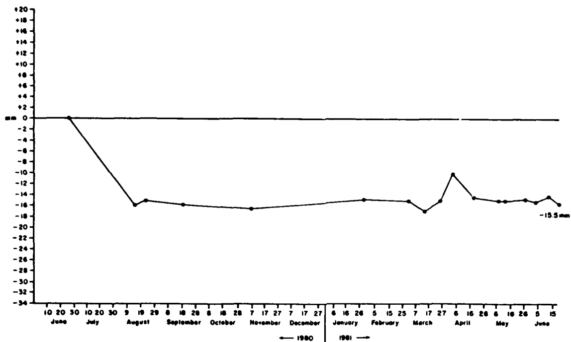
Figure A2.4 Cumulative Net Changes at Overland Erosion Station #4 Orwell Lake, Minnesota (1980-1981)
