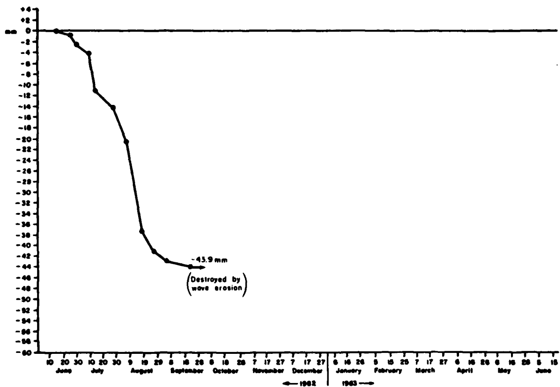
Figure A6.1 Cumulative Average Erosion at Overland Erosion Station #1 Orwell Lake, Minnesota (1982)
