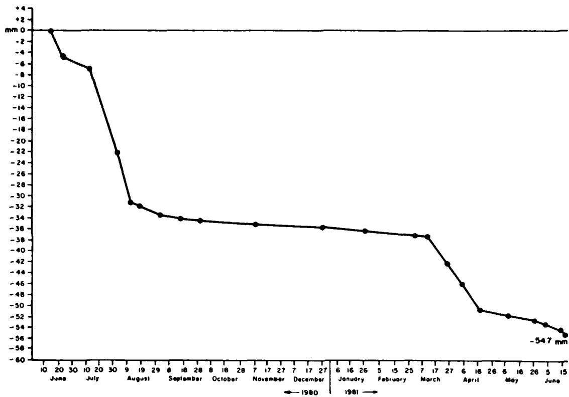
Figure A4.2 Cumulative Average Erosion at Overland Erosion Station #2 Orwell Lake, Minnesota (1980 - 1981)
