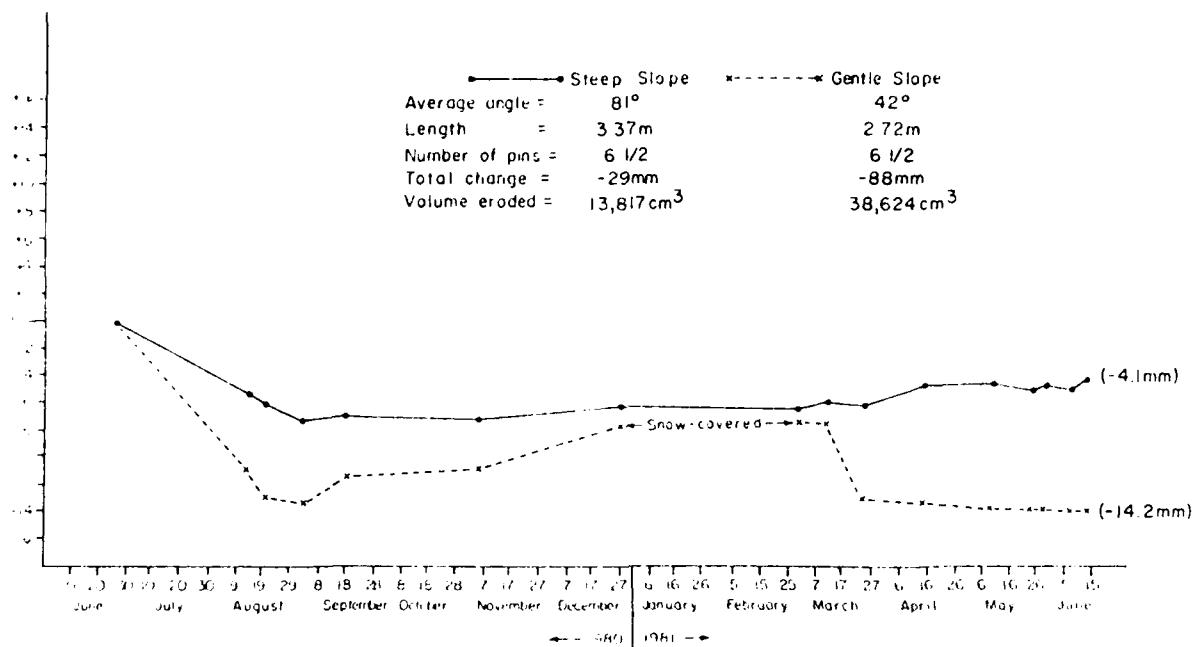
Figure A1.6 Average Cumulative Change of Surface at Erosion Station # 7 , 1980-1981. Orwell Lake, Minnesota
