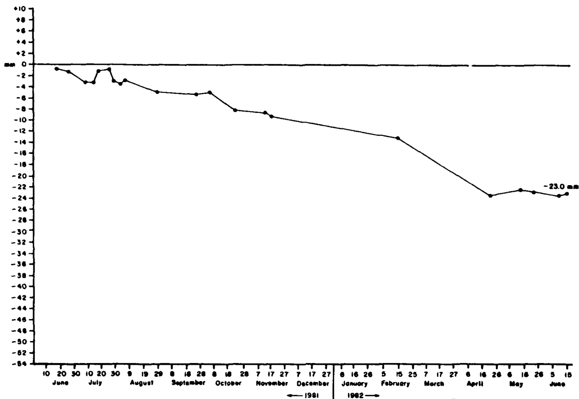
Figure A3.10 Cumulative Net Changes at Overland Erosion Station # 8 Orwell Lake, Minnesota (1981 - 1982)
