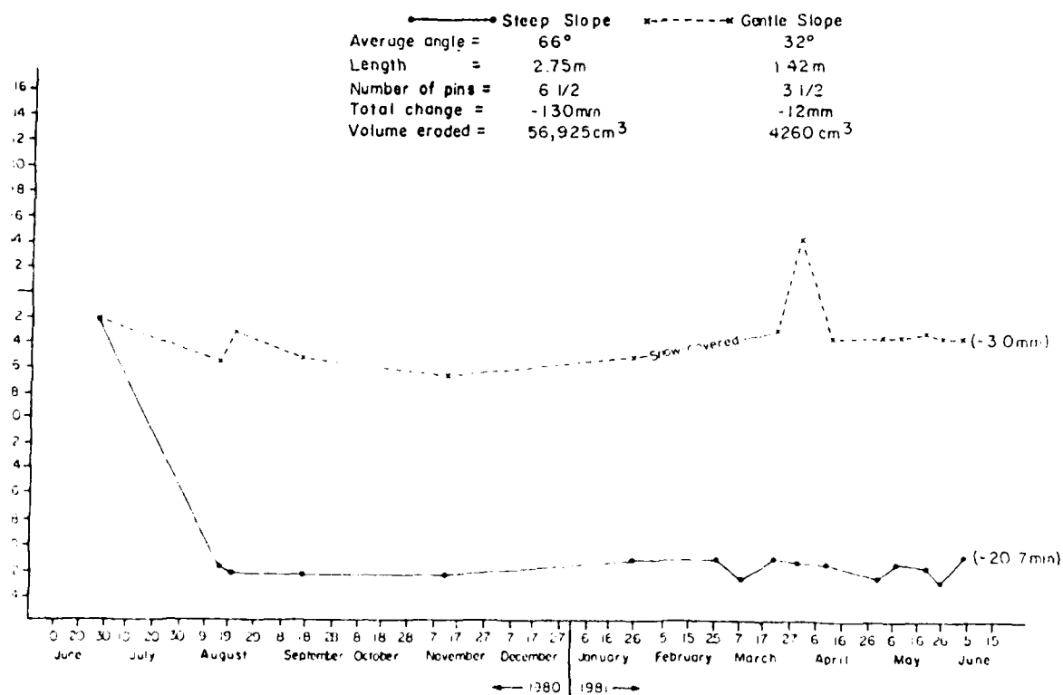
Figure A1.3 Average Cumulative Change of Surface at Erosion Station # 4, 1980-1981. Orwell Lake, Minnesota
