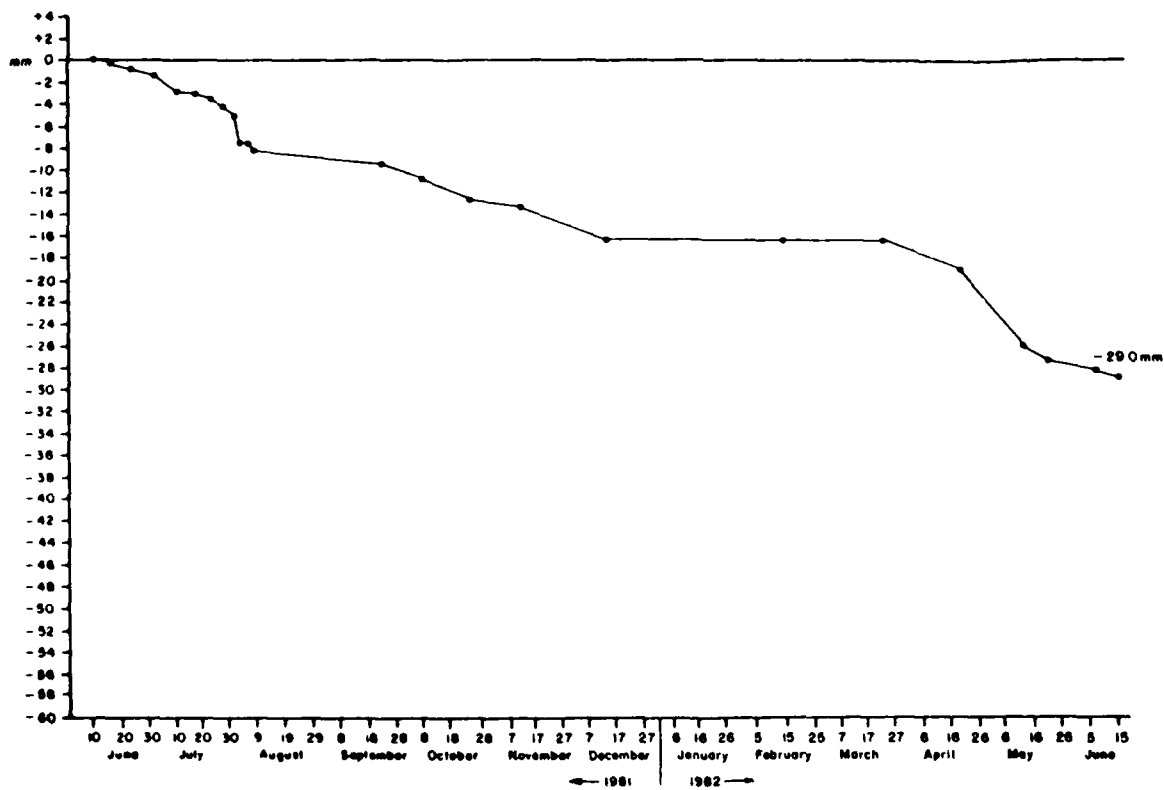
Figure A5.3 Cumulative Average Erosion at Overland Erosion Station #3 Orwell Lake, Minnesota (1981 - 1982)
