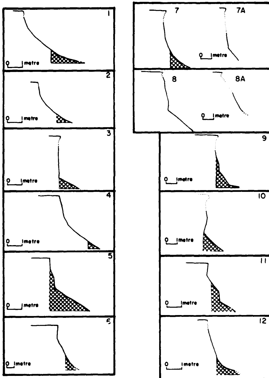
Figure 27. Profiles of Orwell Lake banks at overland erosion station sites before and after wave modification in October 1981. The patterned area was removed by lake erosion. (See Fig. 6 for location of stations.)
