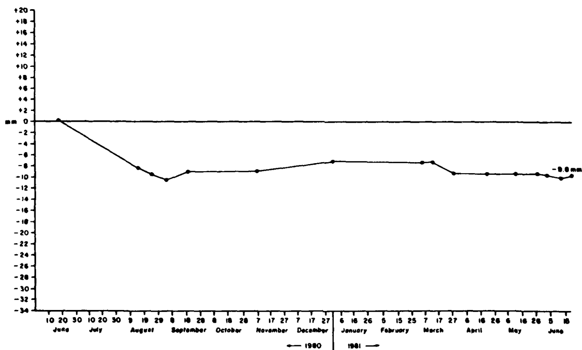
Figure A2.7 Cumulative Net Changes at Overland Erosion Station #7 Orwell Lake, Minnesota (1980-1981)
