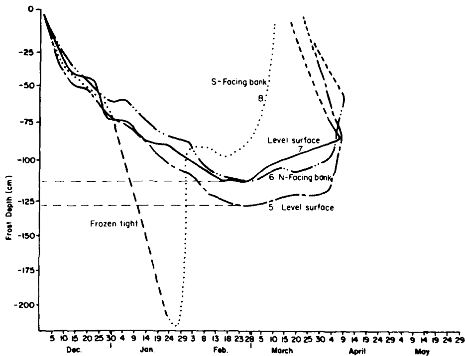
Figure 34. Penetration of frost (winter 1980-81), tubes 5-8.
