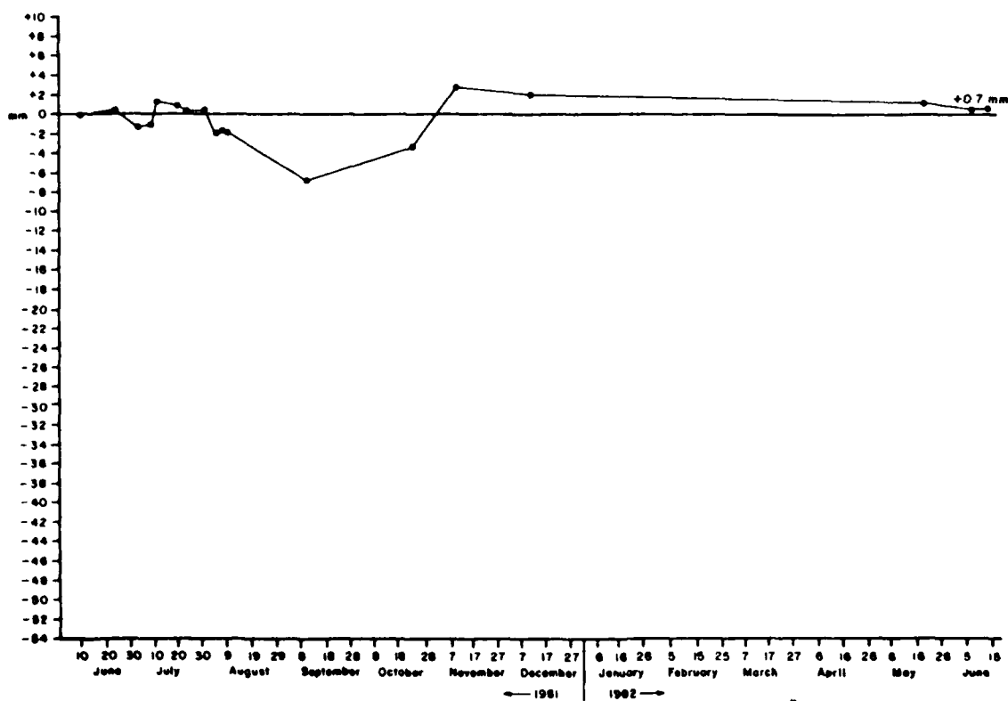
Figure A3.5 Cumulative Net Changes at Overland Erosion Station # 5 Orwell Lake, Minnesota (1981 - 1982)
