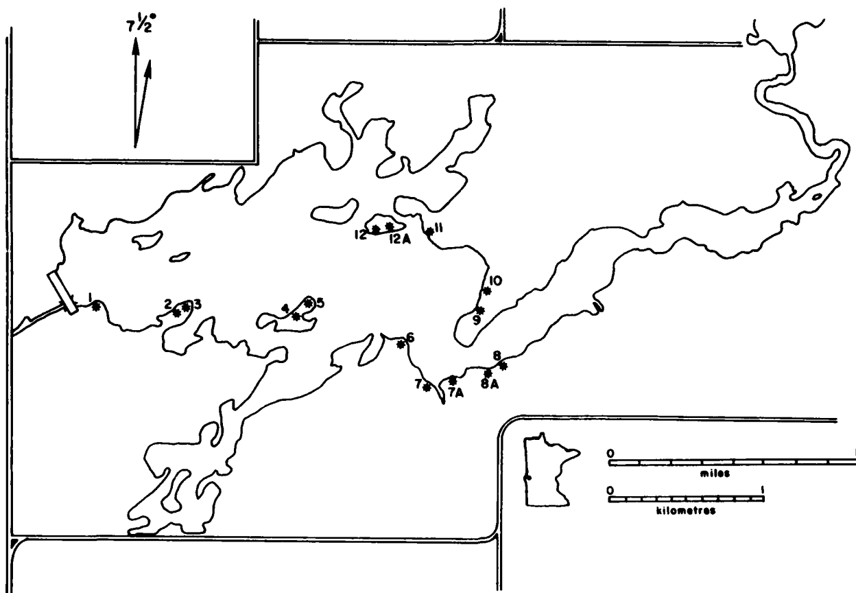
Figure 6. Orwell Lake, Minnesota with locations of erosion stations.
