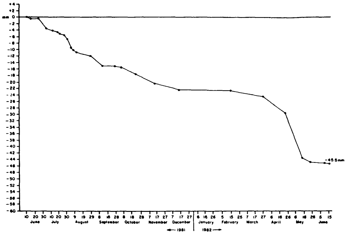
Figure A5.2 Cumulative Average Erosion at Overland Erosion Station #2 Orwell Lake, Minnesota (1981 - 1982)
