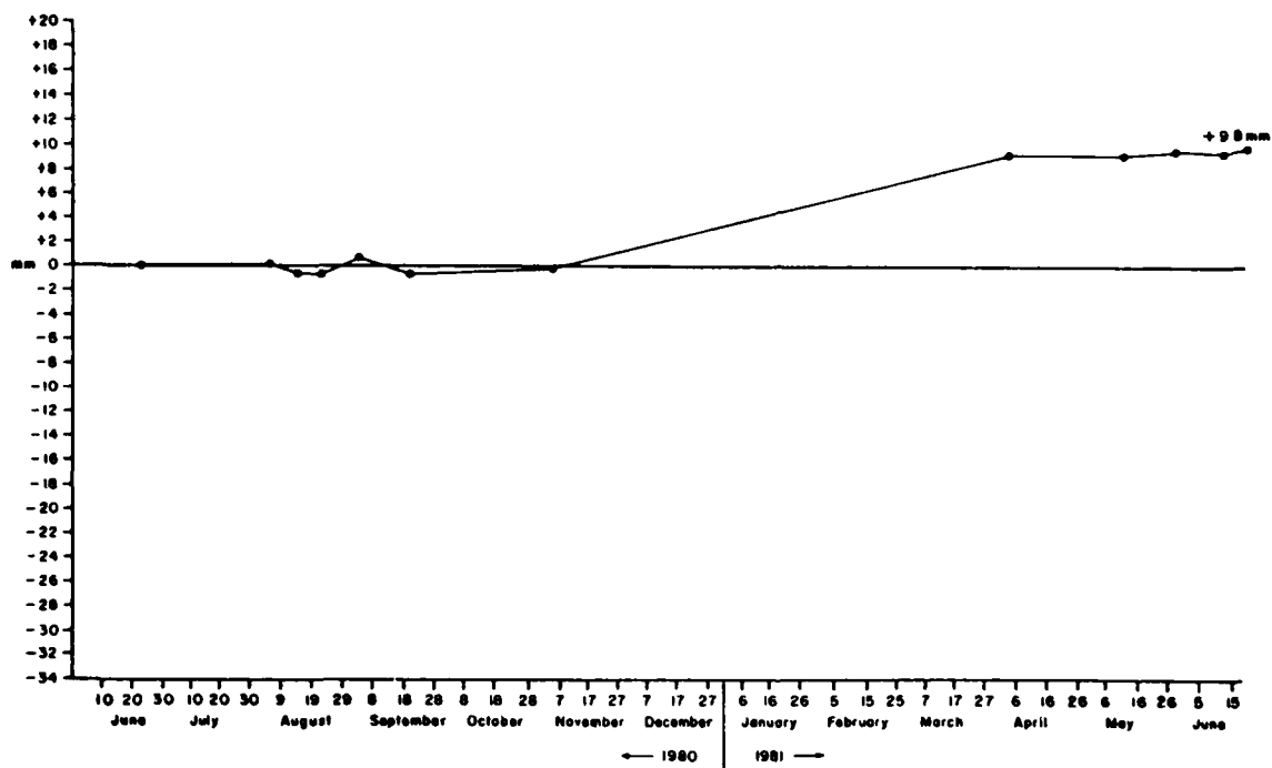
Figure A2.12 Cumulative Net Changes at Overland Erosion Station #12 Orwell Lake, Minnesota (1980 - 1981)
