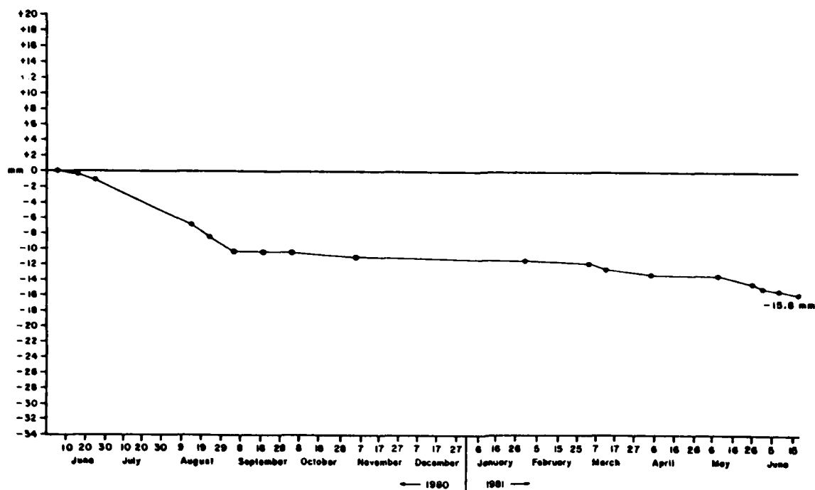
Figure A4.10 Cumulative Average Erosion at Overland Erosion Station #10 Orwell Lake, Minnesota (1980-1981)
