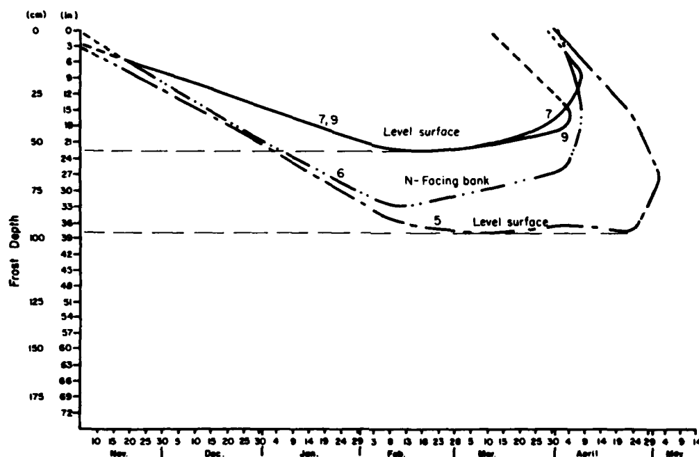
Figure 38. Penetration of frost (winter 1982-83), tubes 5-9.
