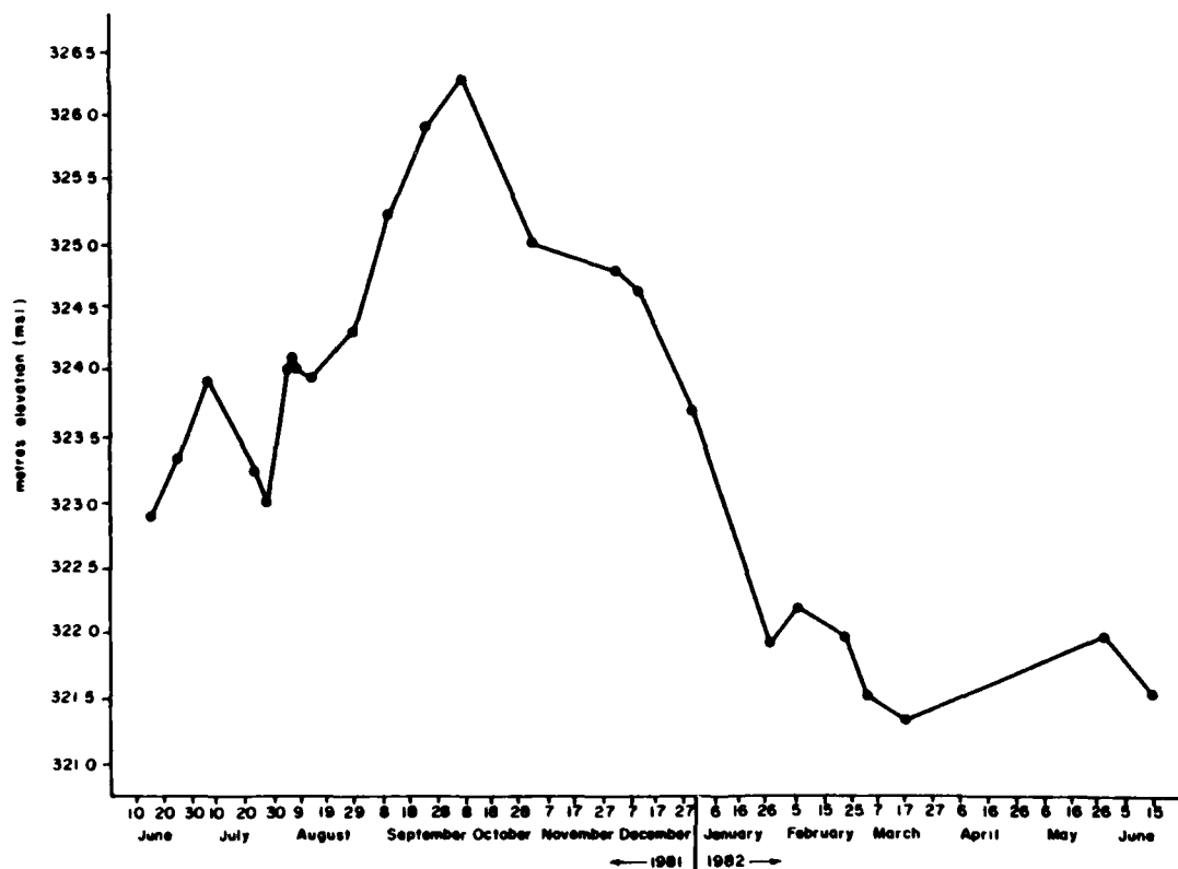
Figure 26. Orwell Lake pool levels 1981-1982.
