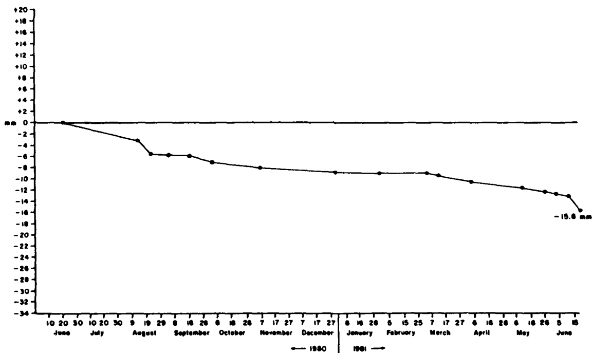
Figure A4.9 Cumulative Average Erosion at Overland Erosion Station #9 Orwell Lake, Minnesota (1980-1981)
