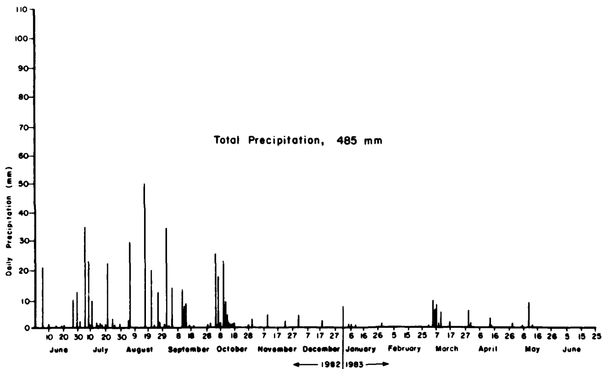
Figure 49. Daily precipitation, Orwell Lake, 1982-1983.
