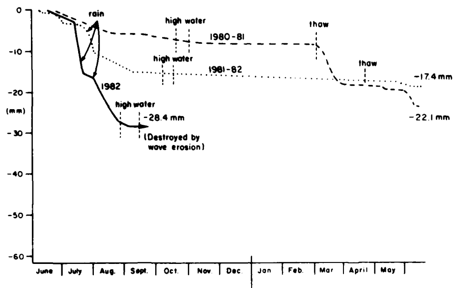
Figure 21. Cumulative average erosion at overland erosion station 5, 1980-1982.
