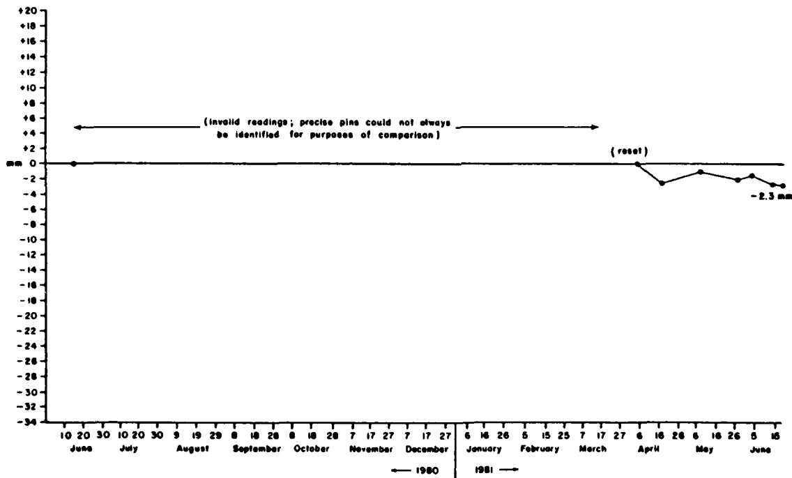
Figure A2.1 Cumulative Net Changes at Overland Erosion Station #1 Orwell Lake, Minnesota (1980-1981)
