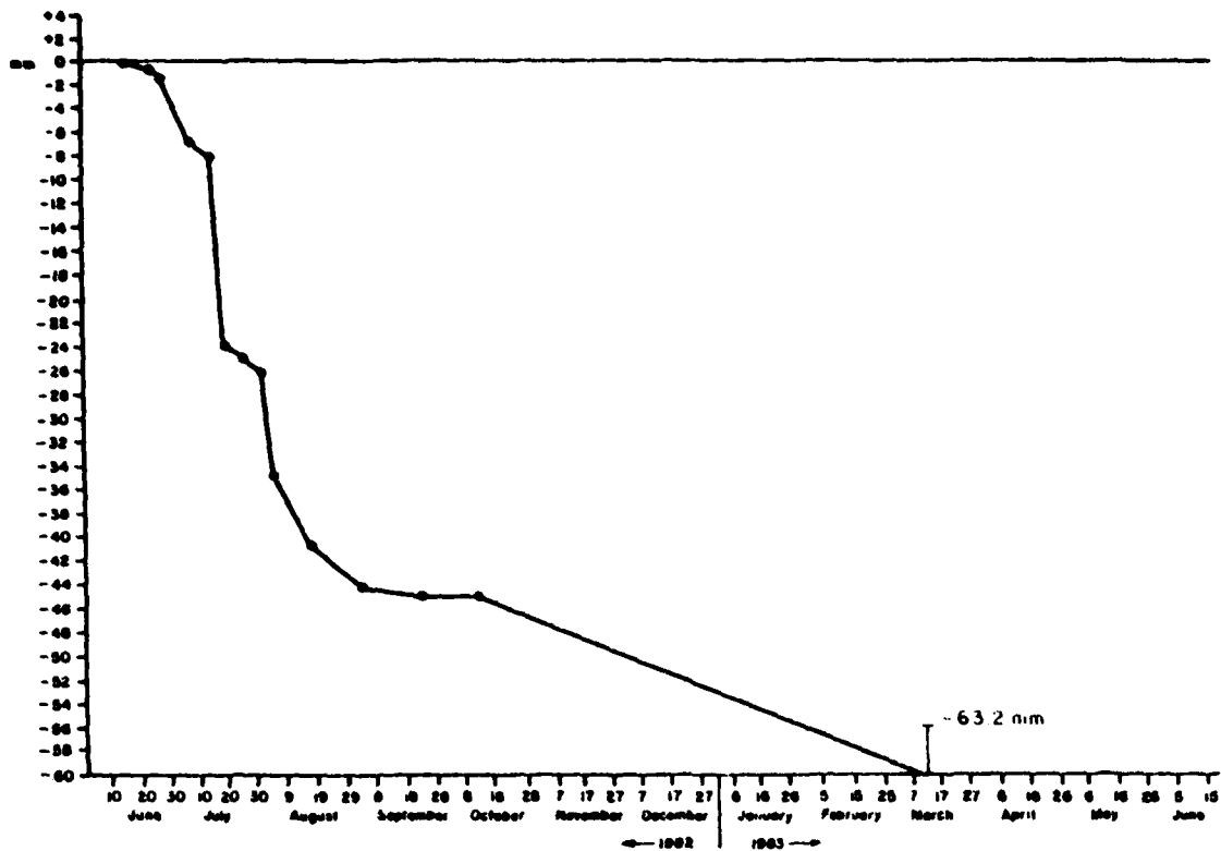
Figure A6.2 Cumulative Average Erosion at Overland Erosion Station #2 Orwell Lake, Minnesota (1982-1983)
