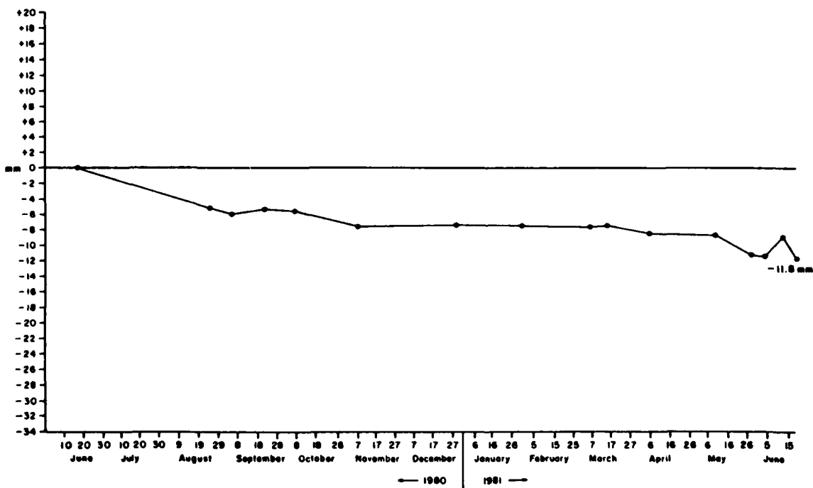
Figure A2.9 Cumulative Net Changes at Overland Erosion Station #9 Orwell Lake, Minnesota (1980-1981)
