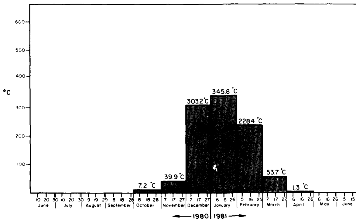
Figure 30. Accumulated average degrees below freezing, winter 1980-81.
