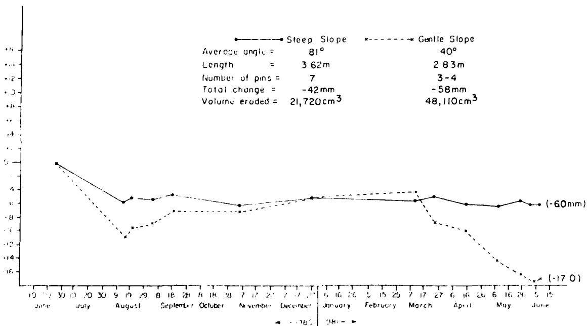
Figure A1.7 Average Cumulative Change of Surface at Erosion Station # 8 , 1980-1981. Orwell Lake, Minnesota
