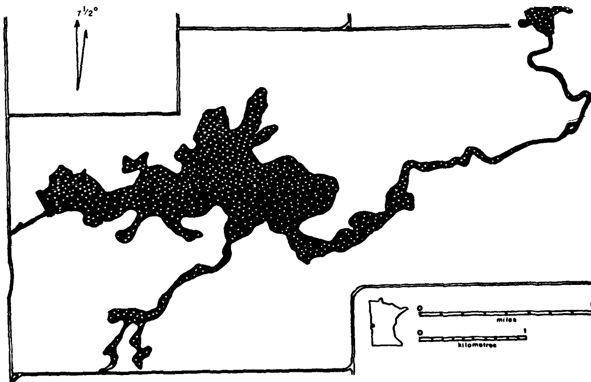
Figure 2. Orwell Lake, Minnesota, 323-m level.
