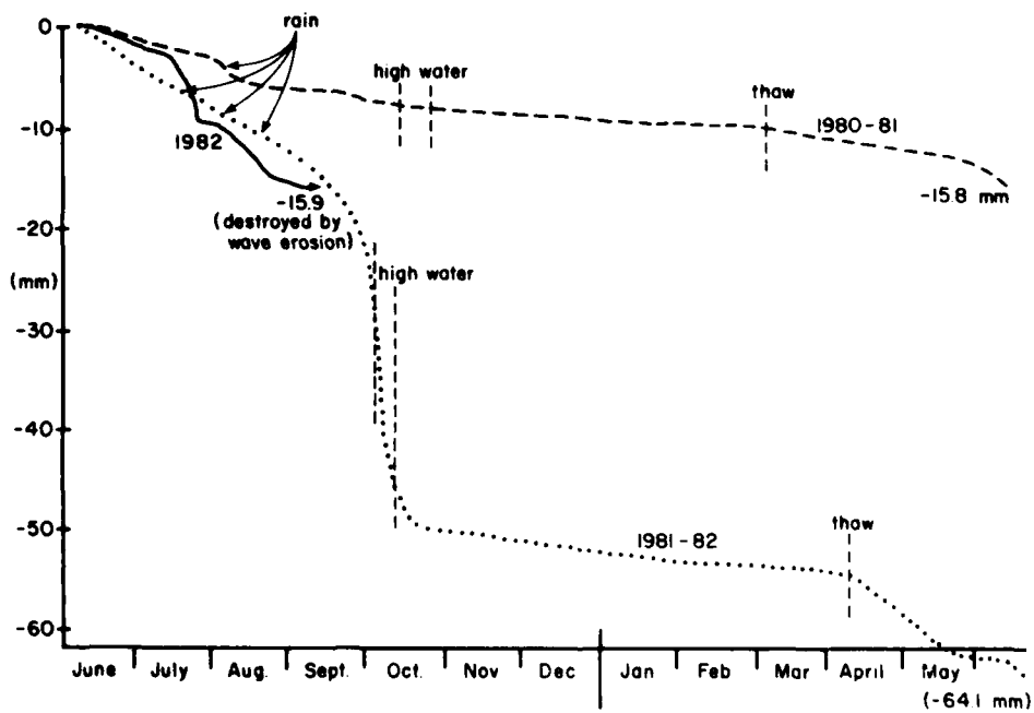
Figure 22. Cumulative average erosion, erosion station 9, 1980-1982.
