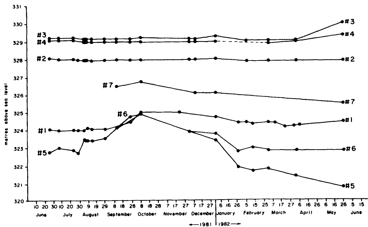
Figure 45. Piezometric head fluctuations, 1981-82.
