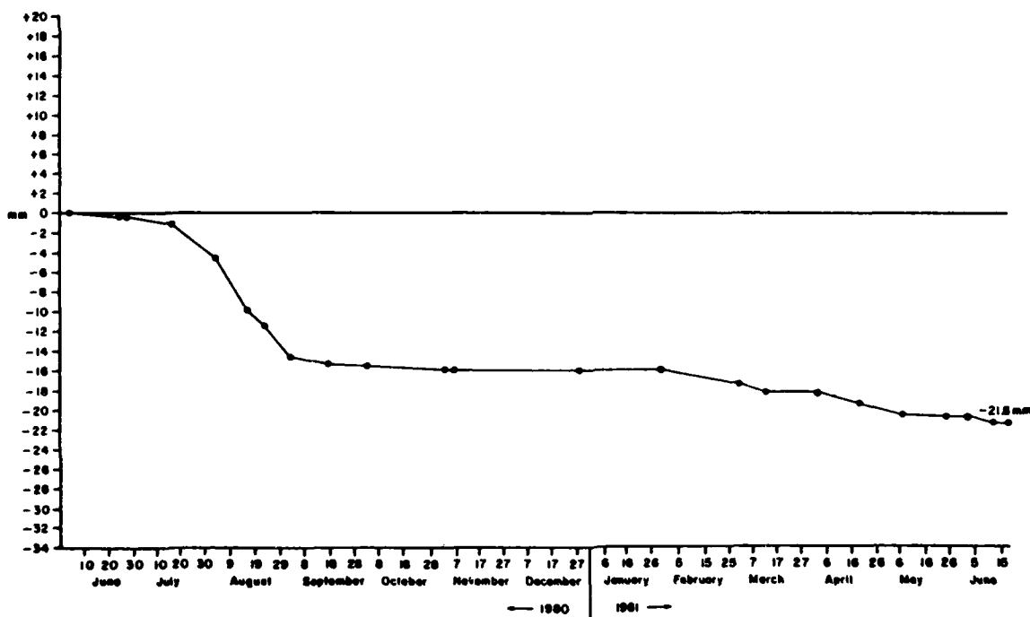
Figure A4.3 Cumulative Average Erosion at Overland Erosion Station #3 Orwell Lake, Minnesota (1980 - 1981)
