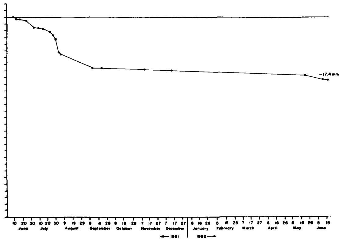
Figure A5.5 Cumulative Average Erosion at Overland Erosion Station #5 Orwell Lake, Minnesota (1981 - 1982)
