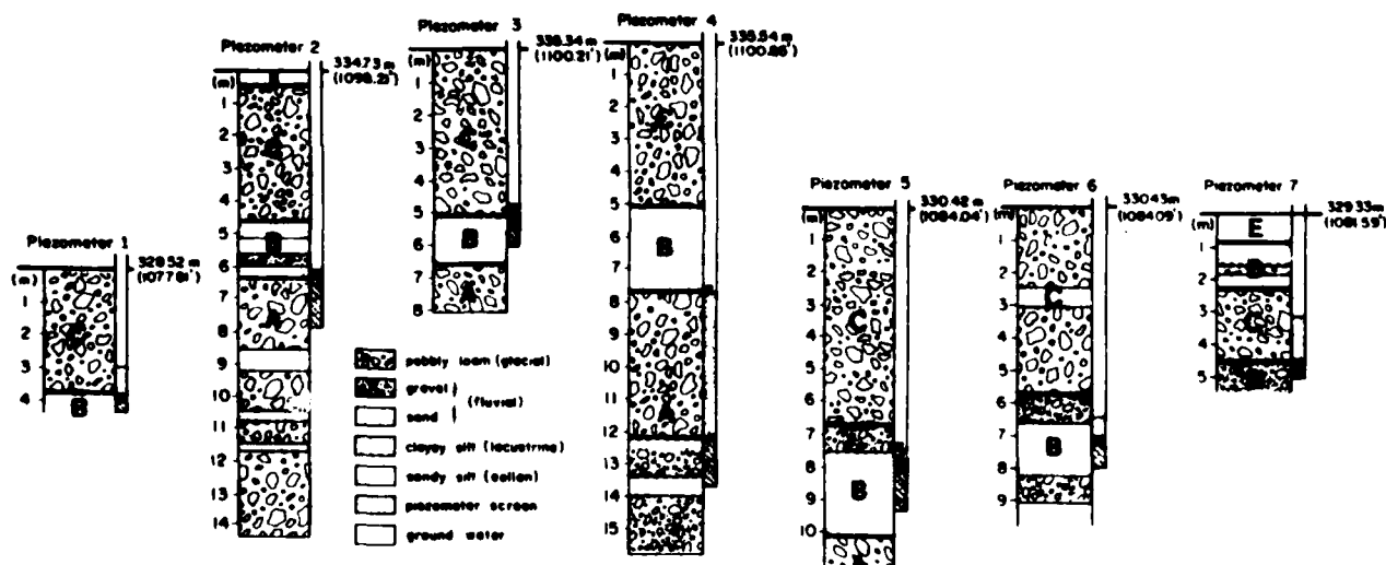
Figure 43. Lithologies and interpreted stratigraphy at the piezometer stations, showing the position of the screen and the water table for each site.
