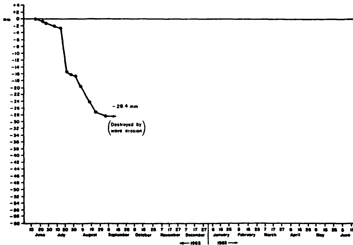
Figure A6.5 Cumulative Average Erosion at Overland Erosion Station # 5 Orwell Lake, Minnesota (1982)
