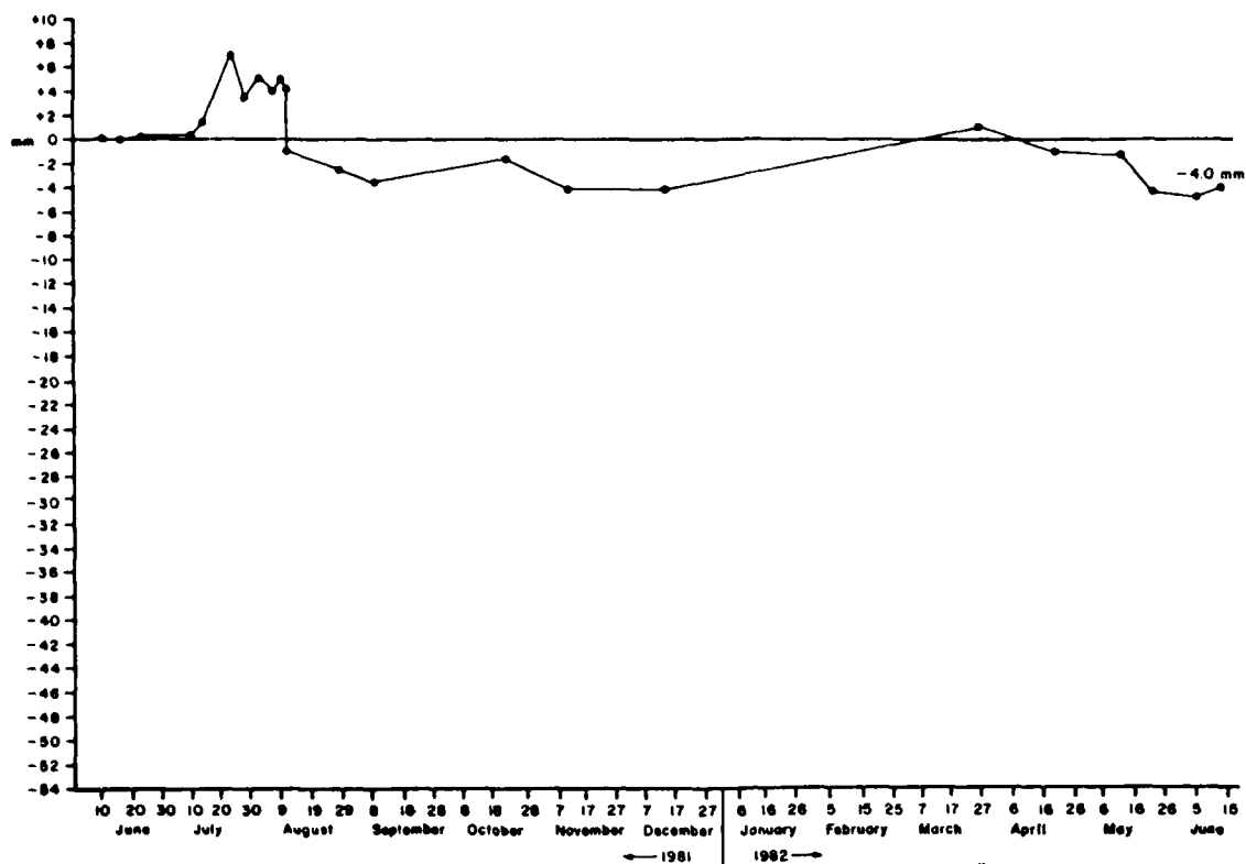
Figure A3.4 Cumulative Net Changes at Overland Erosion Station # 4 Orwell Lake, Minnesota (1981 - 1982)
