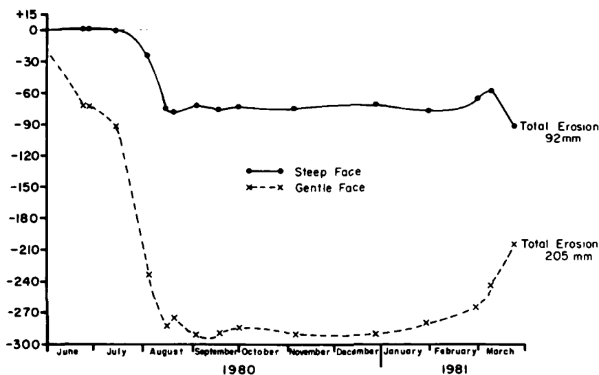
Figure 18. Cumulative net change for steep and gentle slope, erosion station 2, 1980-81.
