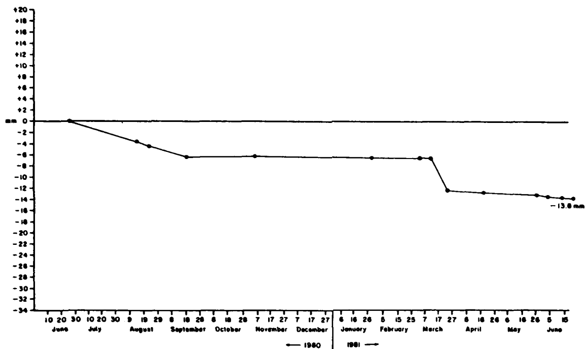
Figure A4.6 Cumulative Average Erosion at Overland Erosion Station # 6 Orwell Lake, Minnesota (1980-1981)
