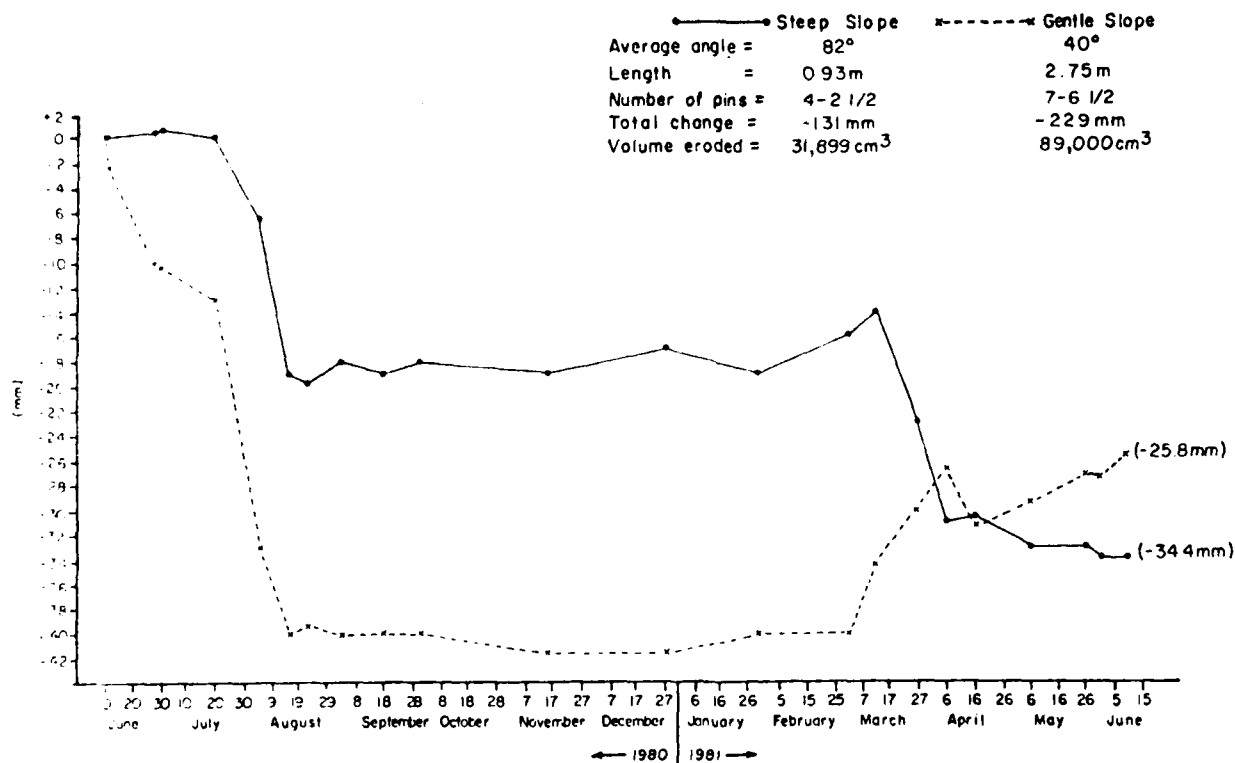
Figure A1.1 Average Cumulative Change of Surface at Erosion Station #2 , 1980-1981. Orwell Lake, Minnesota
