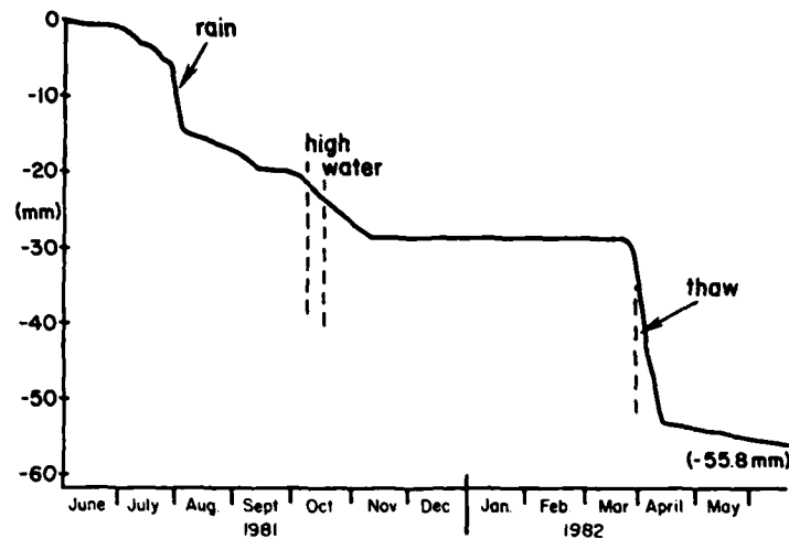
Figure 20. Cumulative average erosion, erosion station 1, 1981-1982.
