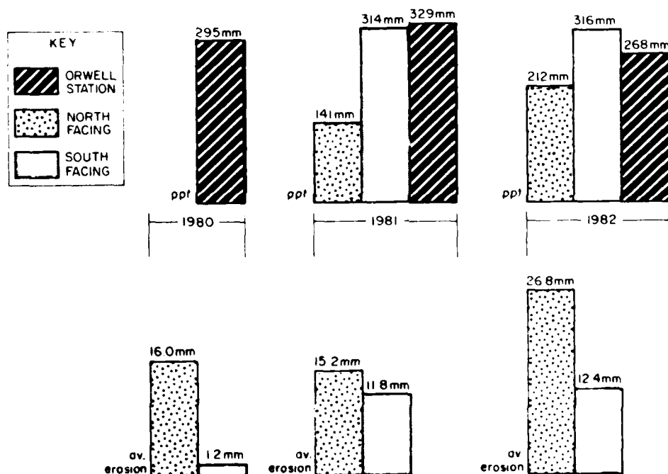
Figure 50. Comparison of bank exposure to variations in summer precipitation and accompanying erosion (June-August, only).
