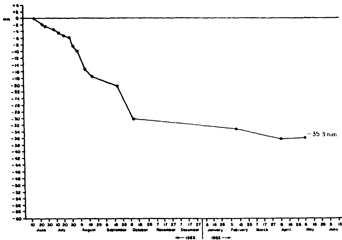
Figure A6.6 Cumulative Average Erosion at Overland Erosion Station #6 Orwell Lake, Minnesota (1982-1983)
