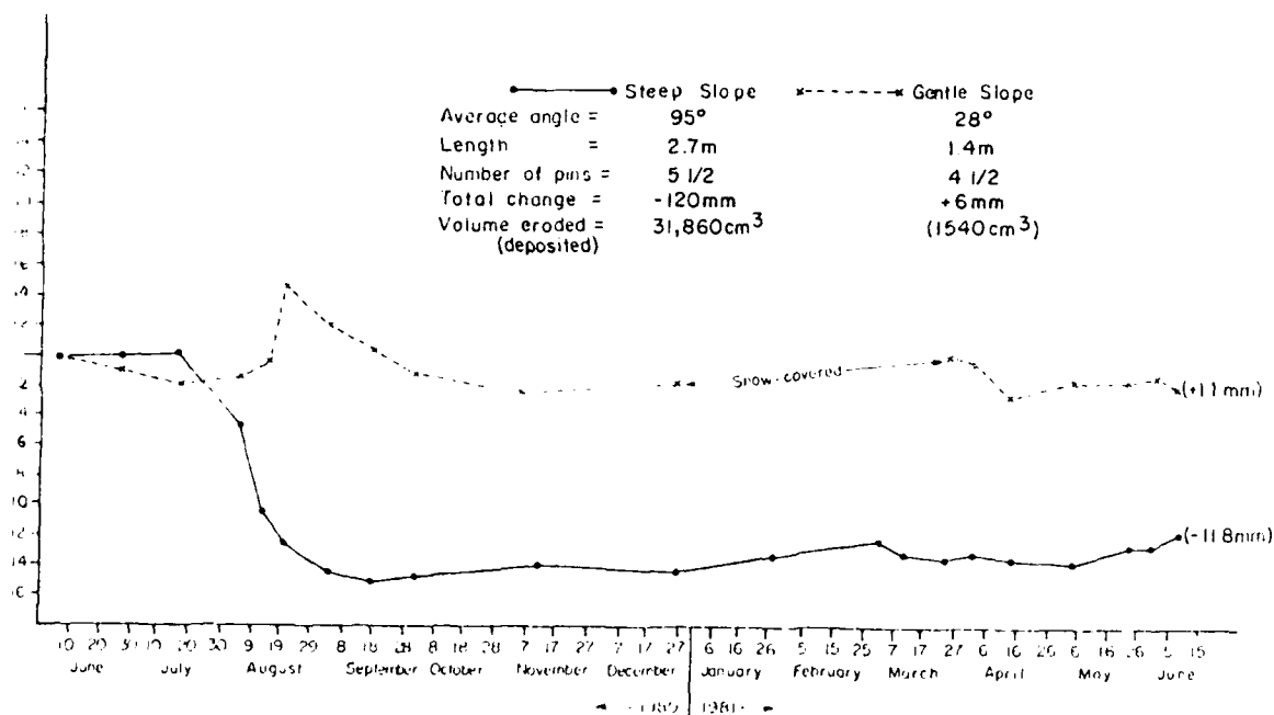
Figure A1.2 Average Cumulative Change of Surface at Erosion Station # 3, 1980-1981. Orwell Lake, Minnesota
