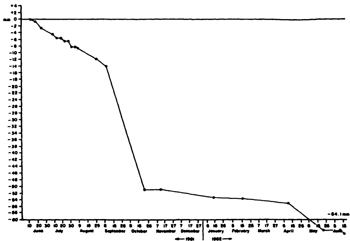
Figure A5.11 Cumulative Average Erosion at Overland Erosion Station #9 Orwell Lake, Minnesota (1981 - 1982)
