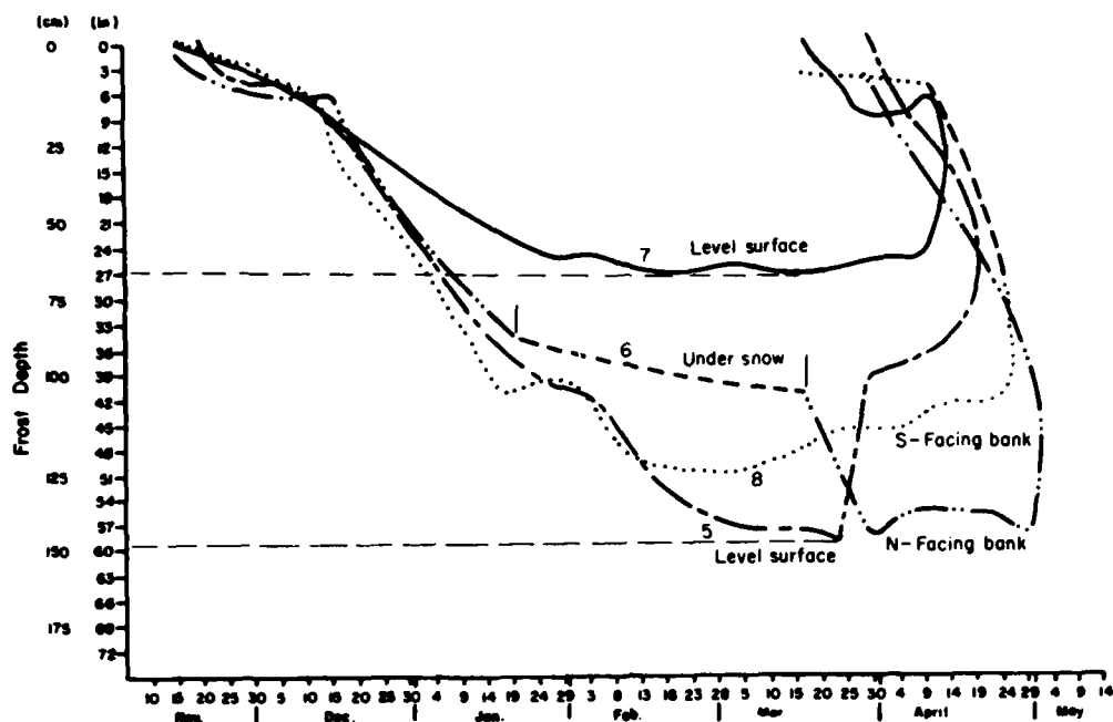
Figure 36. Penetration of frost (winter 1981-82), tubes 5-8.
