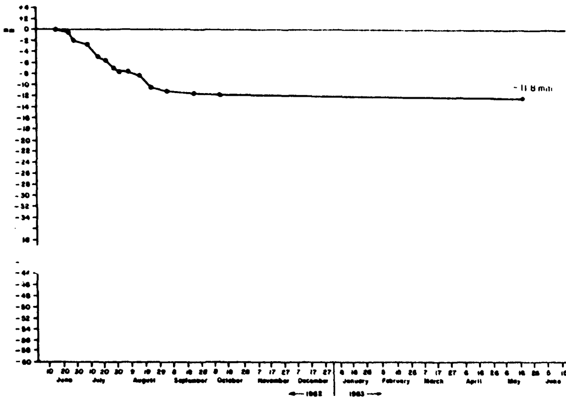
Figure A6.13 Cumulative Average Erosion at Overland Erosion Station #12A Orwell Lake, Minnesota (1982-1983)
