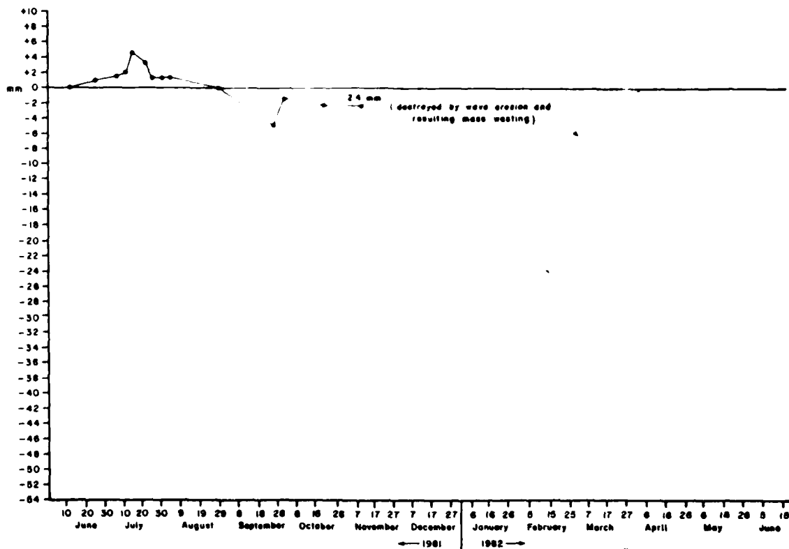
Figure A3.9 Cumulative Net Changes at Overland Erosion Station # 8 A Orwell Lake, Minnesota (1981 - 1982)
