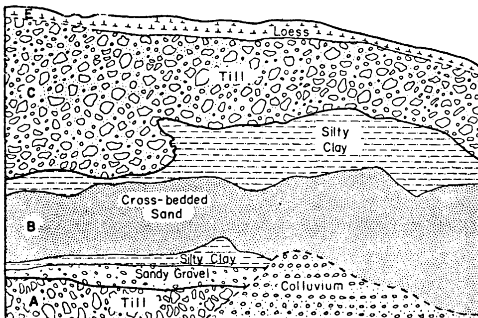
Figure 14. Photograph and interpretive sketch of bank exposure near erosion station 8, showing lithologic units and structures (see Fig. 15 for description of units).
