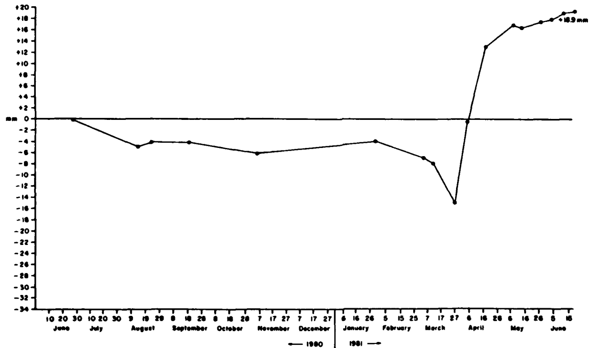
Figure A2.5 Cumulative Net Changes at Overland Erosion Station #5 Orwell Lake, Minnesota (1980-1981)
