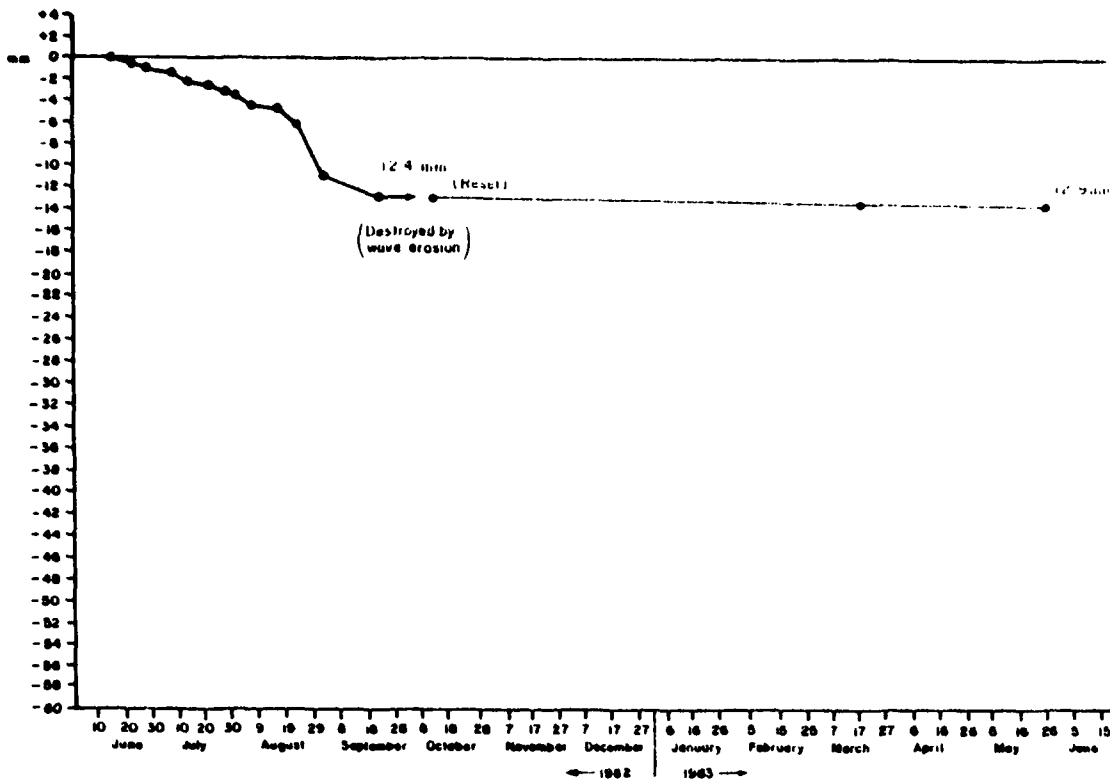
Figure A6.12 Cumulative Average Erosion at Overland Erosion Station #12 Orwell Lake, Minnesota (1982-1983)
