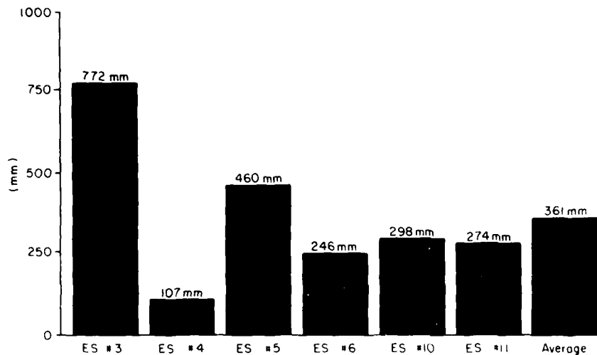
Figure 55. Average yearly bank recession, 1982-83.
