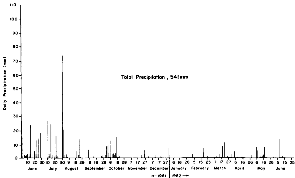
Figure 48. Daily precipitation, Orwell Lake, 1981-1982.
