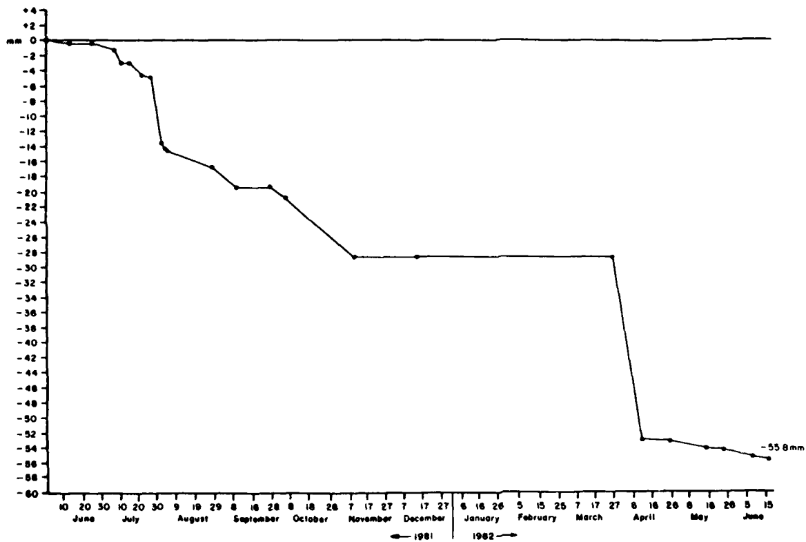
Figure A5.1 Cumulative Average Erosion at Overland Erosion Station #1 Orwell Lake, Minnesota (1981 - 1982)
