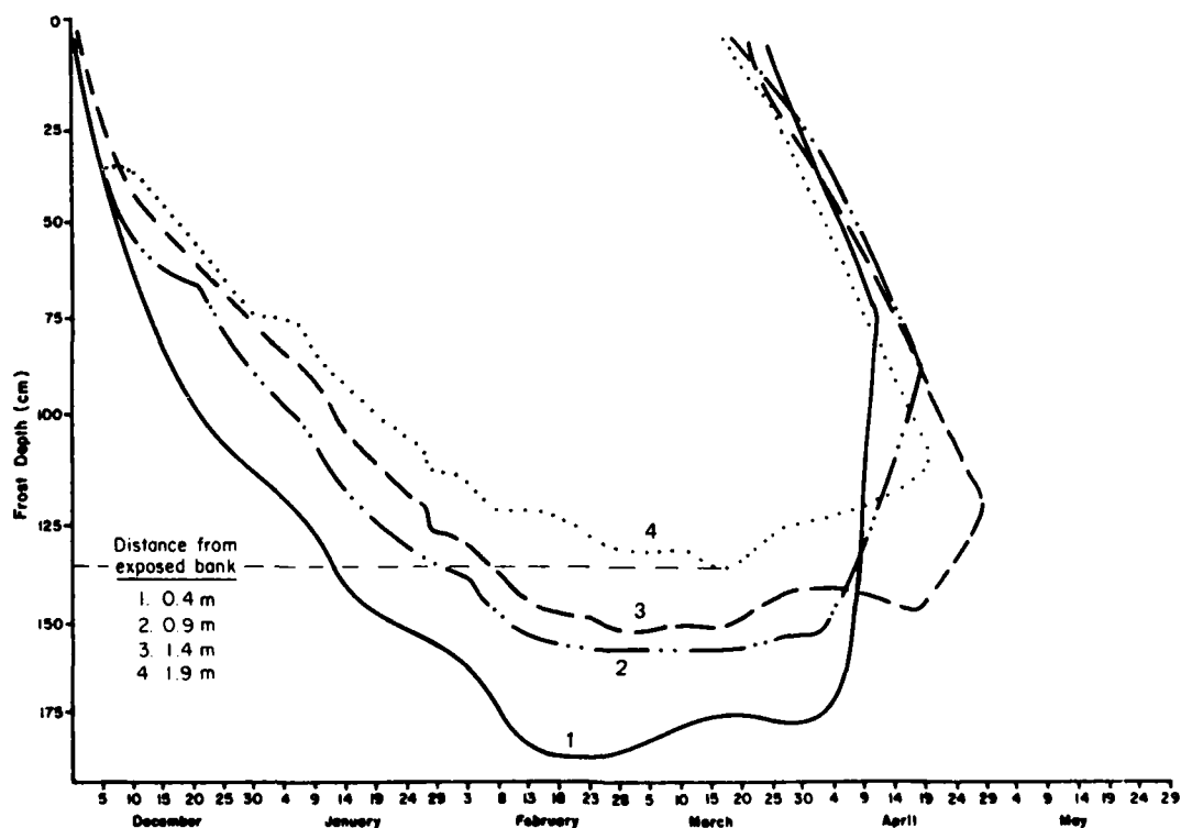
Figure 33. Penetration of frost (winter 1980-81), tubes 1-4.
