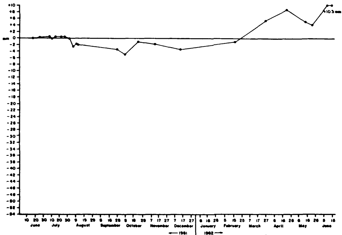
Figure A3.3 Cumulative Net Changes at Overland Erosion Station #3 Orwell Lake, Minnesota (1981 - 1982)
