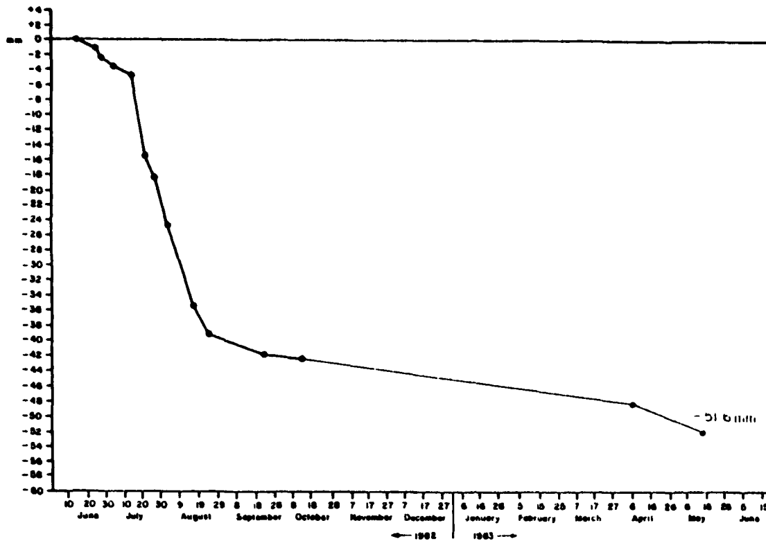
Figure A6.8 Cumulative Average Erosion at Overland Erosion Station #8 Orwell Lake, Minnesota (1982-1983)
