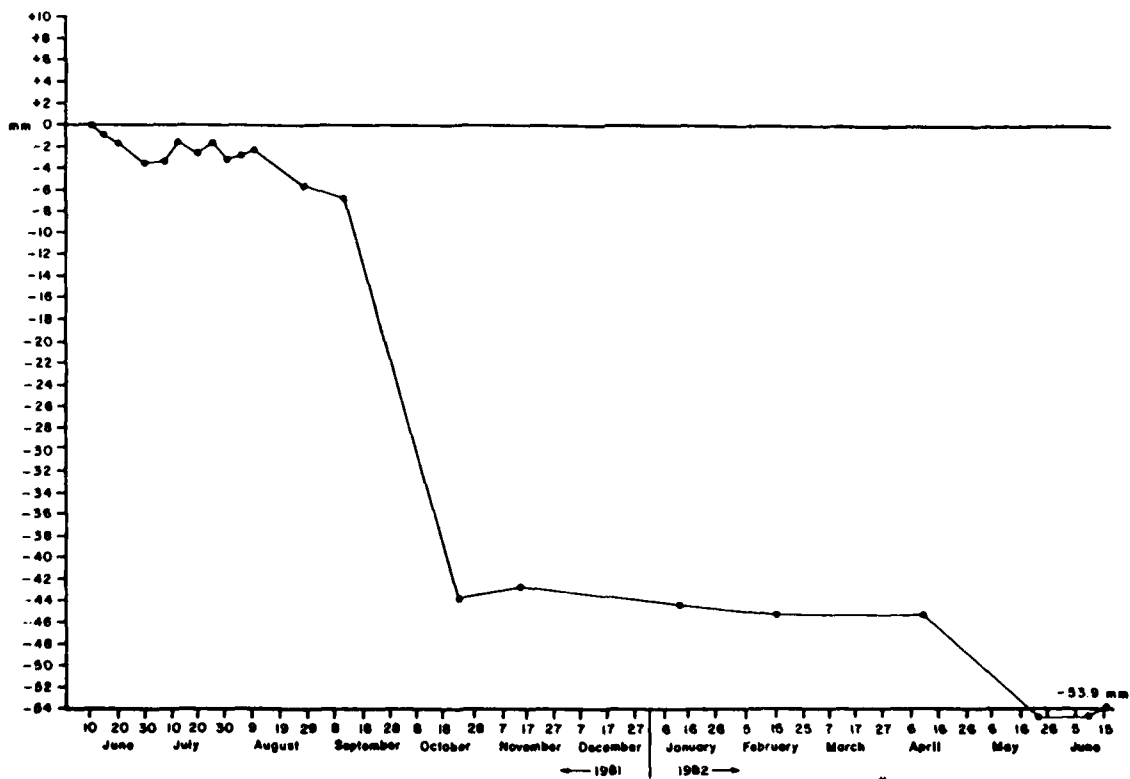
Figure A3.11 Cumulative Net Changes at Overland Erosion Station # 9 Orwell Lake, Minnesota (1981 - 1982)
