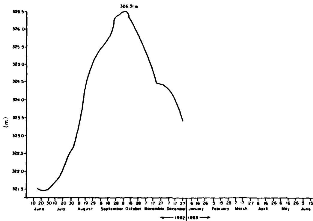
Figure 29. Orwell Lake pool levels, 1982.
