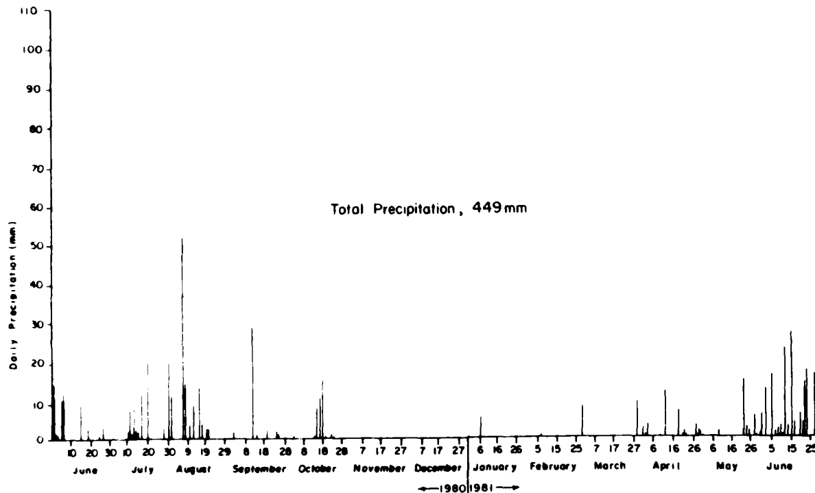
Figure 47. Daily precipitation, Orwell Lake, 1980-1981.
