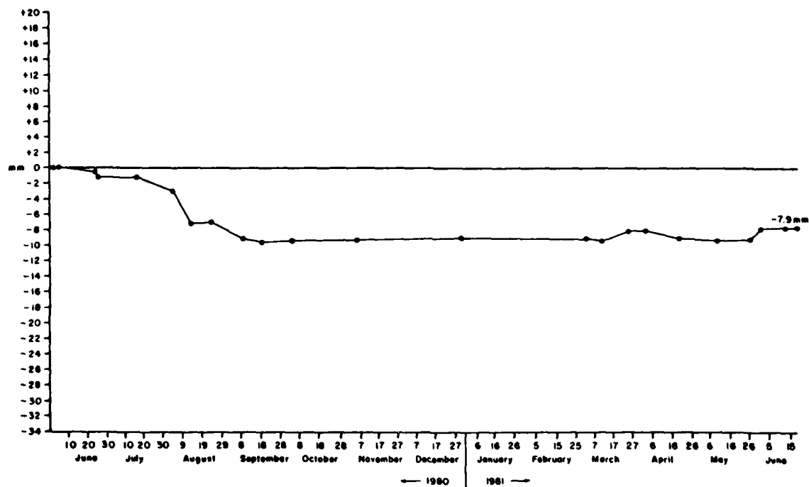
Figure A2.3 Cumulative Net Changes at Overland Erosion Station #3 Orwell Lake, Minnesota (1980-1981)
