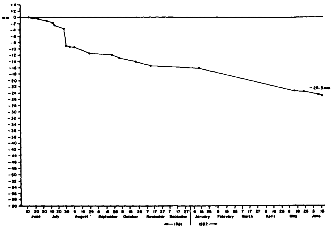
Figure A5.7 Cumulative Average Erosion at Overland Erosion Station #7 Orwell Lake, Minnesota (1981 - 1982)
