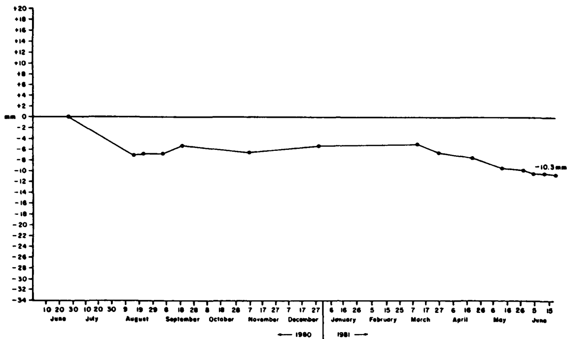
Figure A2.8 Cumulative Net Changes at Overland Erosion Station #8 Orwell Lake, Minnesota (1980-1981)
