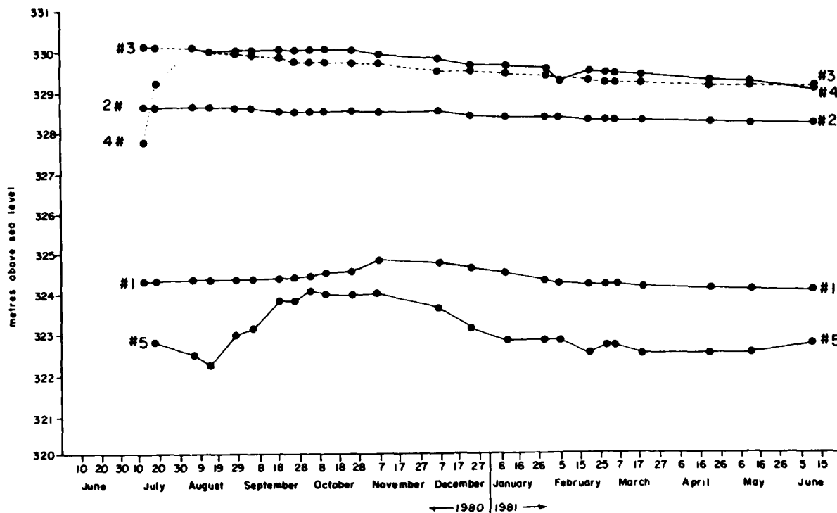
Figure 44. Piezometric head fluctuations, 1980-81.
