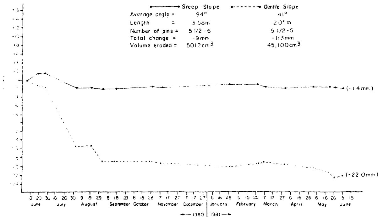
Figure A1.9 Average Cumulative Change of Surface at Erosion Station #10, 1980-1981, Orwell Lake, Minnesota
