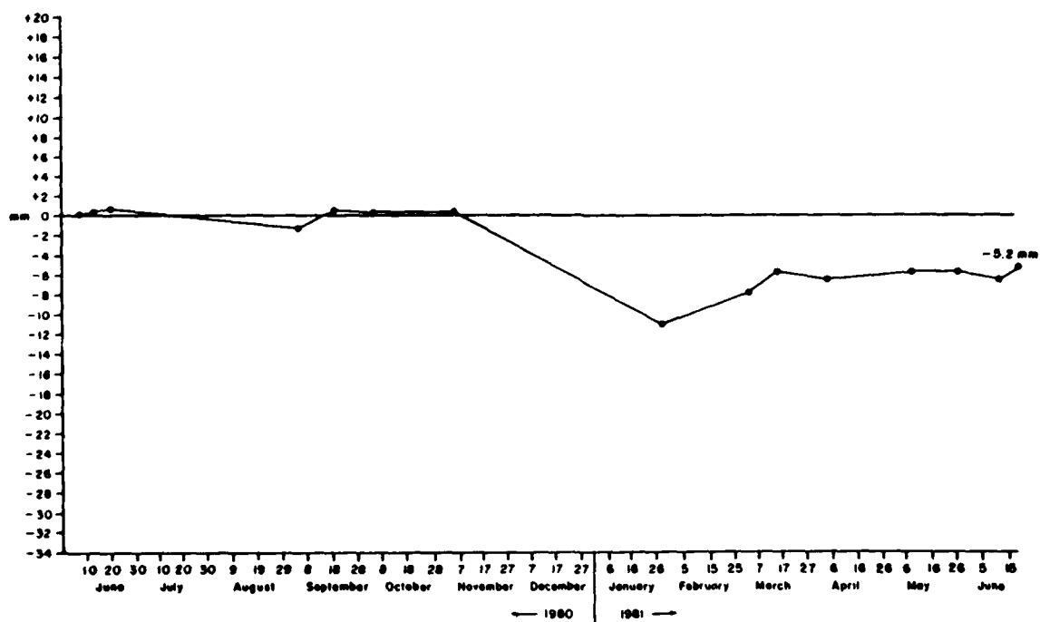
Figure A2.11 Cumulative Net Changes at Overland Erosion Station #11 Orwell Lake, Minnesota (1980-1981)
