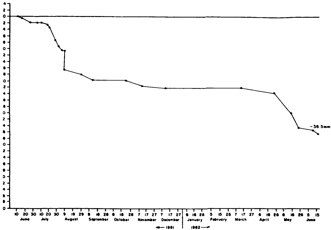
Figure A5.4 Cumulative Average Erosion at Overland Erosion Station #4 Orwell Lake, Minnesota (1981 - 1982)
