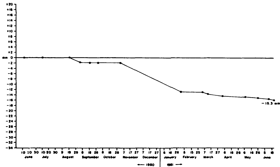
Figure A4.11 Cumulative Average Erosion at Overland Erosion Station #11 Orwell Lake, Minnesota (1980-1981)
