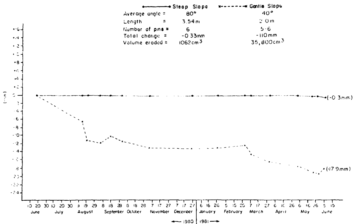
Figure A1.8 Average Cumulative Change of Surface at Erosion Station #9, 1980-1981, Orwell Lake, Minnesota
