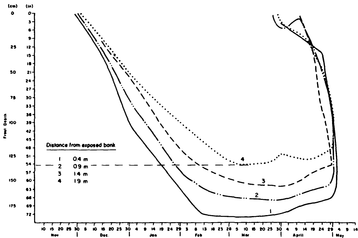
Figure 35. Penetration of frost (winter 1981-82), tubes 1-4.
