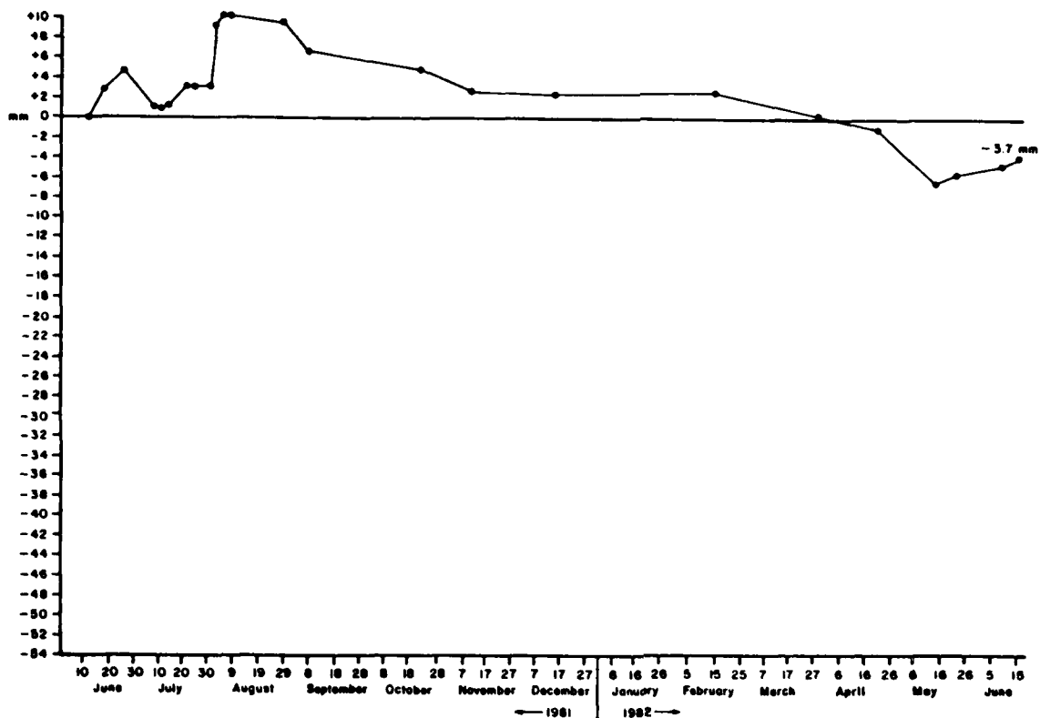
Figure A3.2 Cumulative Net Changes at Overland Erosion Station #2 Orwell Lake, Minnesota (1981 - 1982)
