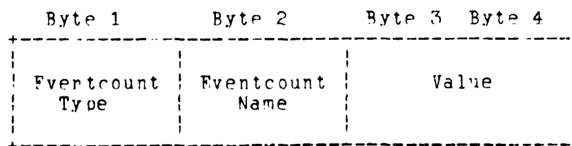
Figure 8 Ethernet Request Packet Format
