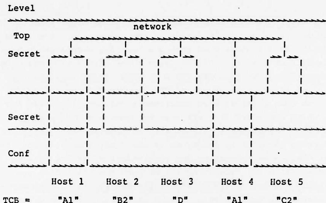
FIGURE III-11. Trusted and Untrusted Computers on a System-High Network
