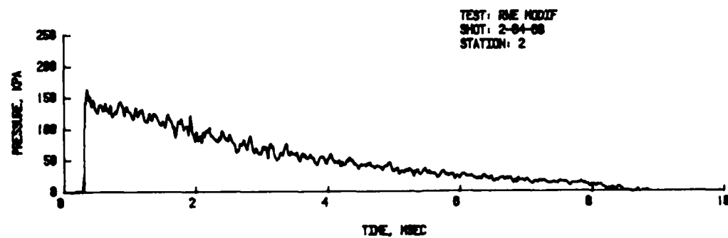
Figure 8. Overpressure Versus Time at Station 2, Input Pressures 20, 50, 100, and 150 kPa, Long Tube without an RWF
