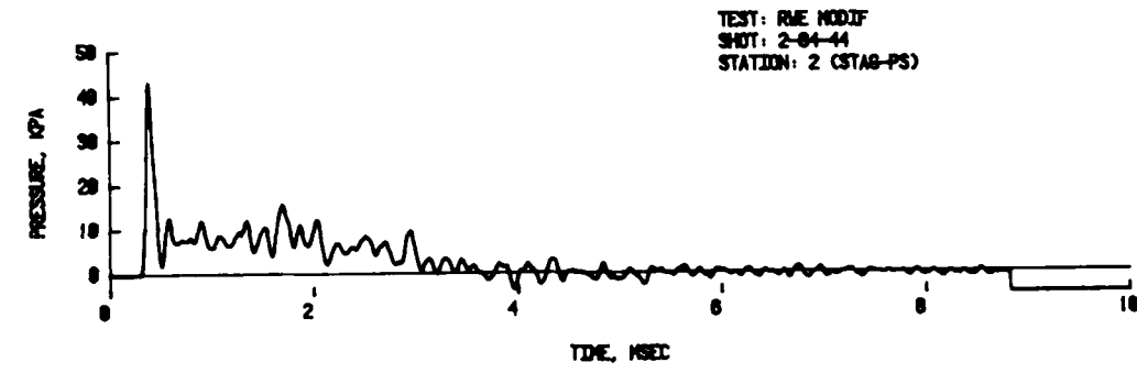
Figure 14. Vented Foam Plate 500, 50 kPa Input Pressure
