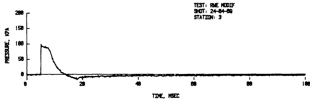
Figure 23. Pressure-Time Records, No BPP, 100 kPa Input Pressure, 0.17 Metre Shock Tube
