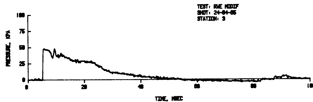
Figure 24. Pressure-Time Records, Vented Foam FWE, 50 kPa Inlet Pressure, 0.57 Metre Shock Tube
