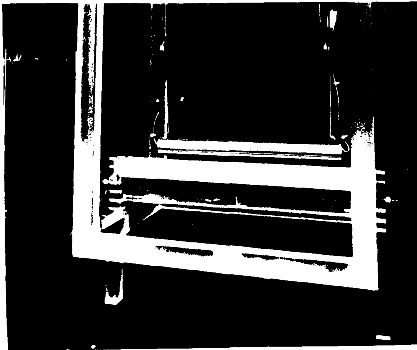
Figure 4. Photograph of Cylinder in Test Section with Shroud Installed
