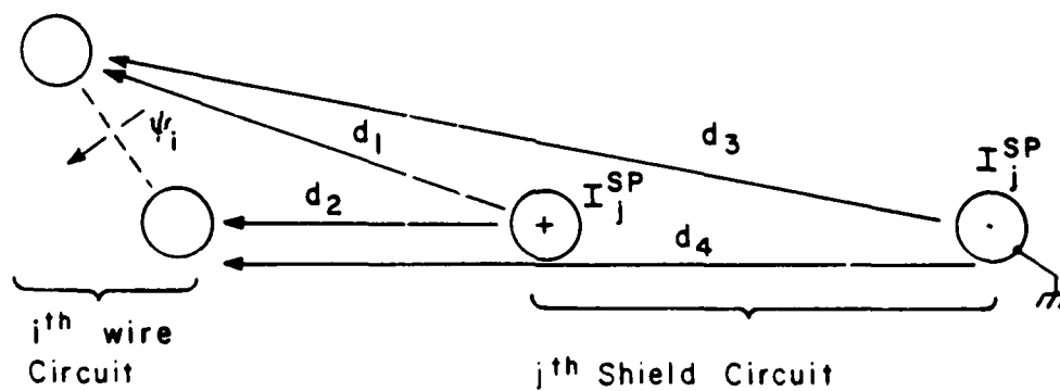
Figure 2.18 - Mutual Inductance Between the i^{\text{th}} Wire Circuit and the j^{\text{th}} Shield Circuit over the Pigtail Sections.
