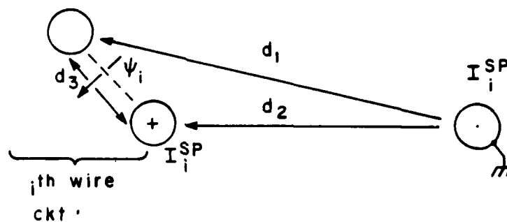
Figure 2.17 - Mutual Inductance Between the i^{\text{th}} Wire Circuit and the i^{\text{th}} Shield Circuit over the Pigtail Sections.
