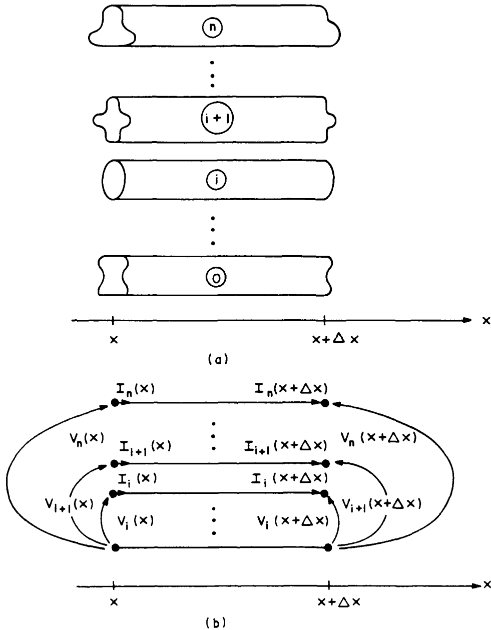
Figure 2.2 - General Transmission Line.
