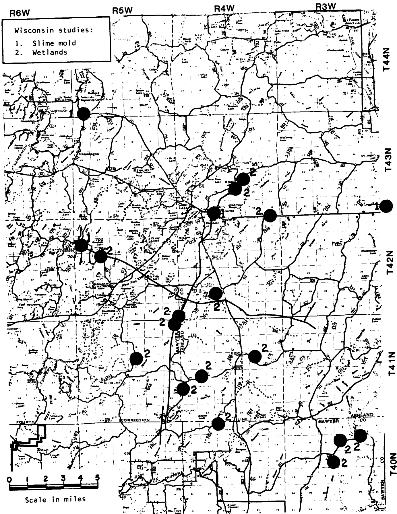
Figure 2. Field sites for Wisconsin ecology studies.
