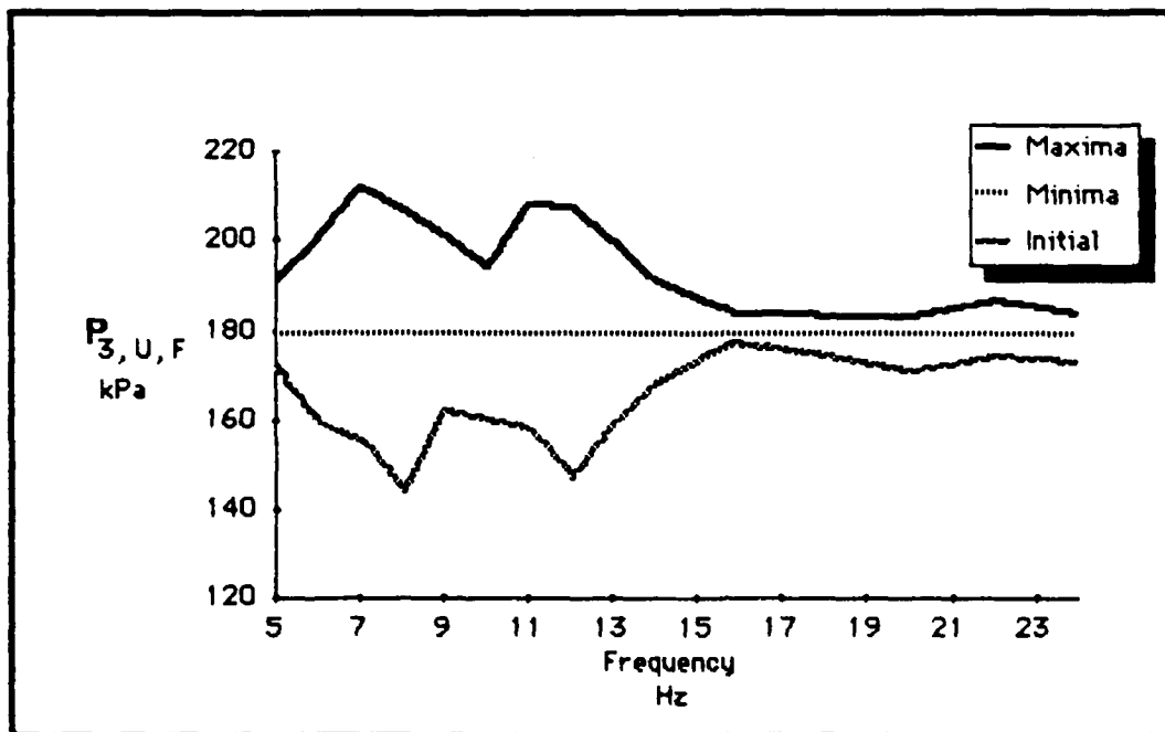
Figure 5.24 Fuel pump inlet pressure frequency response (large compliance).
