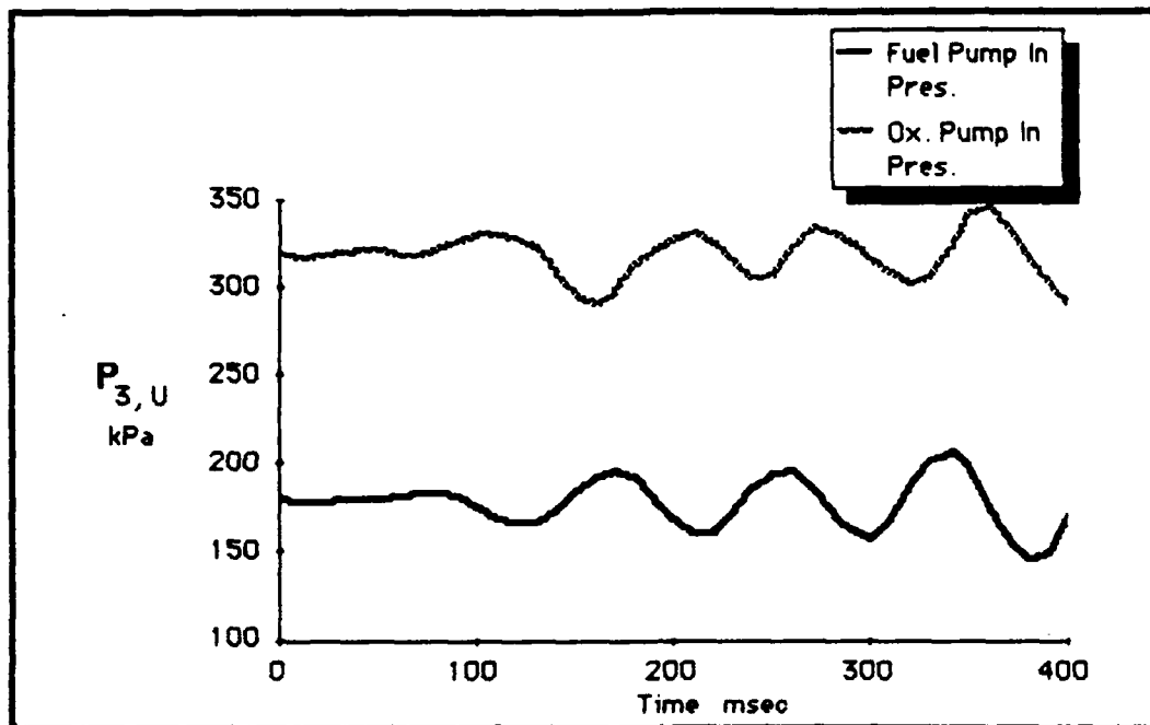
Figure 5.18 Bipropellant system pump inlet pressures (large compliance).
