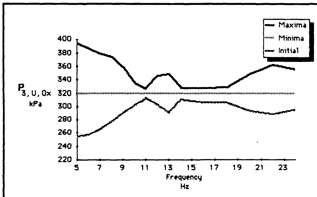
Figure 5.27 Ox. pump inlet pressure frequency response (large compliance).
