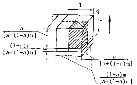
Fig. 2 A unit cubes cell equivalent to the unit cell illustrated in Fig. 1 (b)
