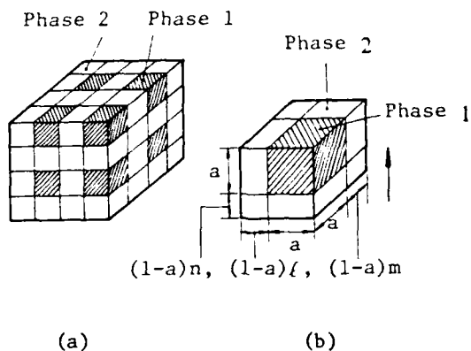
Fig. 1(a) A composite with 3-0 connectivity and (b) a unit cell of the composite
