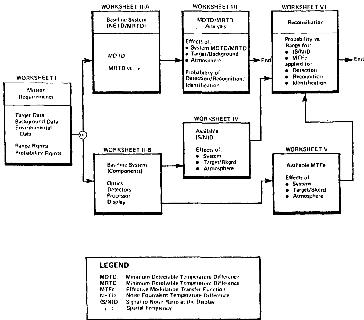
FIGURE: Flow of FLIR system requirements manual.
