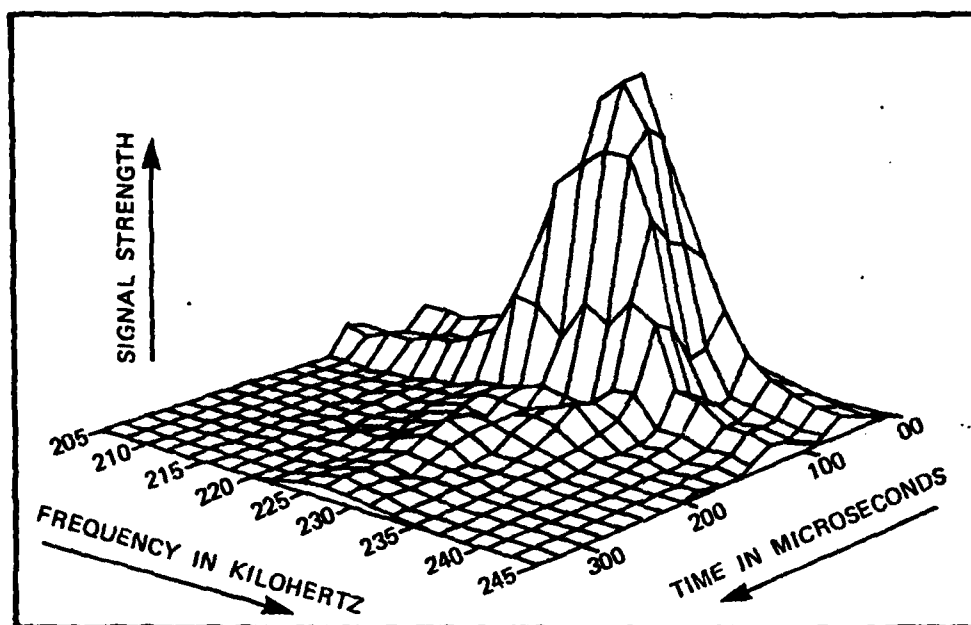
FIGURE: Echo Structure Display.
