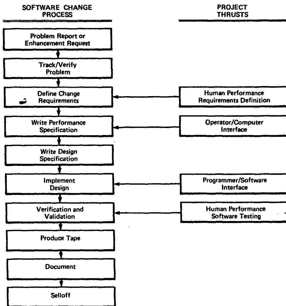
FIGURE: Project Intervention in Software Change.
