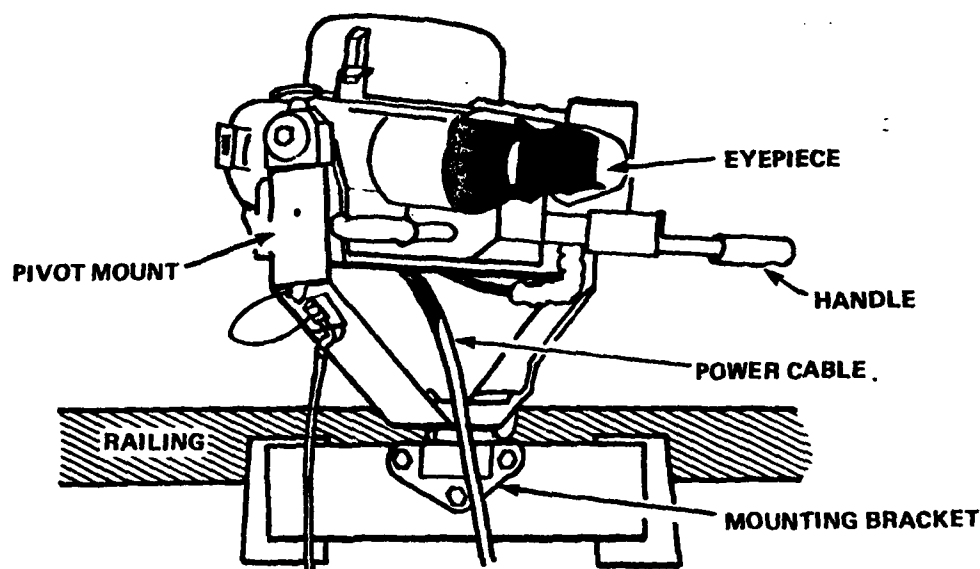
FIGURE: AN/KAS-1 Sensor Unit.
