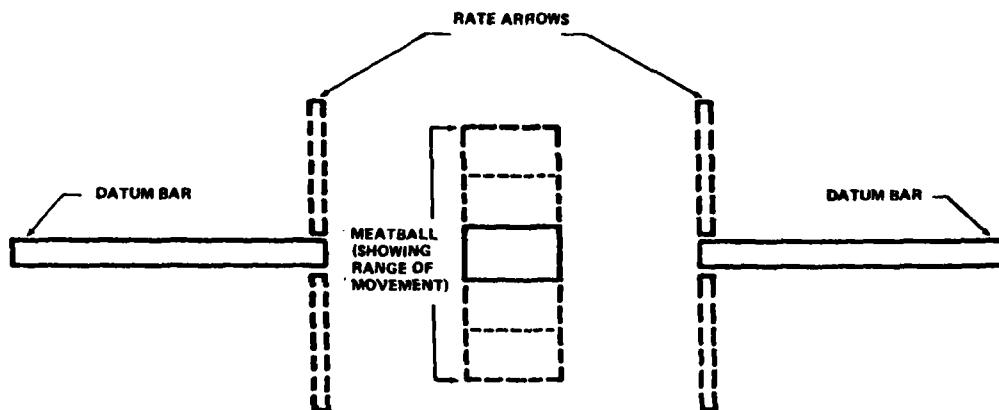
FIGURE: AVCARs Modified FLOLS Display.
