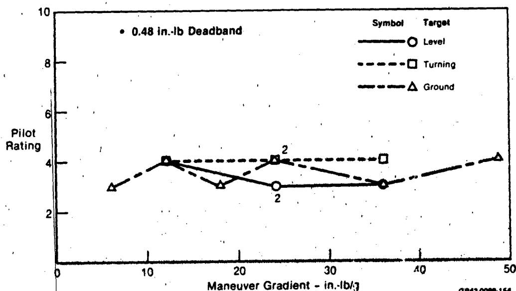
Figure 85. Pilot Rating vs Maneuver Gradient Twist Grip Sidestick Wings Level Turn Pilot 22
