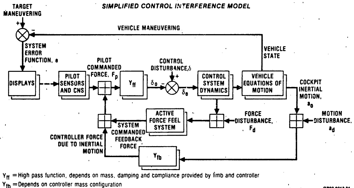
Figure 27. Conceptual Block Diagram for Task Inputs and Measurement Variables
