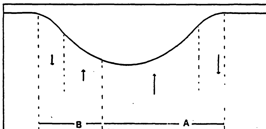
Figure 6.13. The effects of a uniform westward translation on the decay of anticyclonic (a), and cyclonic flow (b). Regions A and B indicate regions where dissipation is more and less effective with respect to the correspondent stationary flow, respectively. Arrows represent the direction of the Ekman velocity at the top of the BBL.
