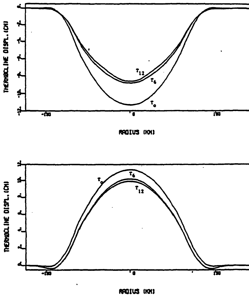
Figure 6.4. The displacement of the thermocline at time t=0, 6 , and 12 months; (a) cyclonic flow, (b) anticyclonic flow.
