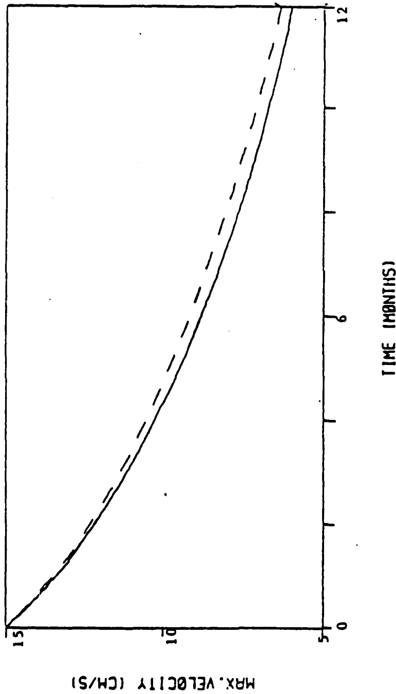
Figure 5.5. The decay at the location of maximum velocity of a cyclonic flow computed with the level 2½ closure scheme (solid line) and relating the Ekman velocity to the Ekman velocity of the correspondent LBL (dashed line).
