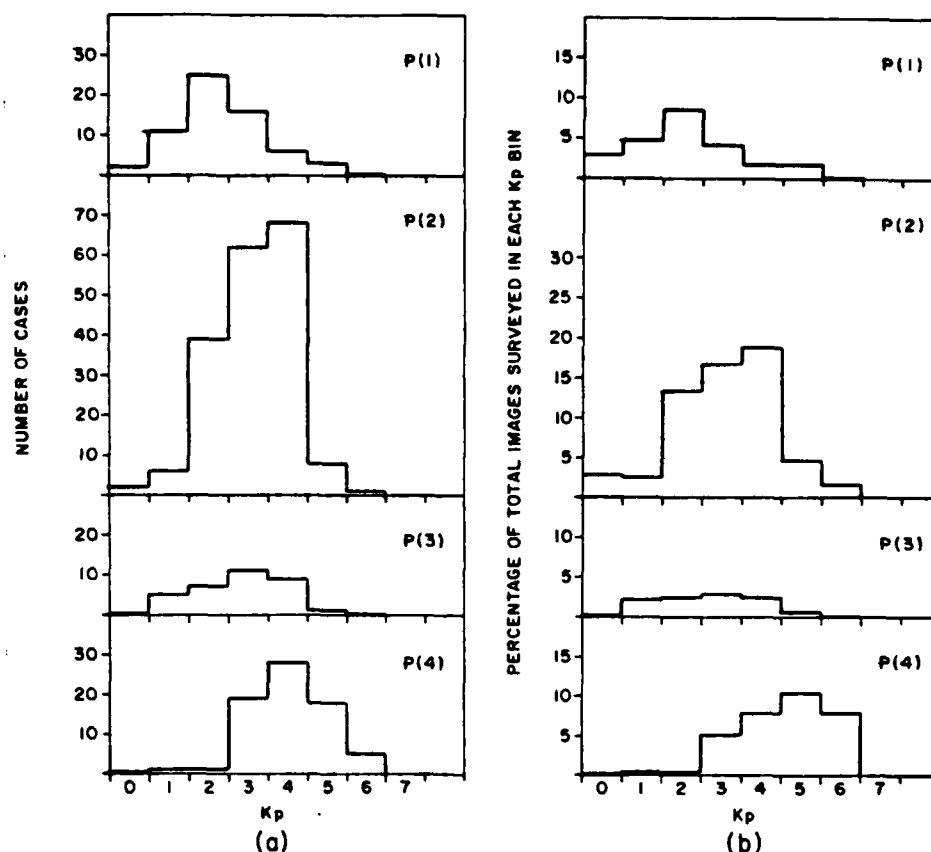
Fig. 3. (a) The distribution of extremely high latitude auroras, by category, according to Kp . (b) The distribution in Kp of the percentage of cases of extremely high latitude auroras in each Kp bin with respect to the number of images in the total survey for that bin. The distribution is separated by category.
