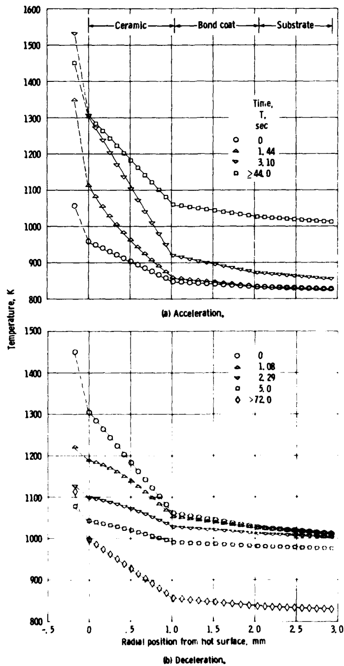
Figure 11. - Variation of shroud temperature profile with time.
