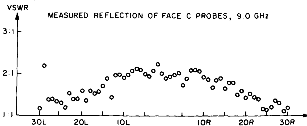
Figure 2. Measured VSWR of Nonuniformly Spaced Concave Circular Array Elements
