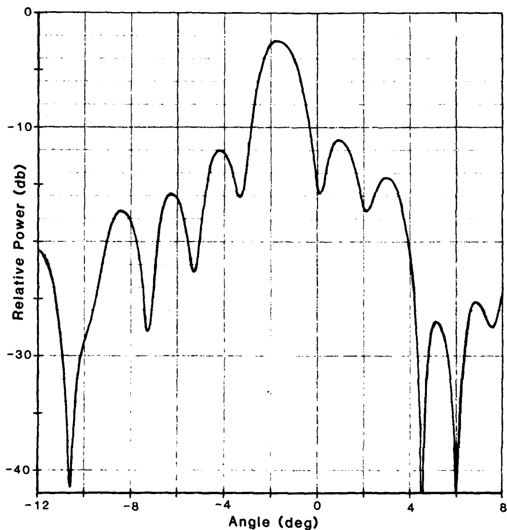
Figure 3. Pattern of Array Lens Beam Port 1L
