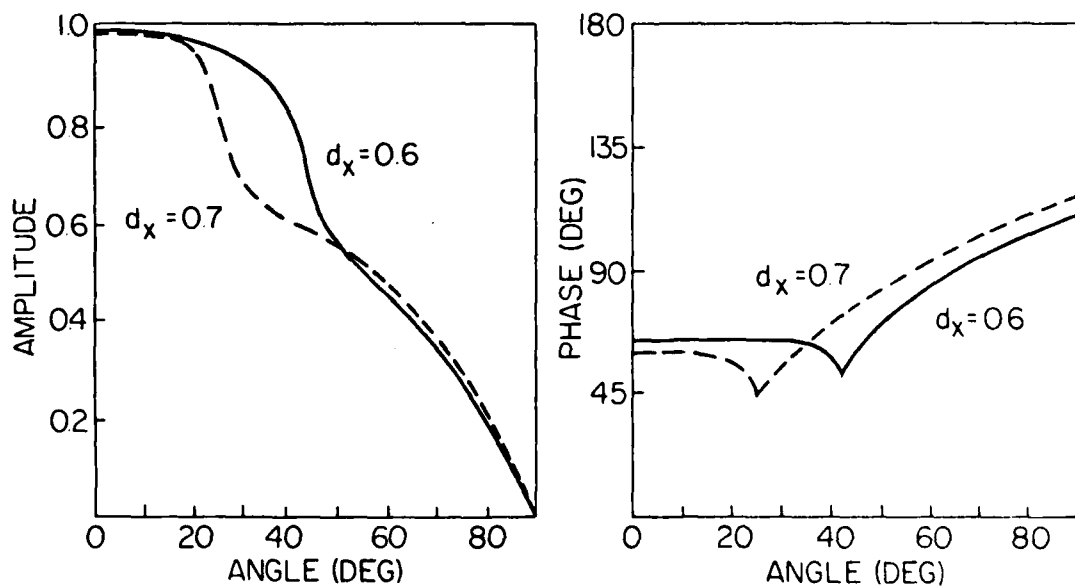
Figure 12. Theoretical Monopole Element Patterns (Tomasic and Hessel)
