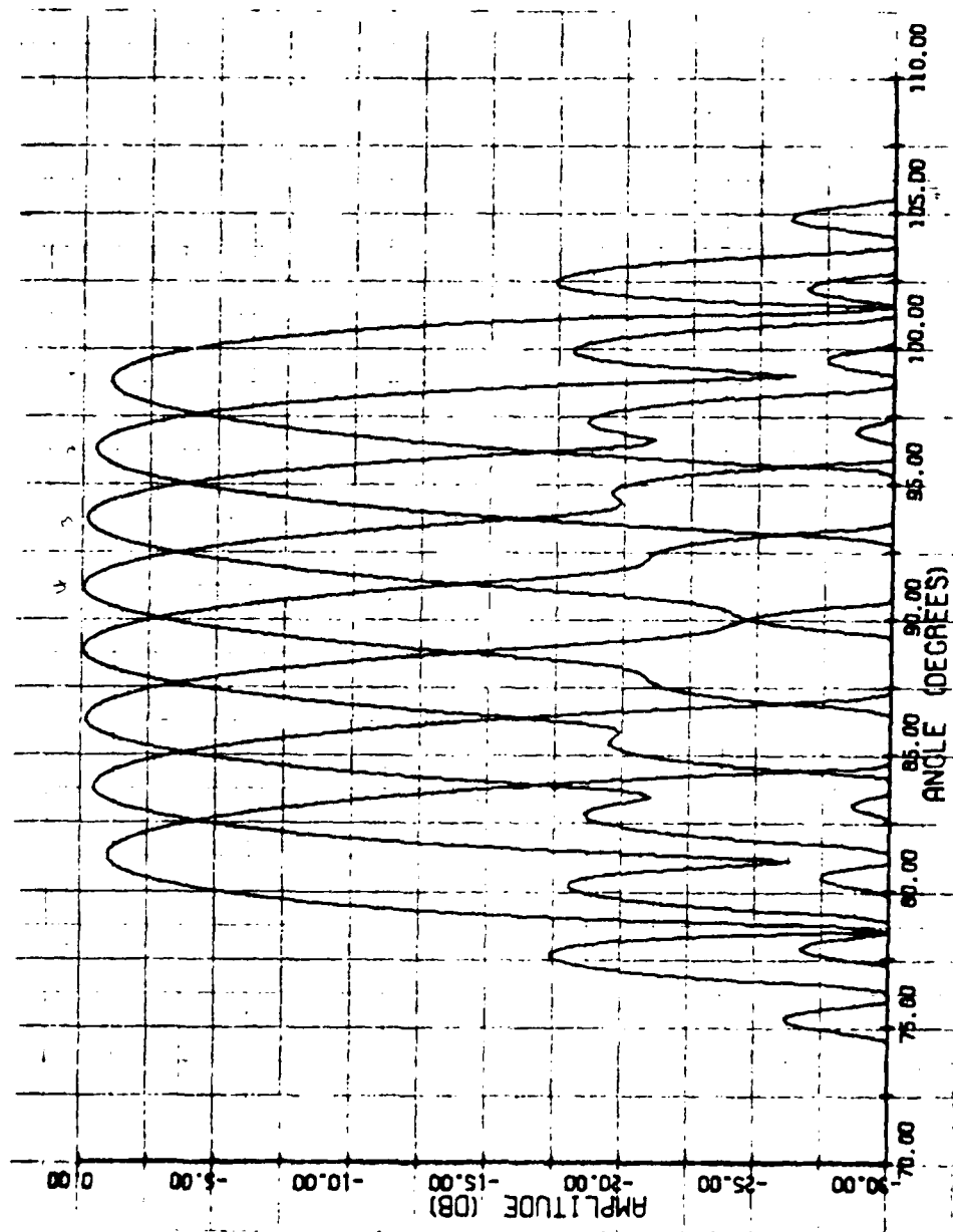
Figure 6 Eight Multiple Beams for an Aperture Edge Taper of -6 dB
