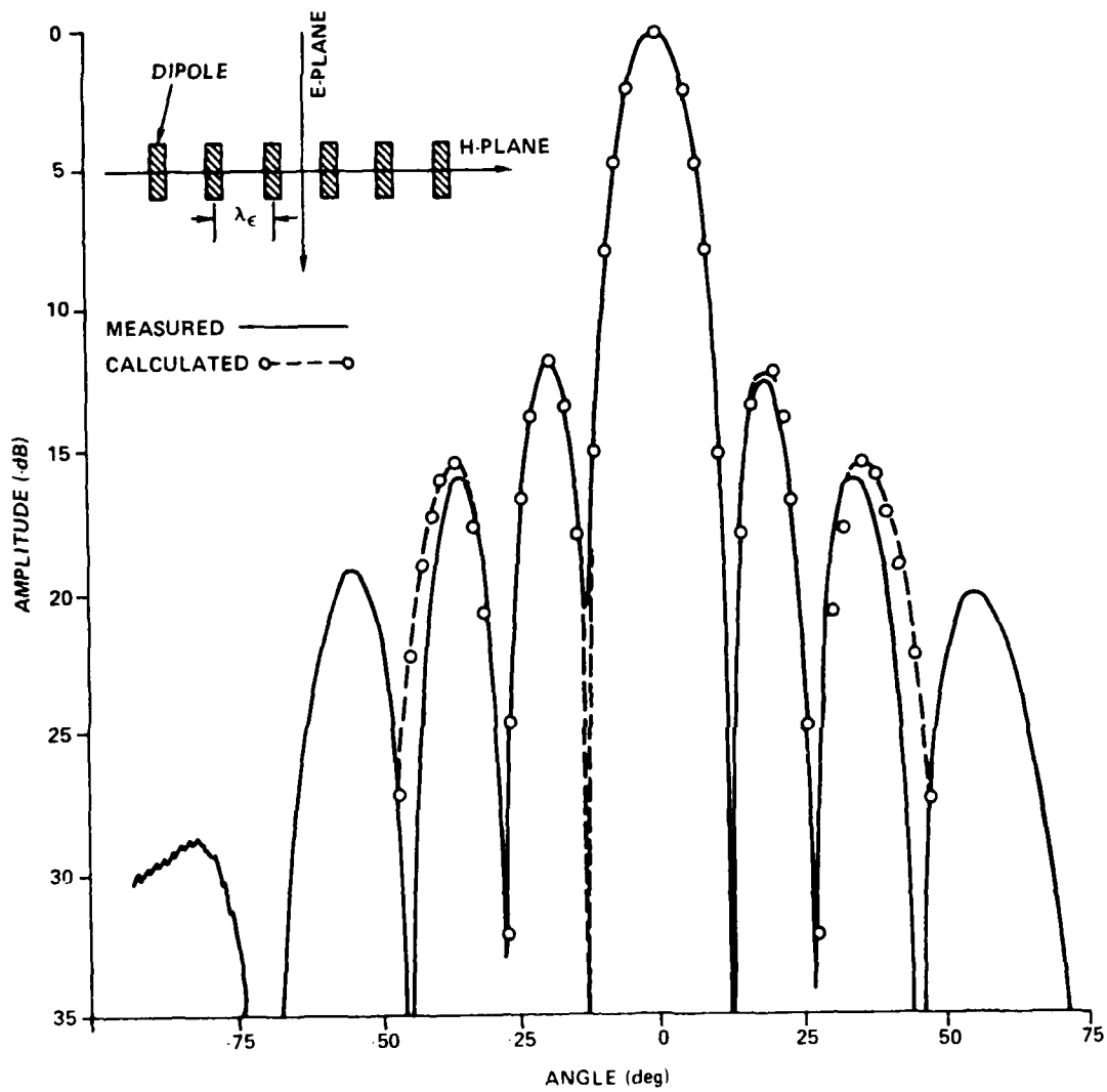
Figure 4. H-Plane Radiation Pattern of 6 Element Linear Array
