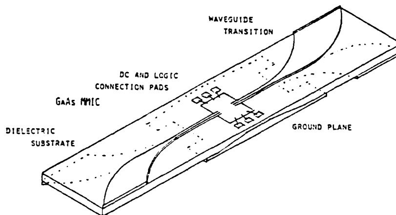
Figure 2. MMIC interconnectivity.
