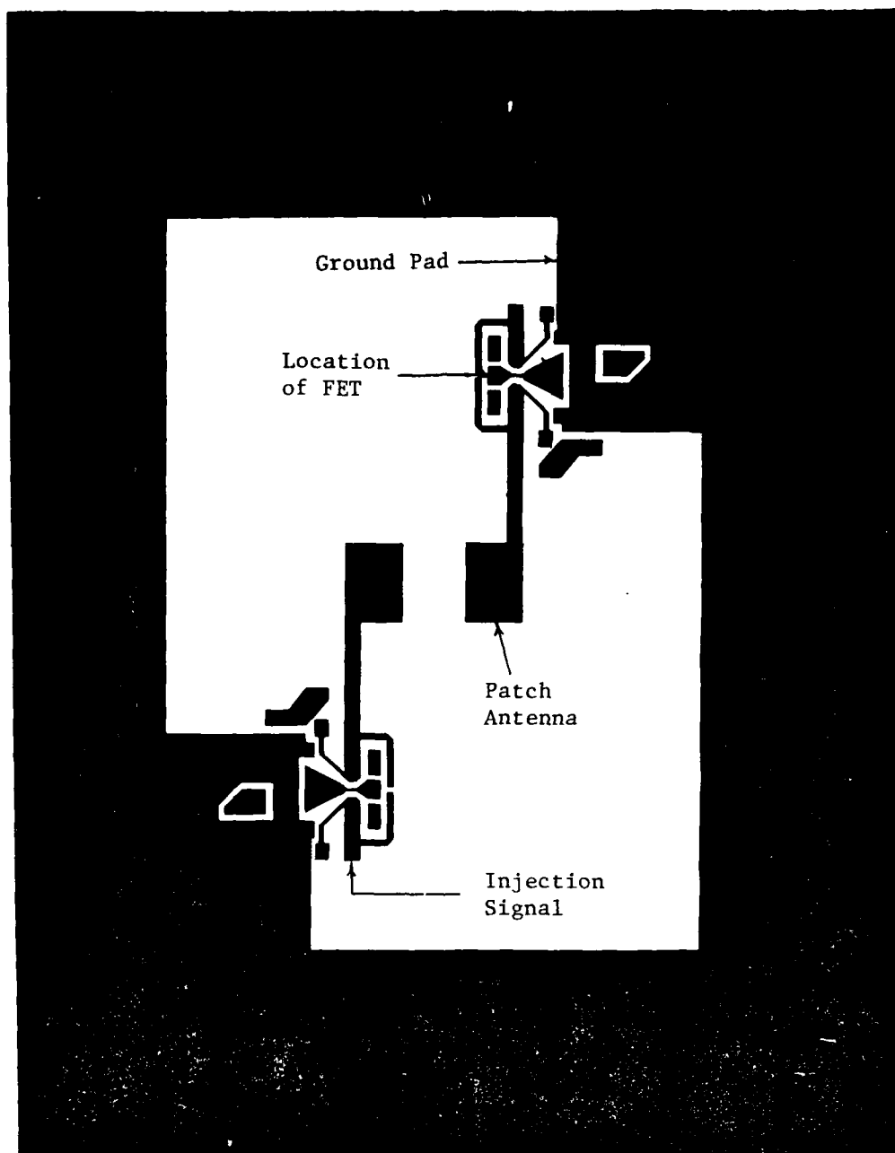
Figure 13. Photolithographic mask for injection-locked oscillators and antennas.
