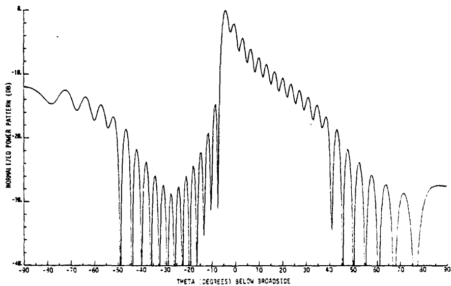
Figure 9b. Final Pattern for 26-Element Shaped Beam Synthesis
