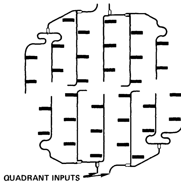
Figure 7. Full Microstrip Array Artwork
