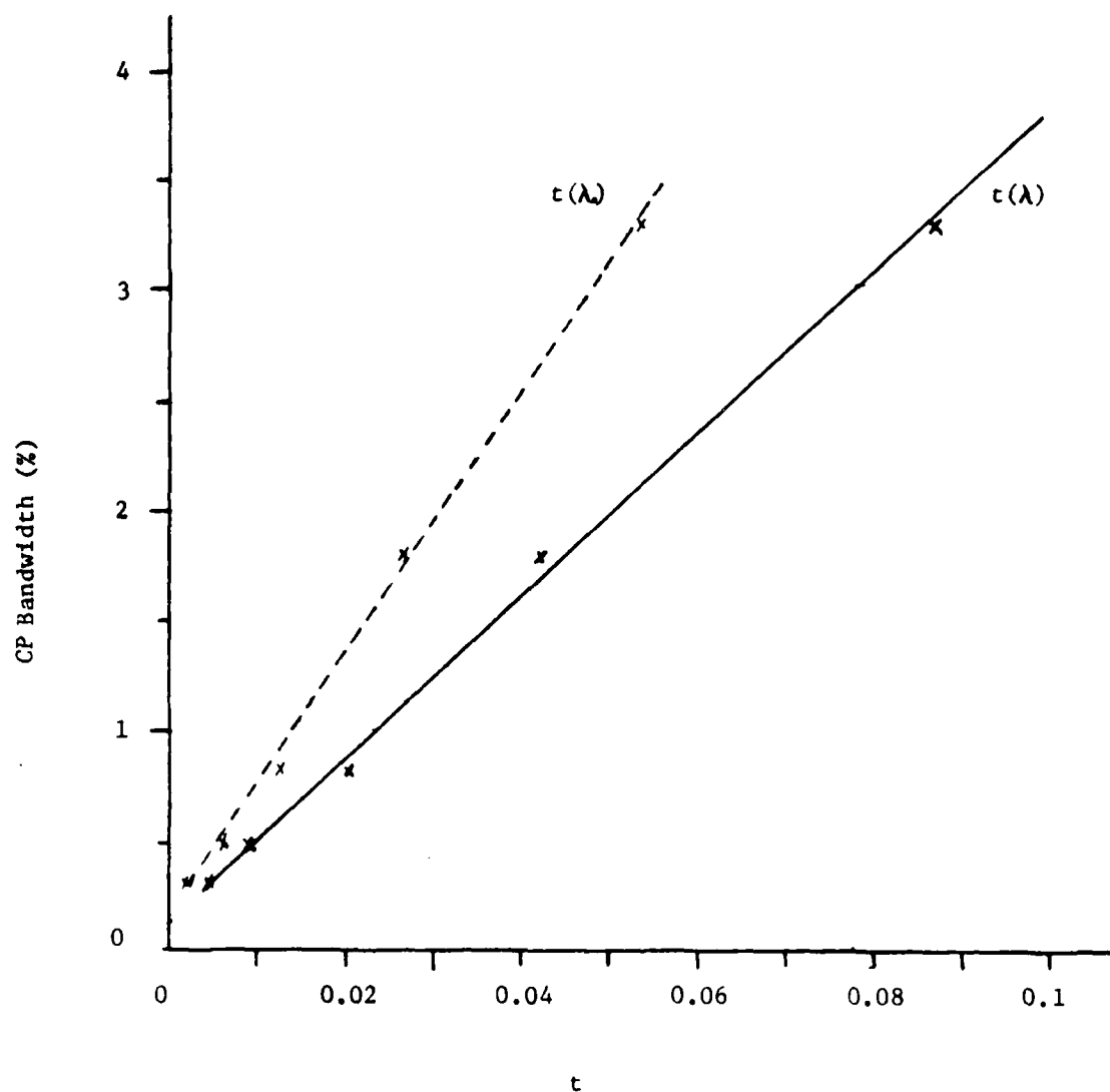
Figure 7. Bandwidth vs. the substrate thickness t , expressed in terms of free space wavelength, \lambda_0 , or substrate dielectric wavelength \lambda .
