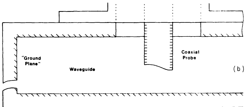
Figure 11. (a) Apparent Phase Center Location versus Frequency relative to (b) Probe/Waveguide Geometry
