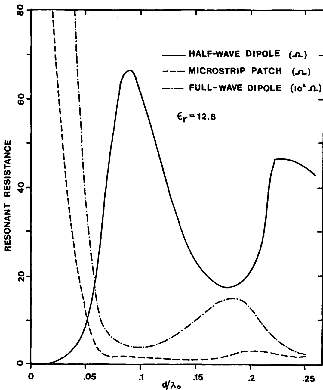
Figure 1. Input resistance of resonant microstrip patch and dipoles (half-wave and full-wave) on substrate \epsilon_r = 12.8 of thickness d . Dipoles are center fed and patch is fed at a point L/4 from edge. Patch width is 0.3\lambda_0 .
