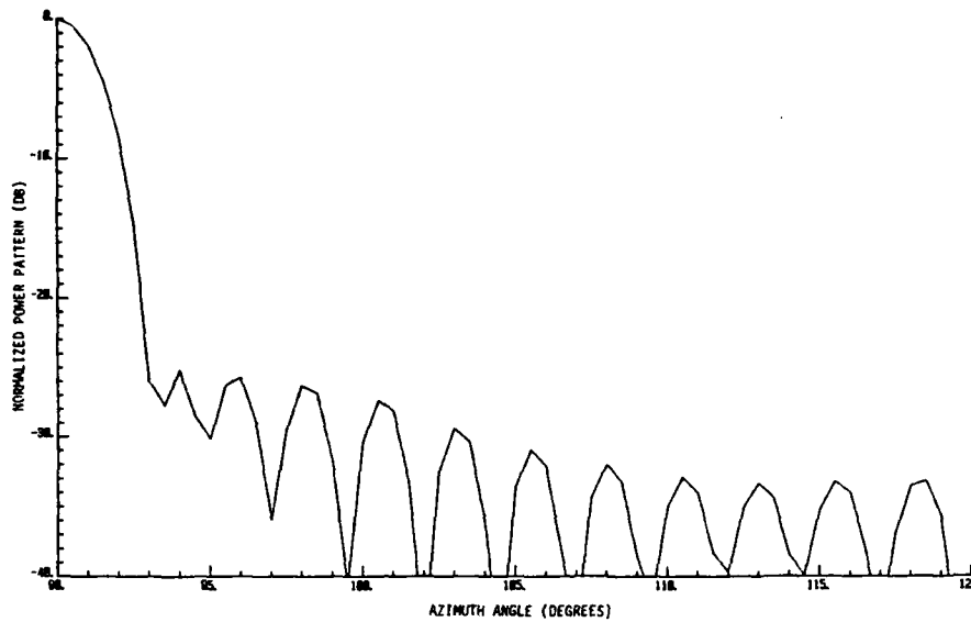
Figure 11. Calculated H-Plane Pattern for Initial Aperture Distribution
