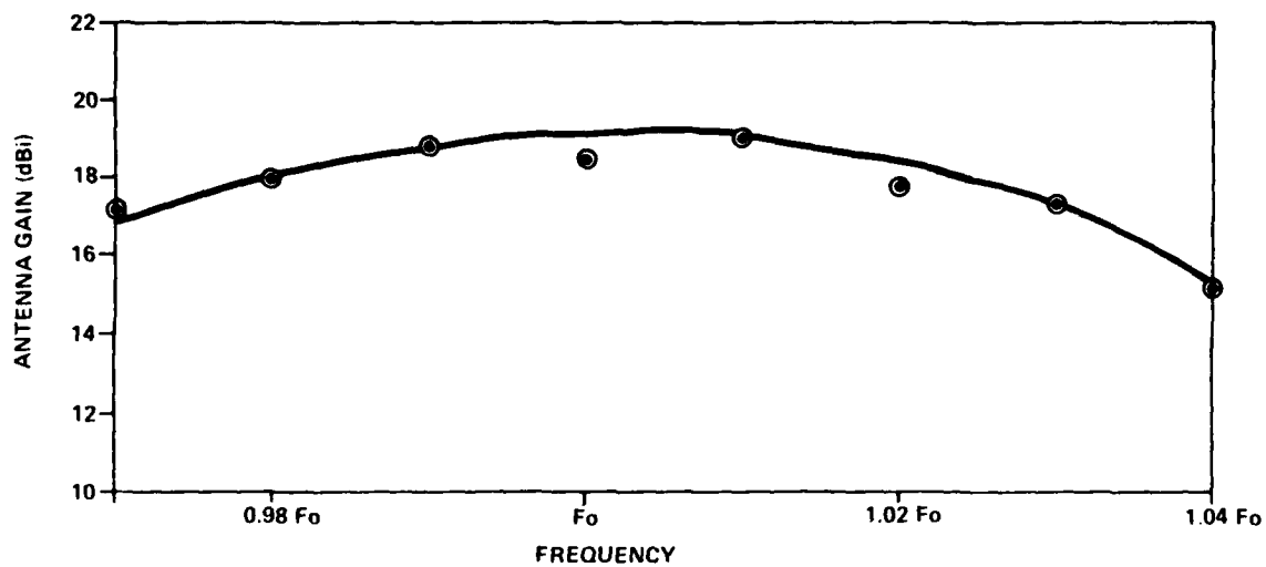
Figure 14. Microstrip Monopulse Dipole Array \Sigma -Channel Peak Gain
