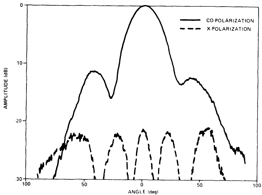
Figure 6. Three Element Dipole Array H-Plane Radiation Pattern
