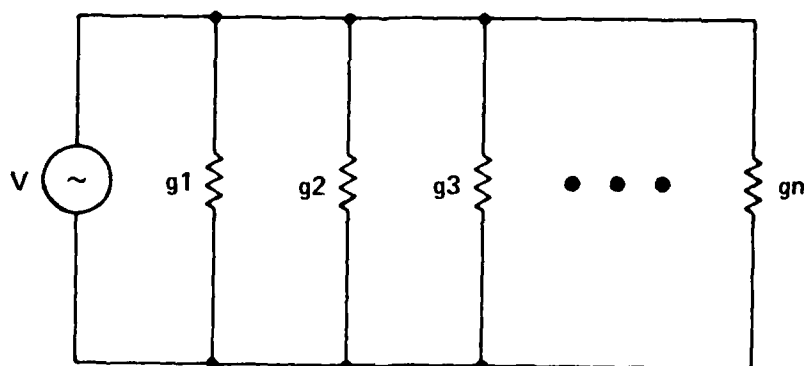
Figure 3. Resonant Circuit Model of Linear EMC Dipole Array
