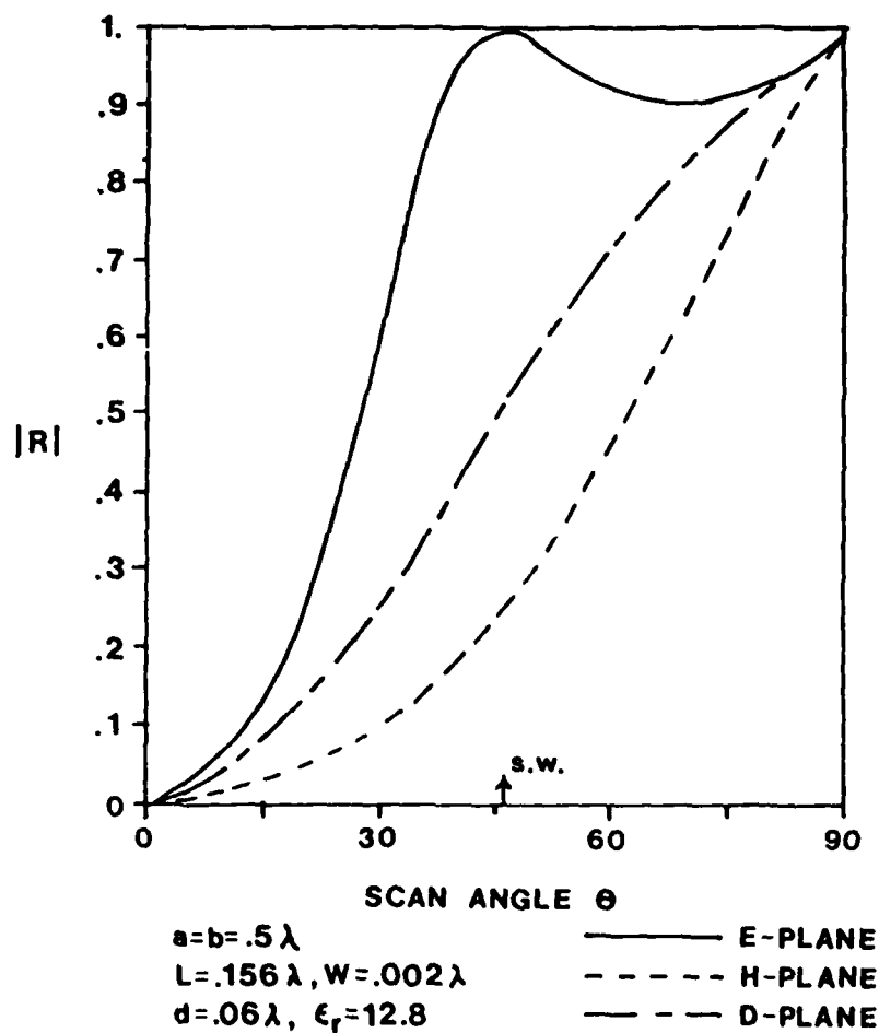
Figure 5. Calculated scan characteristics of infinite array of microstrip dipoles on \epsilon_r=12.8 substrate for scanning in E, H and D planes. Reflection coefficient is calculated with respect to broadside input impedance, Z_p=9.3+j0.3 .
