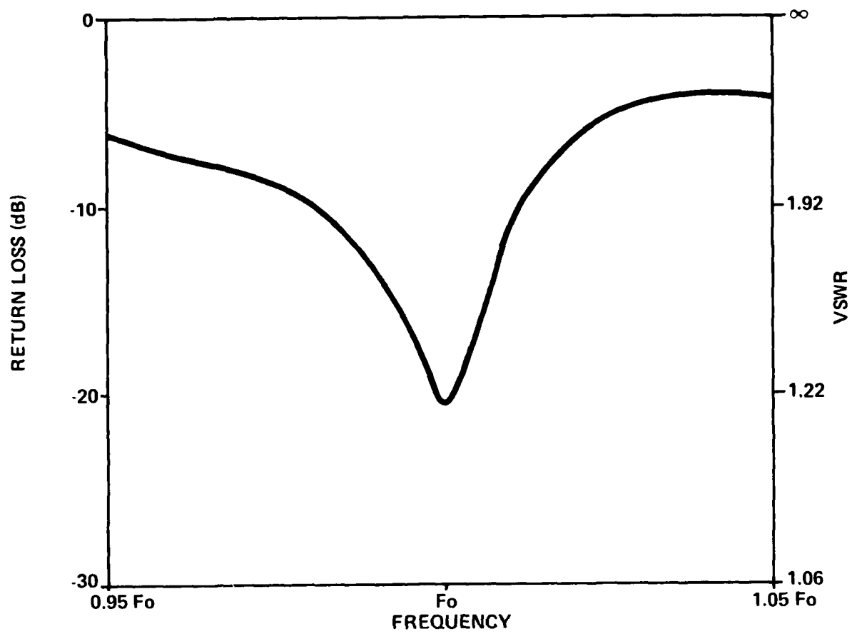
Figure 10. Single Quadrant Input Impedance Match
