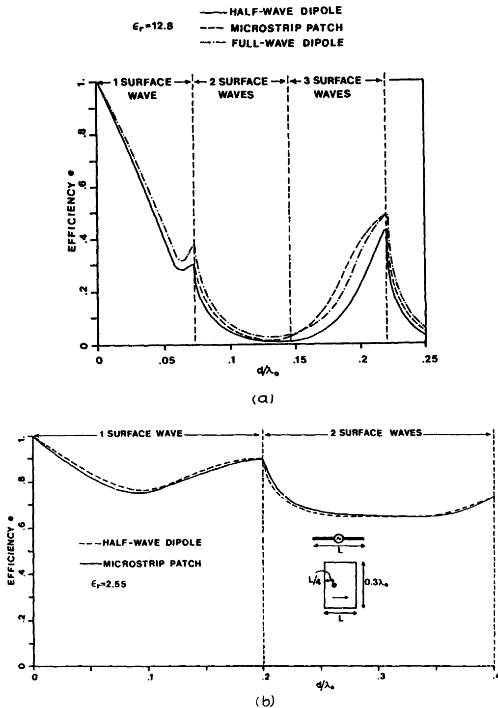
Figure 2. Efficiency due to surface wave excitation by printed dipoles and patches. Patch width is 0.3\lambda_0 . (a) \epsilon_r = 12.8 (b) \epsilon_r = 2.55 .
