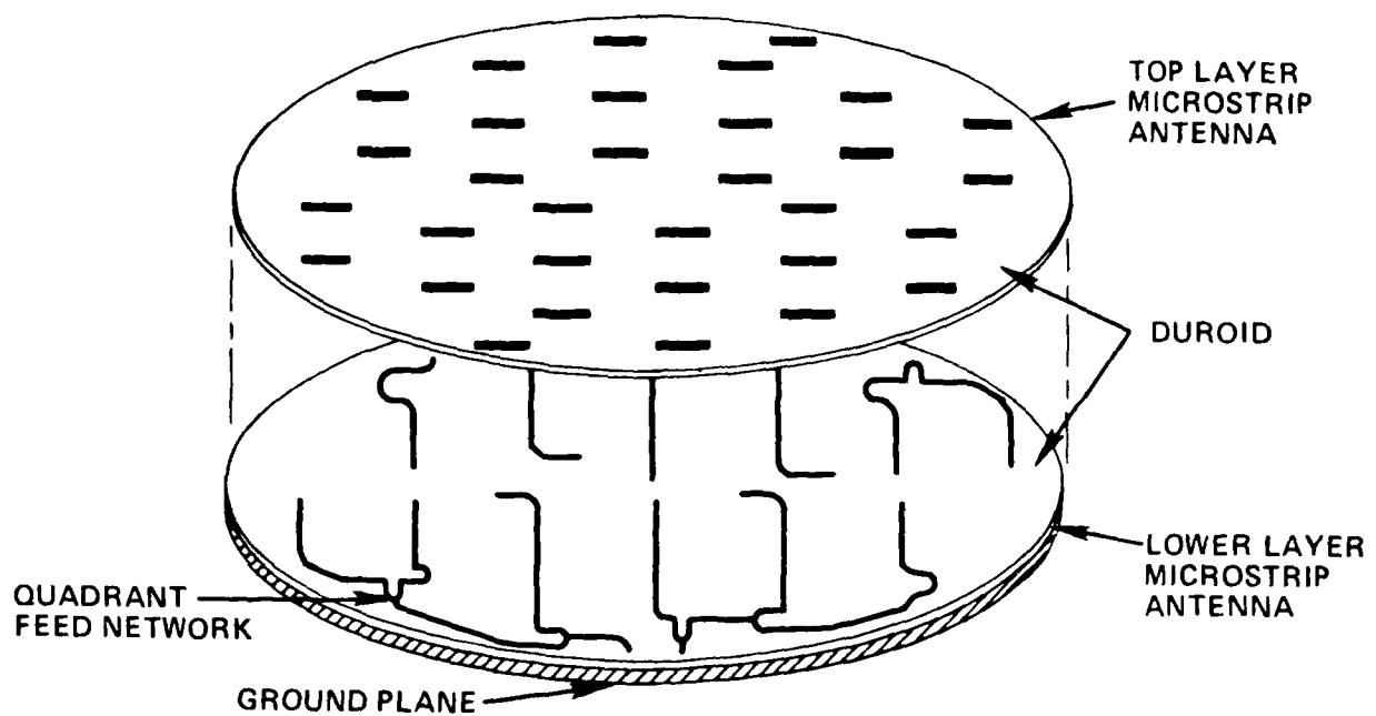
Figure 2. Microstrip Monopulse Array, Exploded View (Quadrants indicated)
