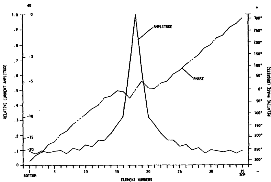
Figure 5. Amplitude and Phase for 35-Element Woodward Distribution
