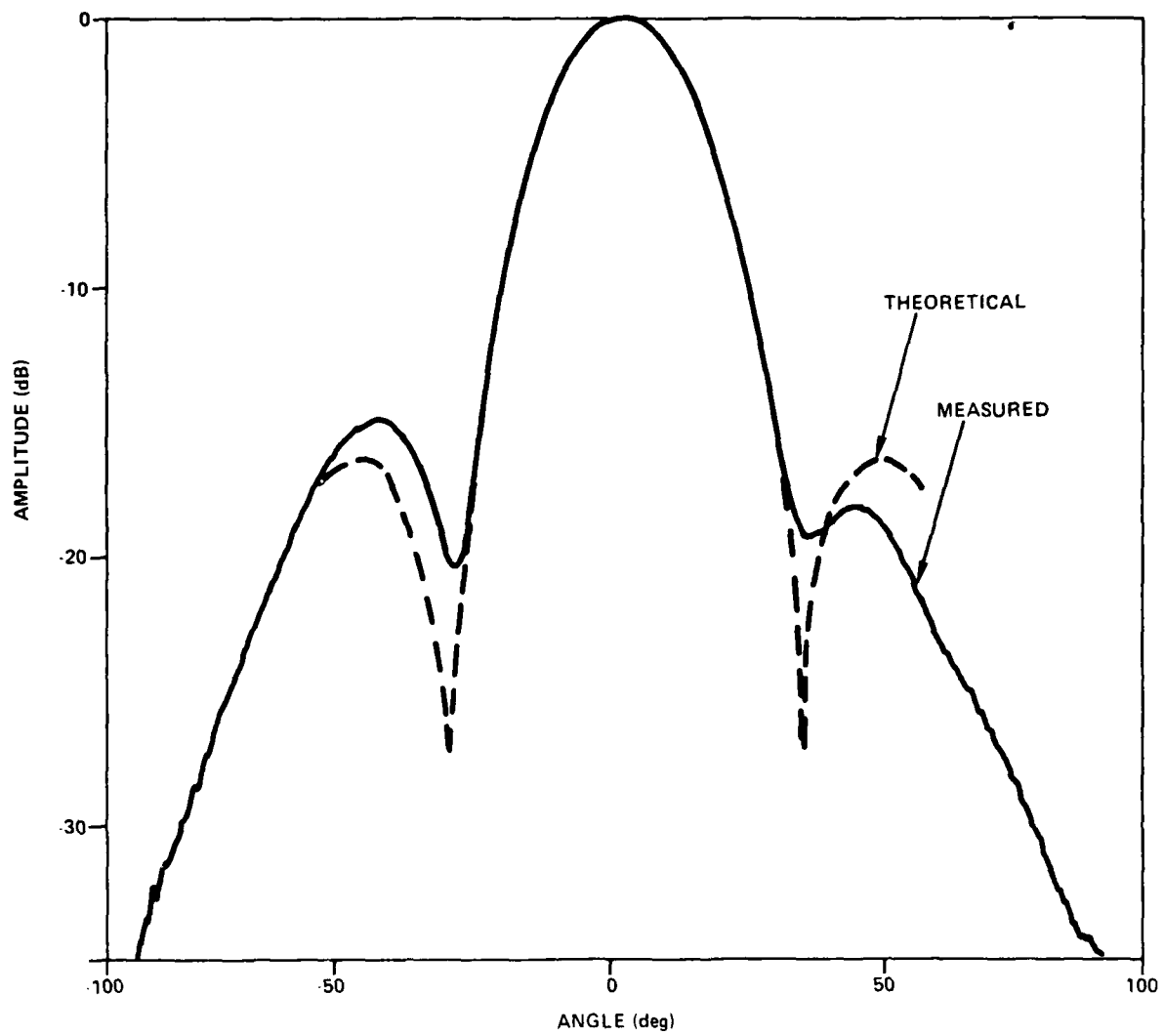
Figure 8. Single Quadrant Principal Plane Pattern (H-Plane Cut)
