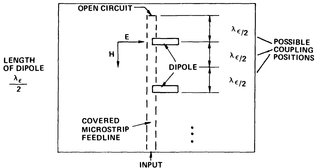
Figure 1b. EMC Linear Array, Top View
