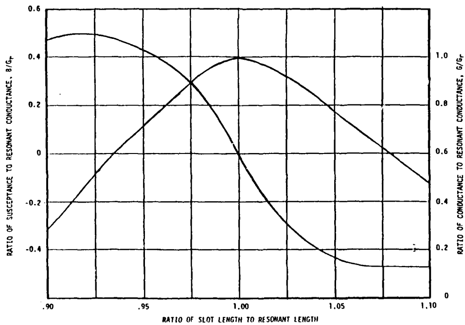
Figure 12. Normalize Self-Admittance Components for Longitudinal Shunt Slot
