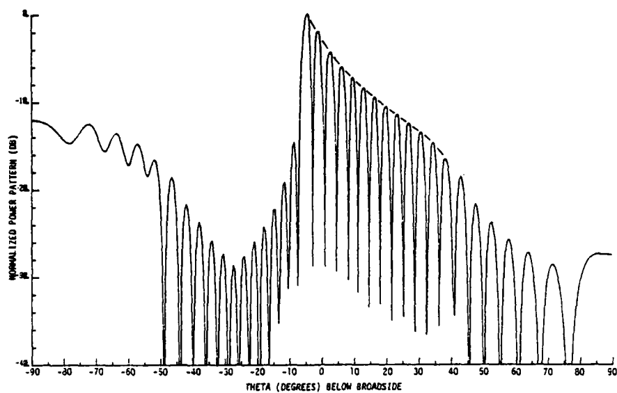
Figure 9a. Starting Pattern for 26-Element Shaped Beam Synthesis
