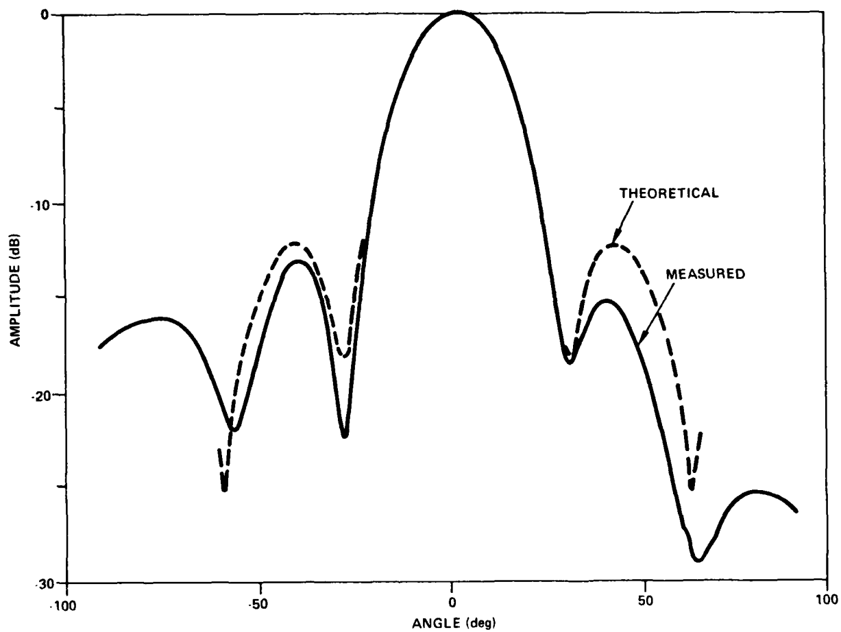
Figure 9. Single Quadrant Principal Plane Pattern (E-Plane Cut)
