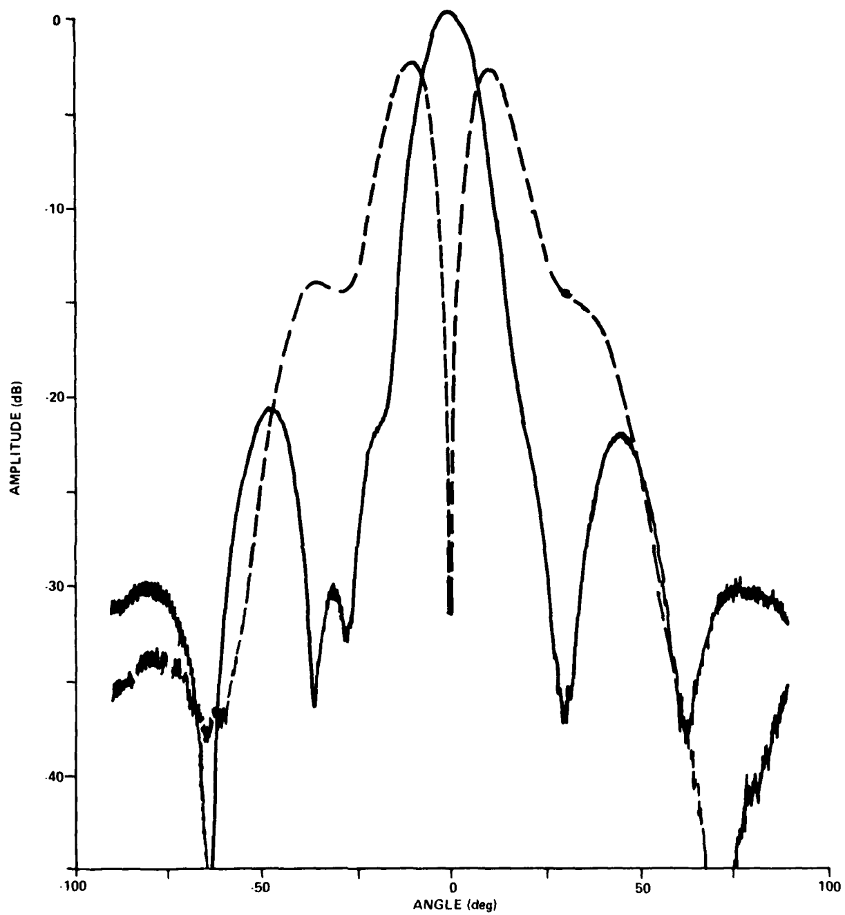
Figure 12. Microstrip Monopulse Dipole Array Principal Plane Radiation Patterns (E-Plane Cut)
