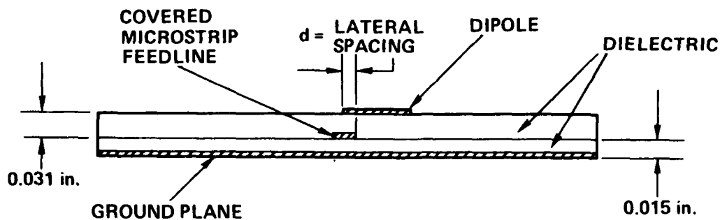
Figure 1a. EMC Linear Array, Cross-Sectional View
