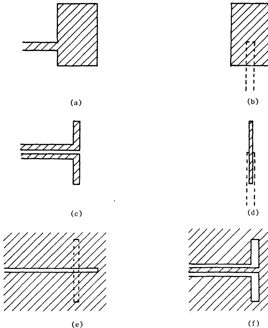
Figure 11. Some possible transmission line and element configurations for integrated structures. (a) Microstripline and patch. (b) Electromagnetically coupled (EMC) microstripline and patch. (c) Printed two-conductor line and dipole. (d) EMC dipole. (e) Slotline and dipole. (f) CPW and slot.
