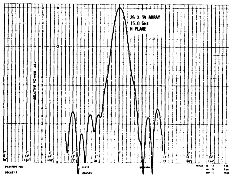
Figure 16. E- and H-Plane Patterns for 26 x 34 Array
