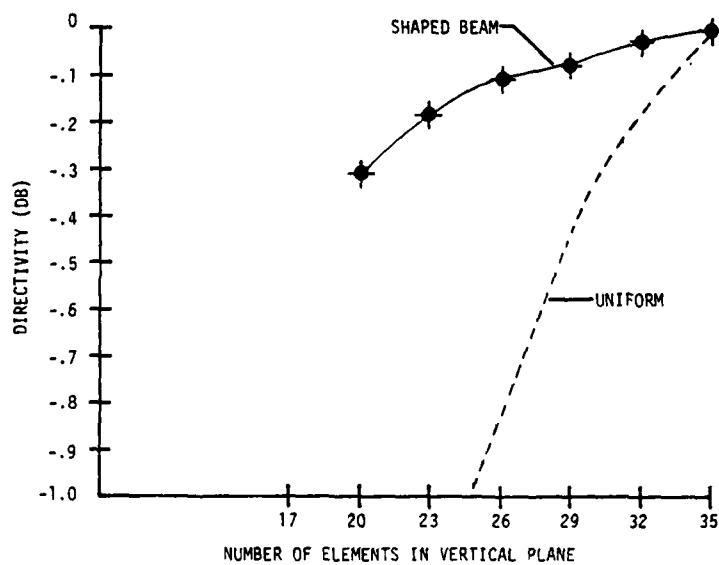
Figure 6. Antenna Directivity vs Number of Elements in the Vertical Plane
