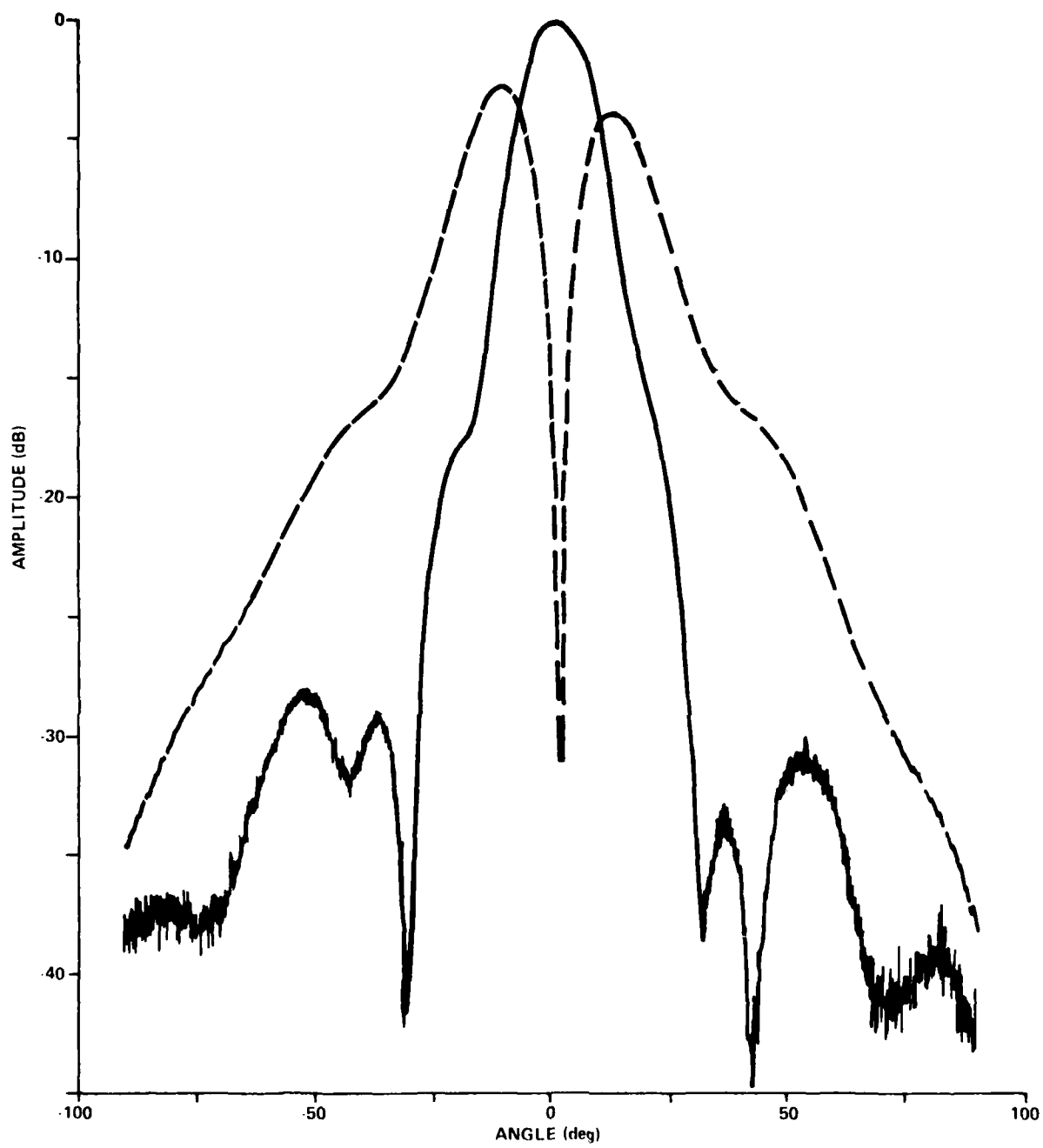
Figure 13. Microstrip Monopulse Dipole Array Principal Plane Radiation Patterns (H-Plane Cut)
