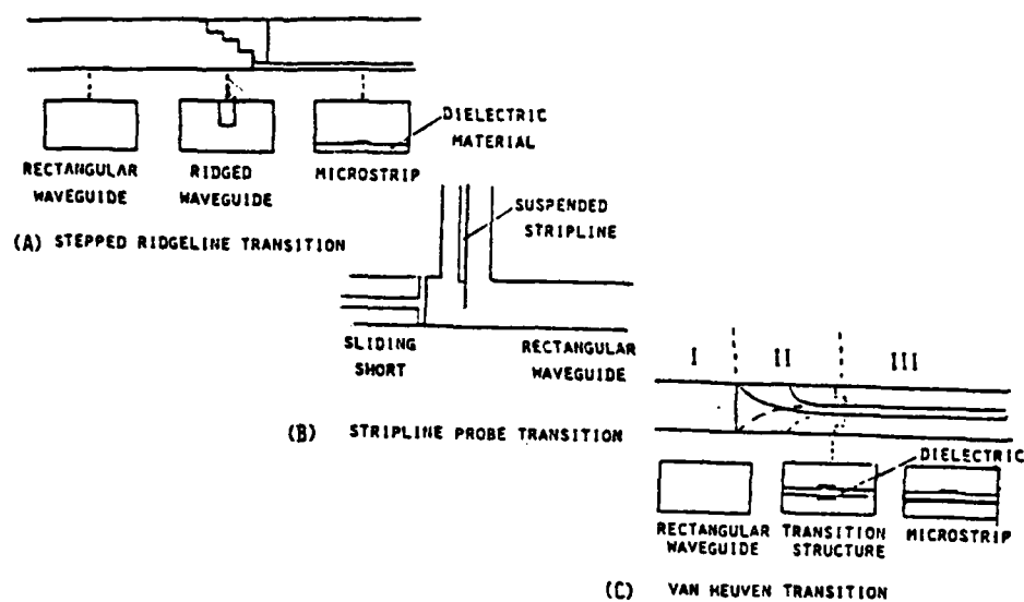
Figure 4. Typical substrate-to-waveguide transitions.
