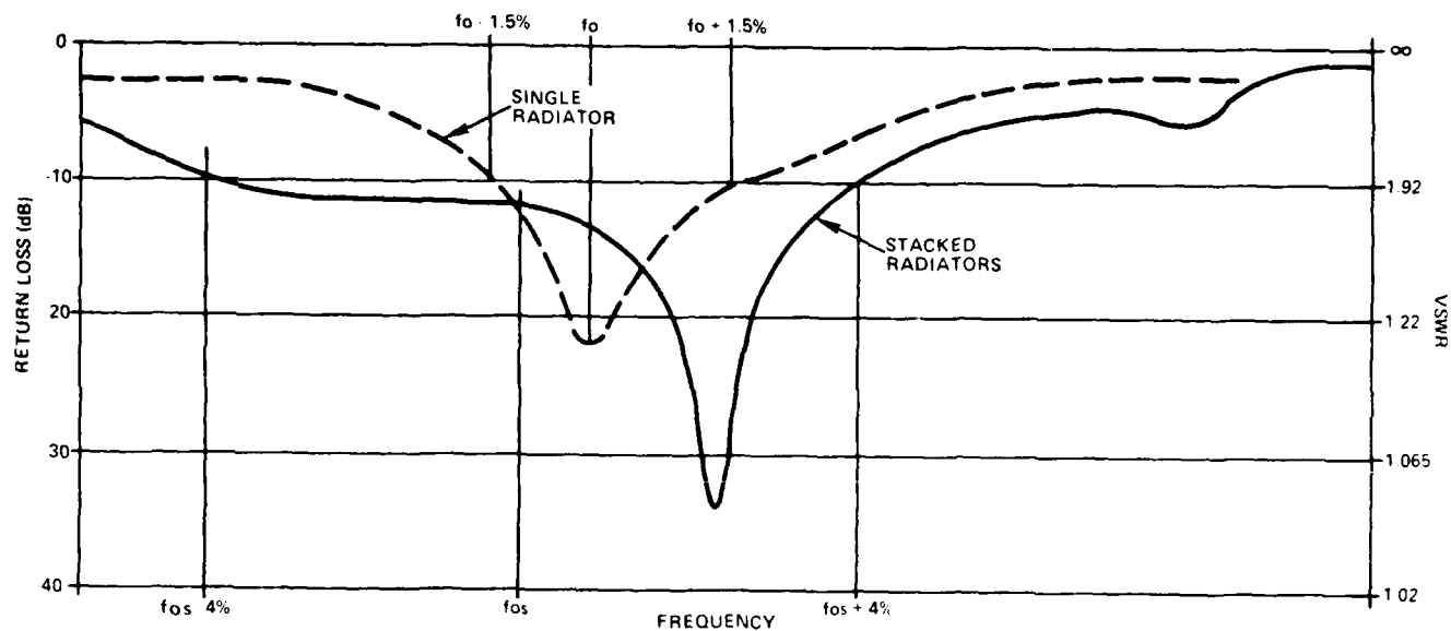
Figure 5. Input Impedance Match of Bonded 3 Element Arrays
