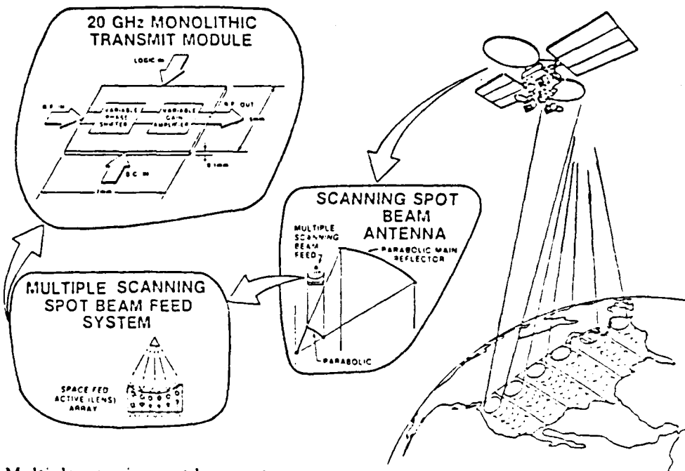
(B) Multiple scanning spot beam antenna.
