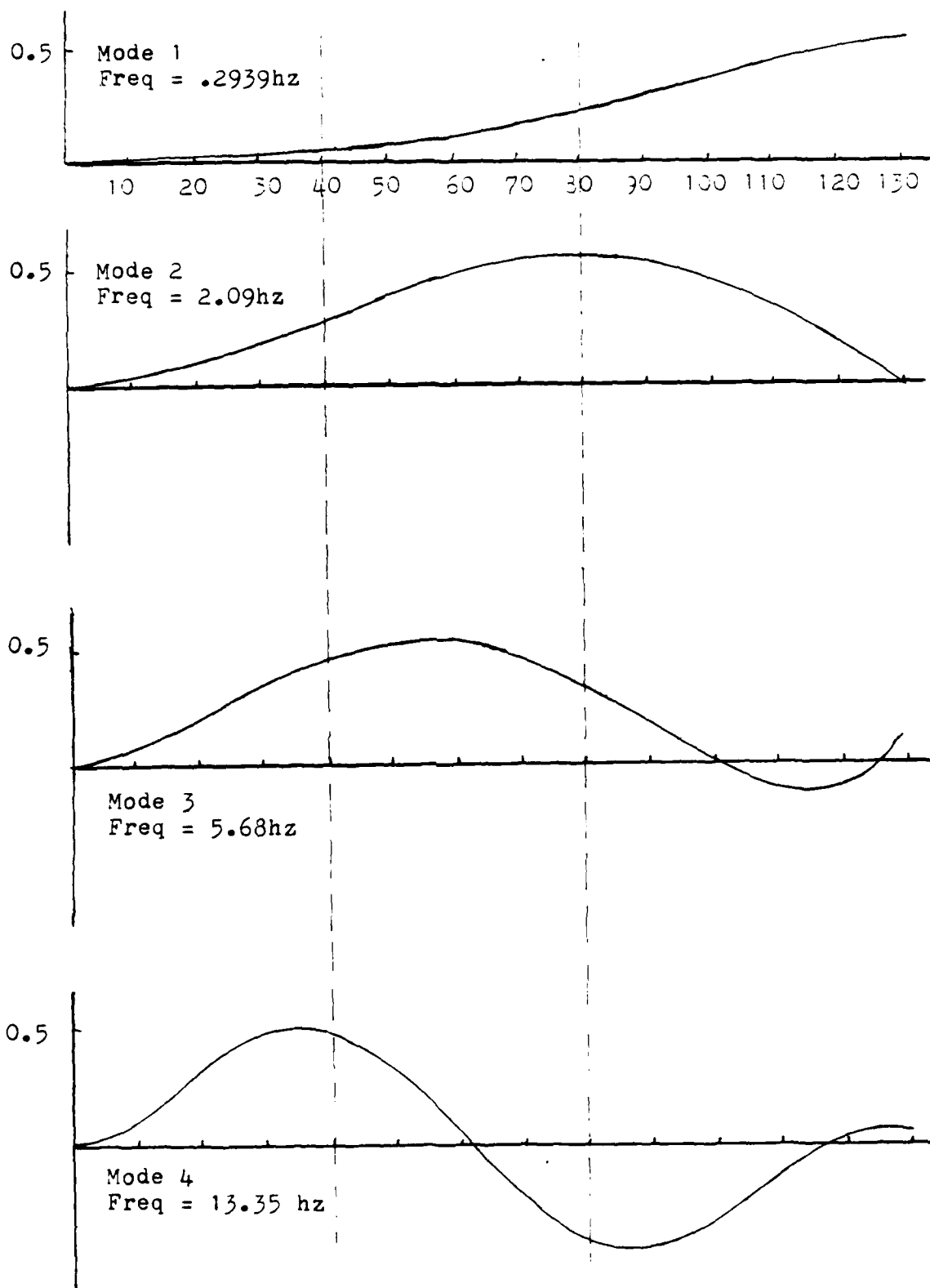
Fig. 6. Roll and Pitch Mode Shapes
