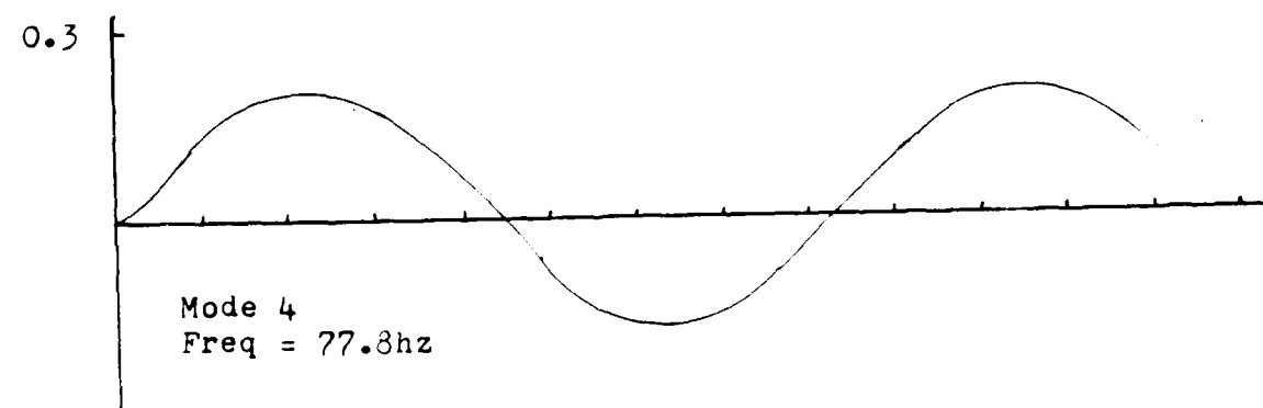
Fig. 8. Yaw Mode Shapes
