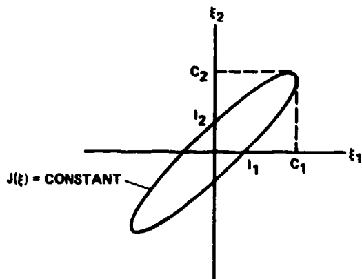
Figure (11.2-5). Cramer-Rao bounds and insensitivities.
