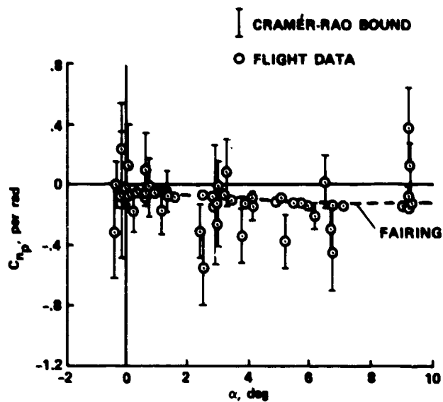
Figure (11.3-1). Estimates of C_{np} .
