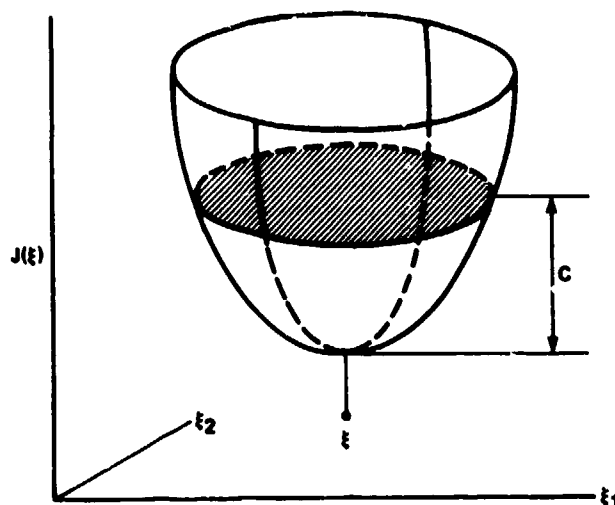
Figure (11.1-3). Construction of two-dimensional confidence ellipsoid.
