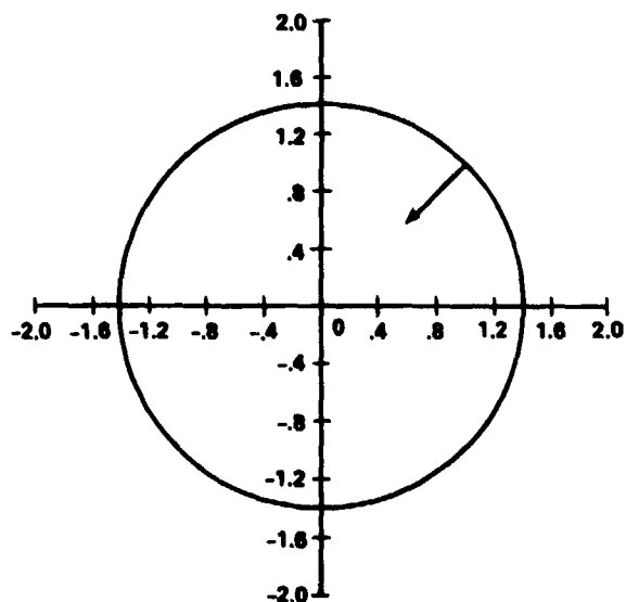
Figure (2.3-1). The gradient direction from a circular isocline.
