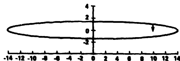
Figure (2.3-2). The gradient direction near a narrow valley.
