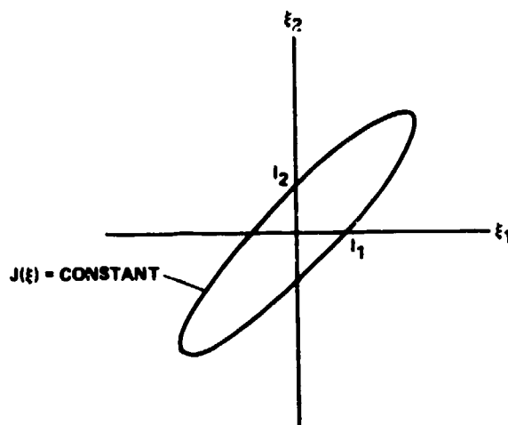
Figure (11.2-1). Geometric interpretation of insensitivity.
