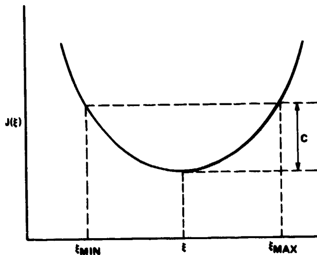
Figure (11.1-2). Construction of one-dimensional confidence ellipsoid.
