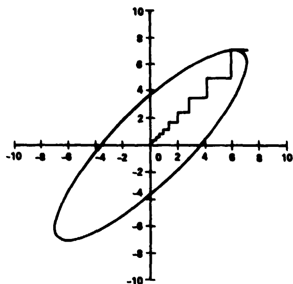
Figure (2.2-1). Behavior of axial iteration.
