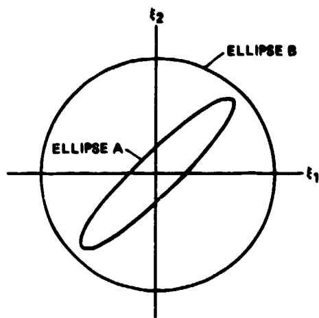
Figure (11.2-2). Correlation and sensitivity.
