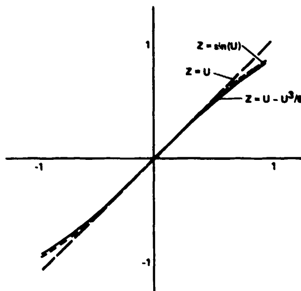
Figure (11.4-4). Z = \sin(U) in the range |U| < 1.0 .
