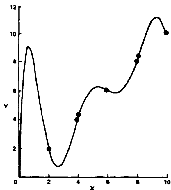
Figure (11.4-2). Exact polynomial match of noise data.
