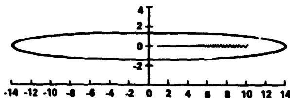
Figure (2.3-4). Worse behavior of the gradient algorithm.
