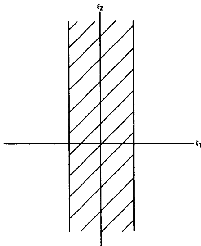
Figure (5.3-1). Confidence region with singular P^{-1} .
