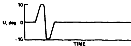
Figure (11.2-4). Low correlation and low sensitivity.
