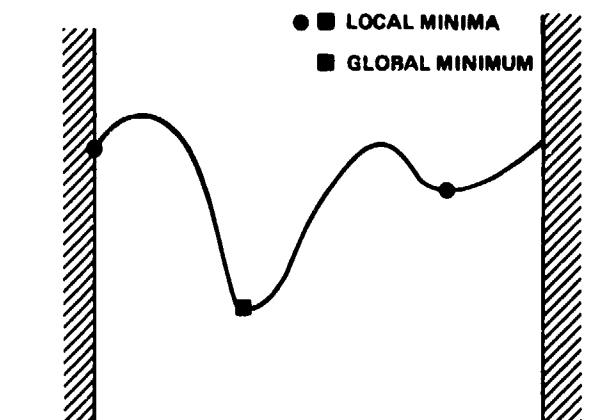
Figure (2.0-1). Illustration of local and global minima.
