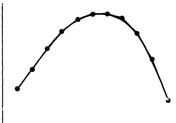
Figure (7.5-3). Linear interpolation input model.
