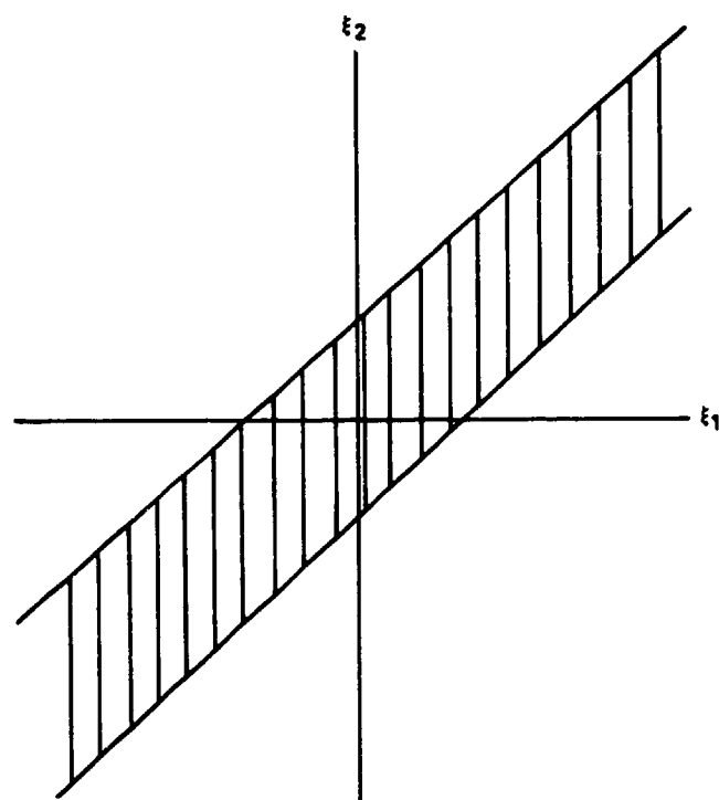
Figure (5.3-2). Confidence region with another singular P^{-1} .
