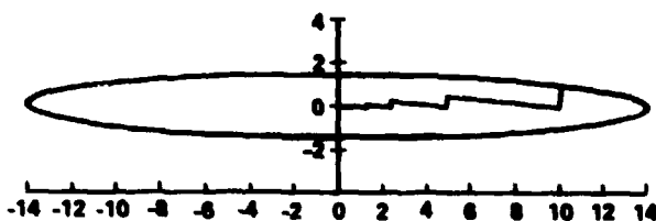
Figure (2.3-3). Behavior of the gradient algorithm in a narrow valley.
