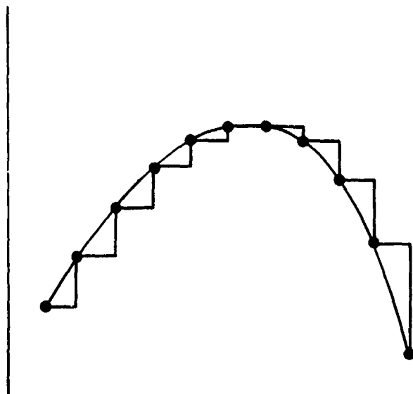
Figure (7.5-1). Hold-last-value input model.
