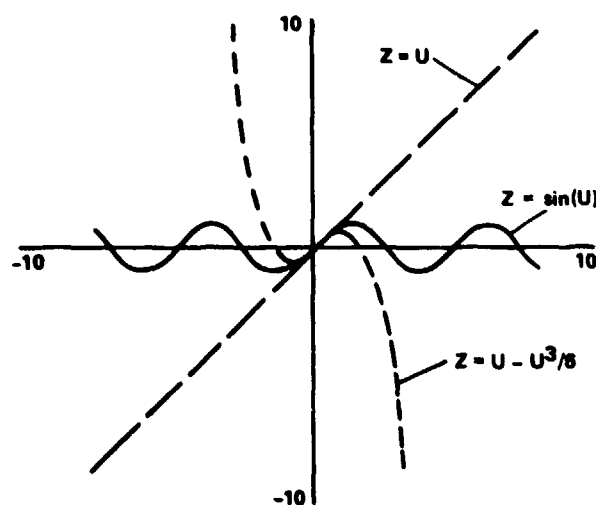
Figure (11.4-5). Z = \sin(U) in the range |U| < 10.0 .
