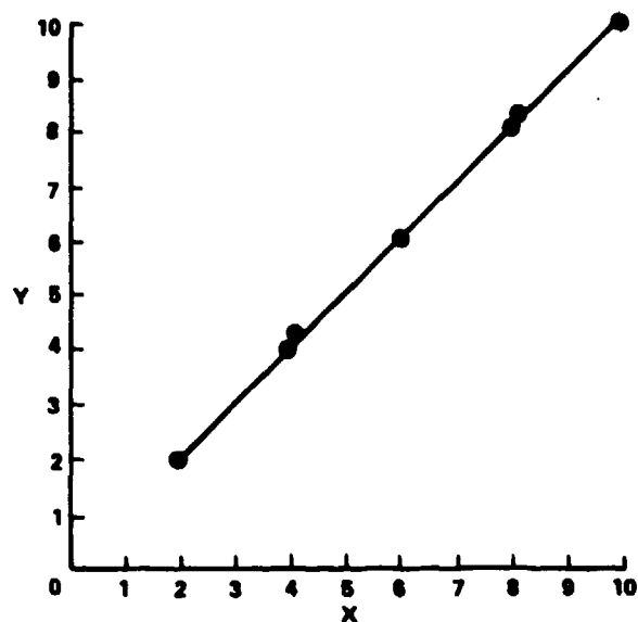
Figure (11.4-1). Best linear fit of noise data.
