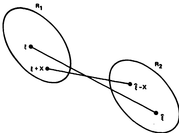
Figure (11.1-1). Construction of R_2 .
