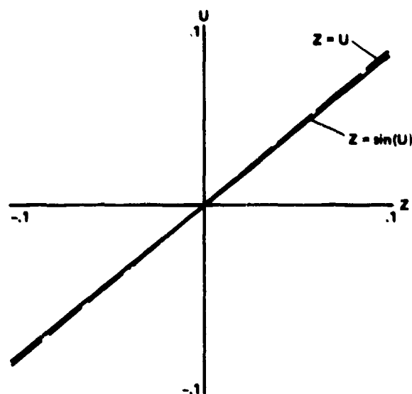
Figure (11.4-3). Z = \sin(U) in the range |U| < 0.1 .
