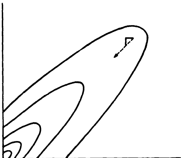
Figure (2.2-2). The pattern direction.
