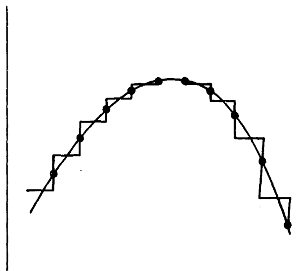
Figure (7.5-2). Average value input model.
