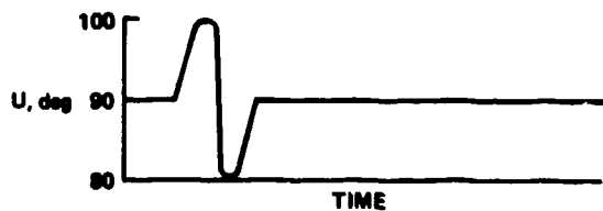
Figure (11.2-3). High correlation and high sensitivity.
