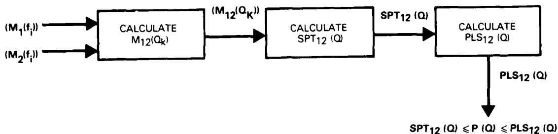
FIGURE II-5. OVERVIEW OF DEMPSTER-SHAFER UPDATING
