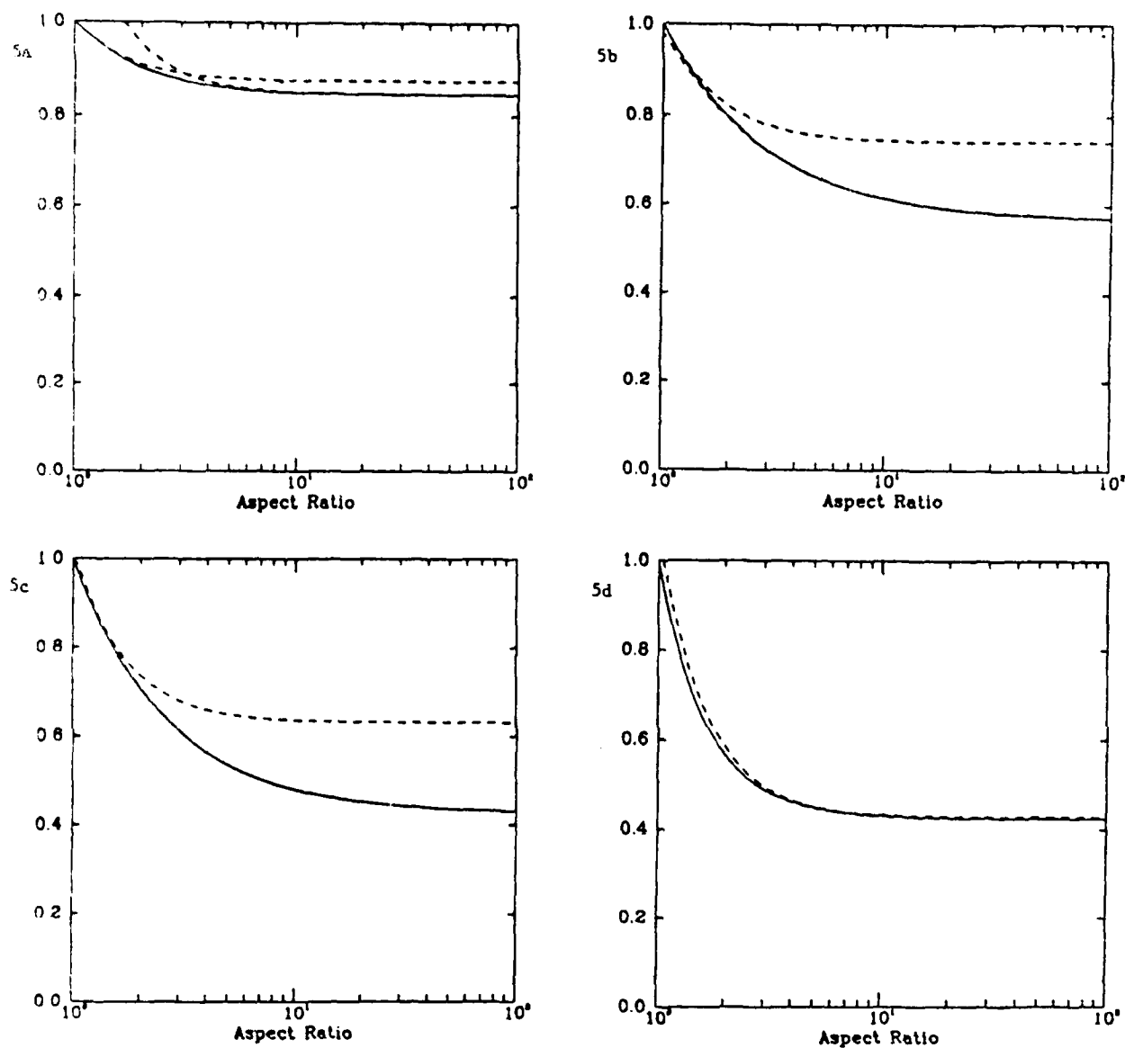
Figure 5. The resistance functions for prolate spheroids, scaled by the results for spheres. The dashed curves are the asymptotic forms of Table 3.
