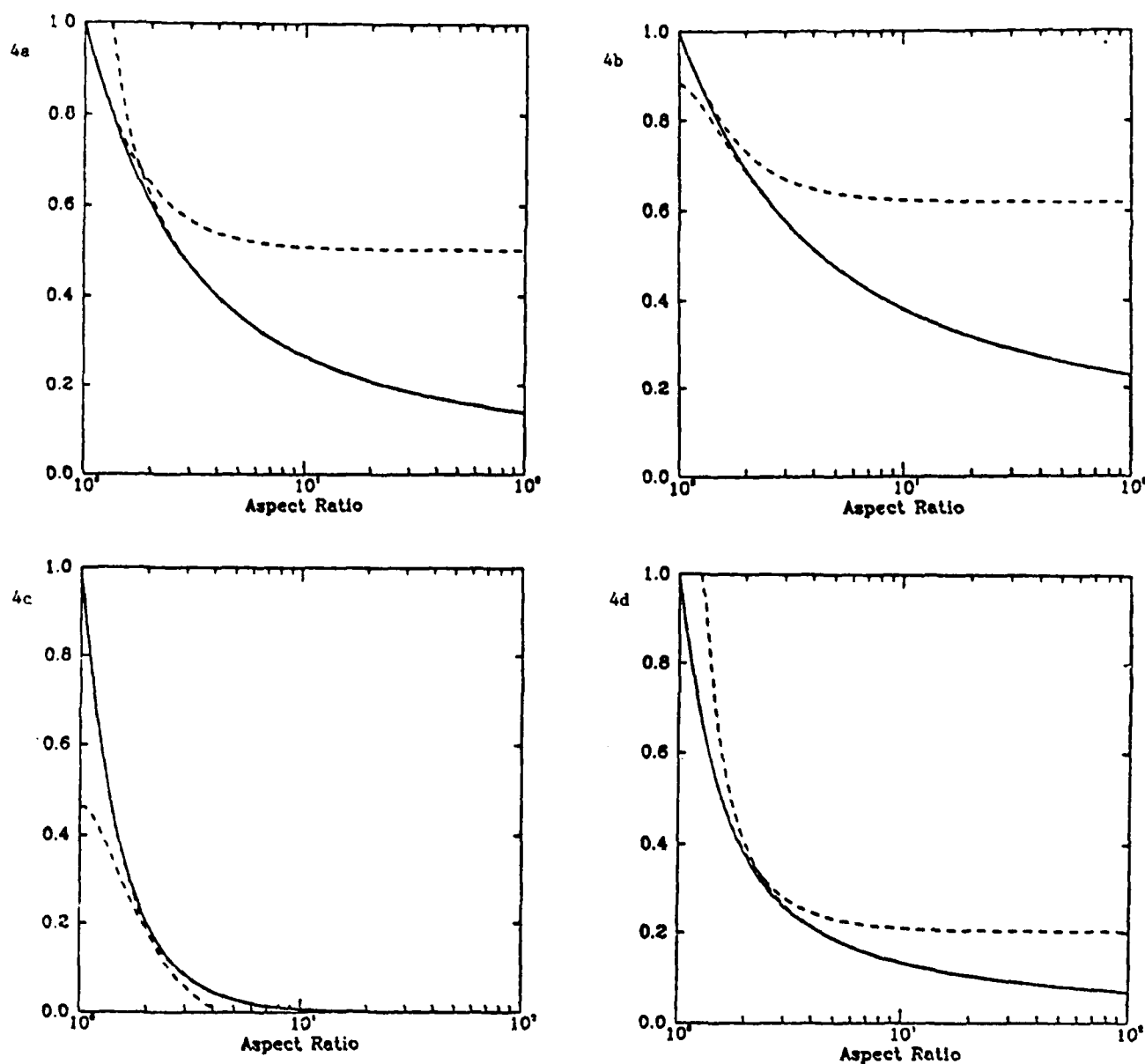
Figure 4. The resistance functions for oblate spheroids, scaled by the results for spheres. The dashed curves are the asymptotic forms of Table 3.
